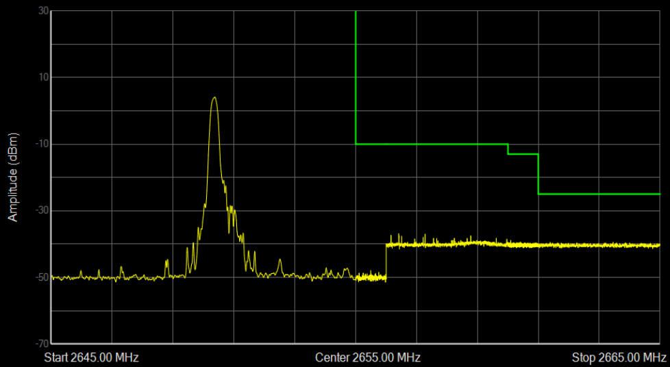
Band41(2555-2655) QPSK BW=5MHz Channel=41215 RB Size=1 Position=#0
