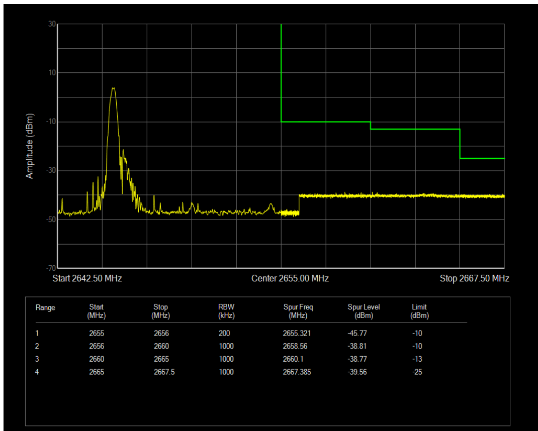
Band41(2555-2655) QAM16 BW=10MHz Channel=41190 RB Size=1 Position=#Max
