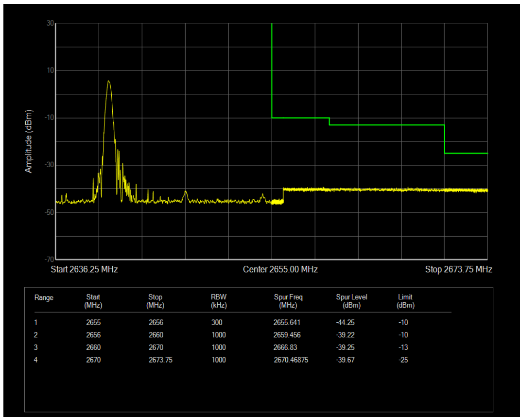
Band41(2555-2655) QAM16 BW=15MHz Channel=41165 RB Size=1 Position=#Max
