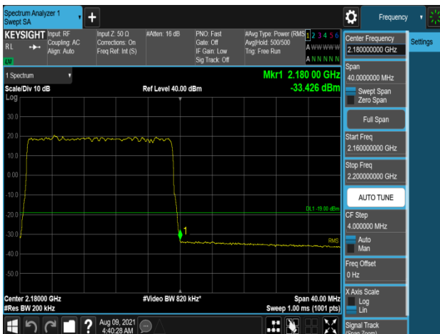
Plot 7-953. Band Edge Emission (2180MHz to 2181MHz) Plot (B66_5M+15M+20M_3C_16QAM - High Channel, Port 3)
