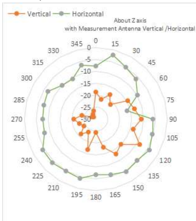
Figure 10: X-Y plane antenna pattern
