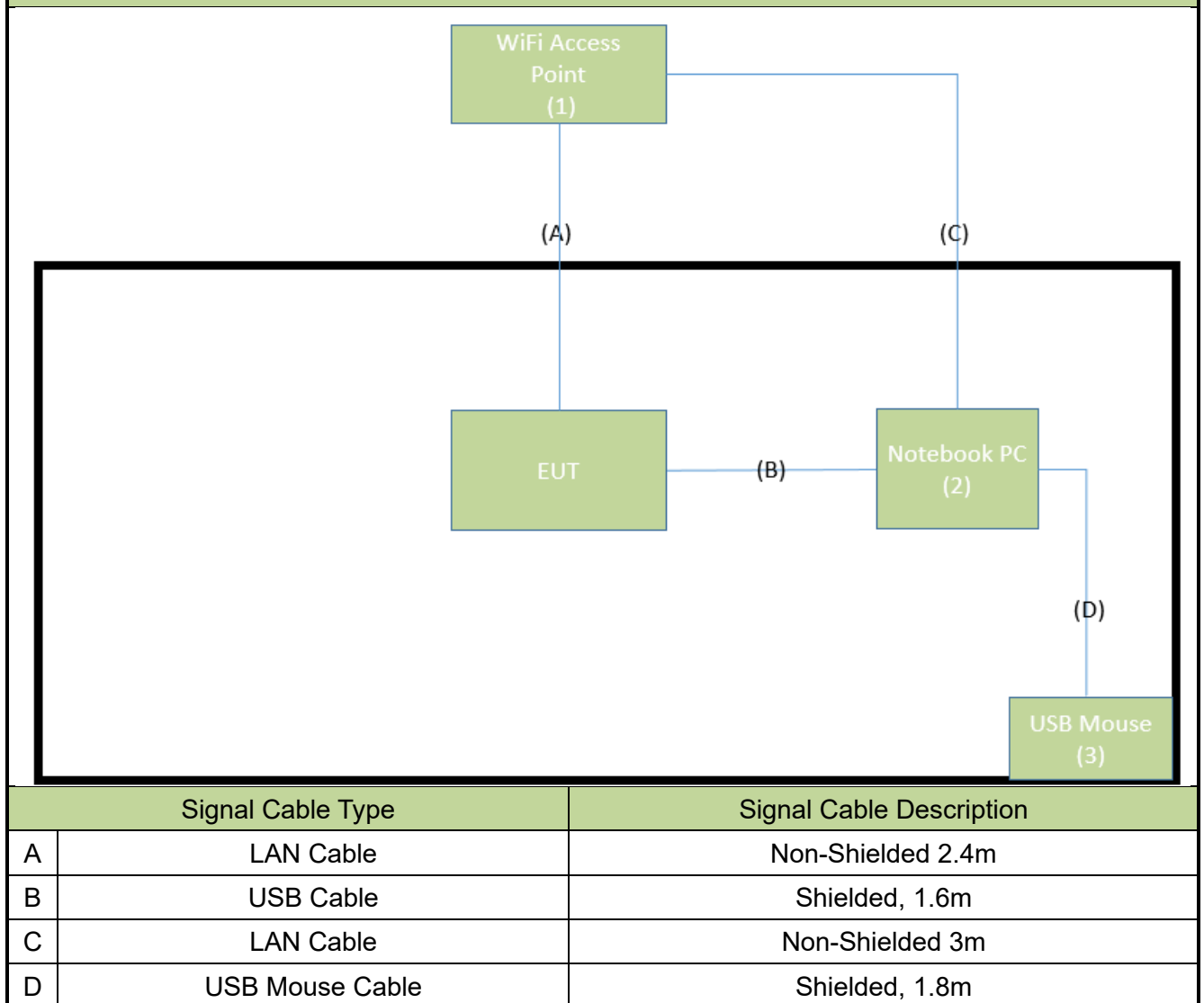
Connection Diagram (Adapter Mode)
