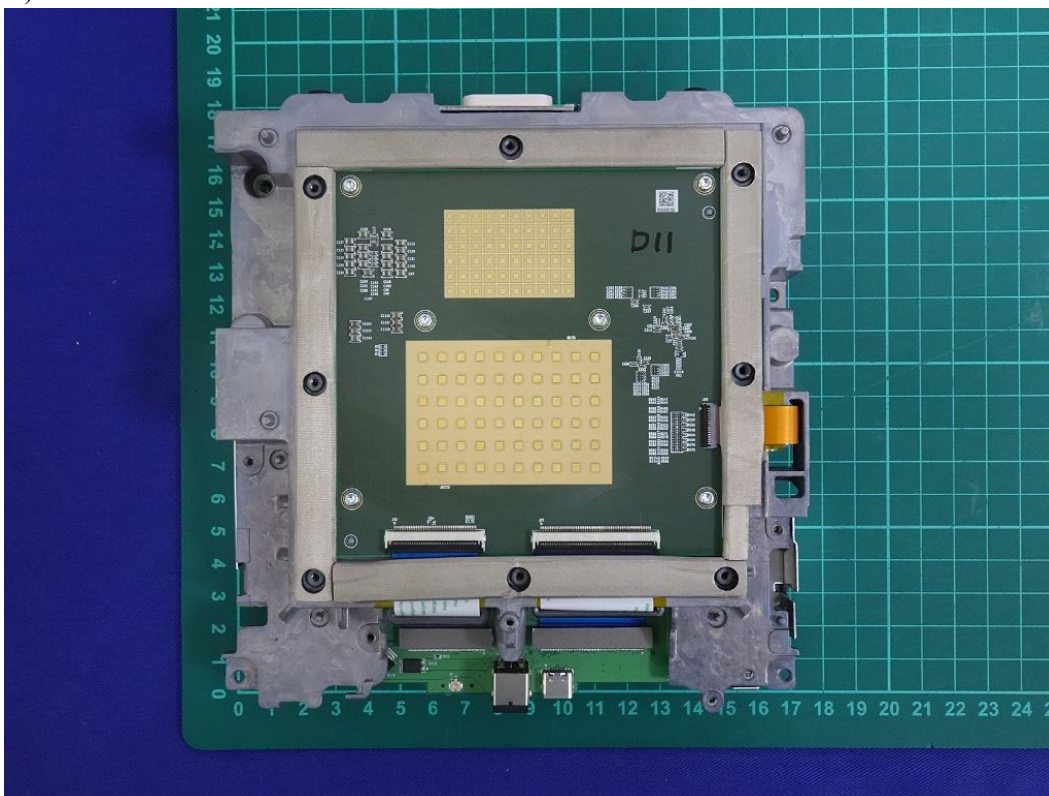
(23) EUT Photo
