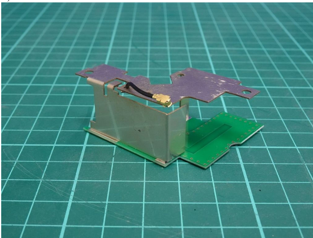
(22) EUT Photo
