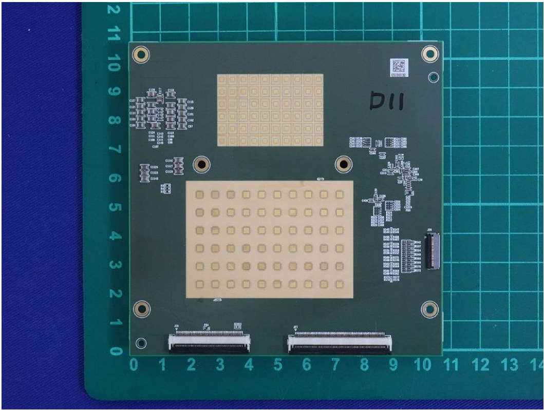
(25) EUT Photo
