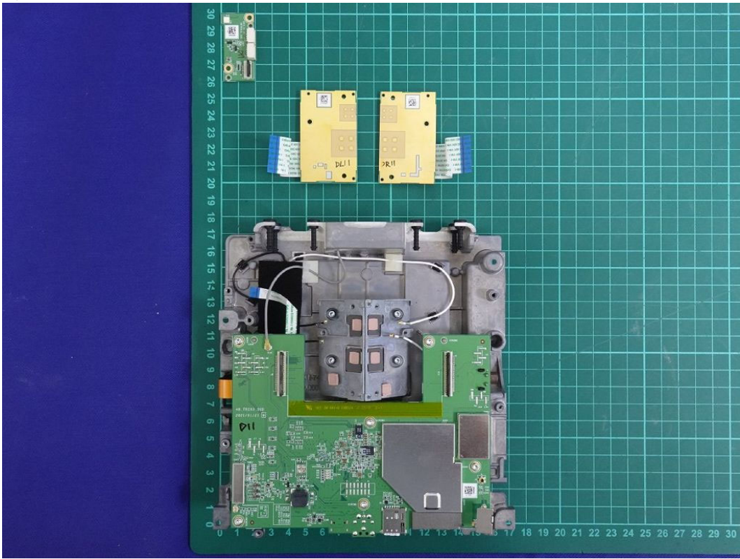
(43) EUT Photo
