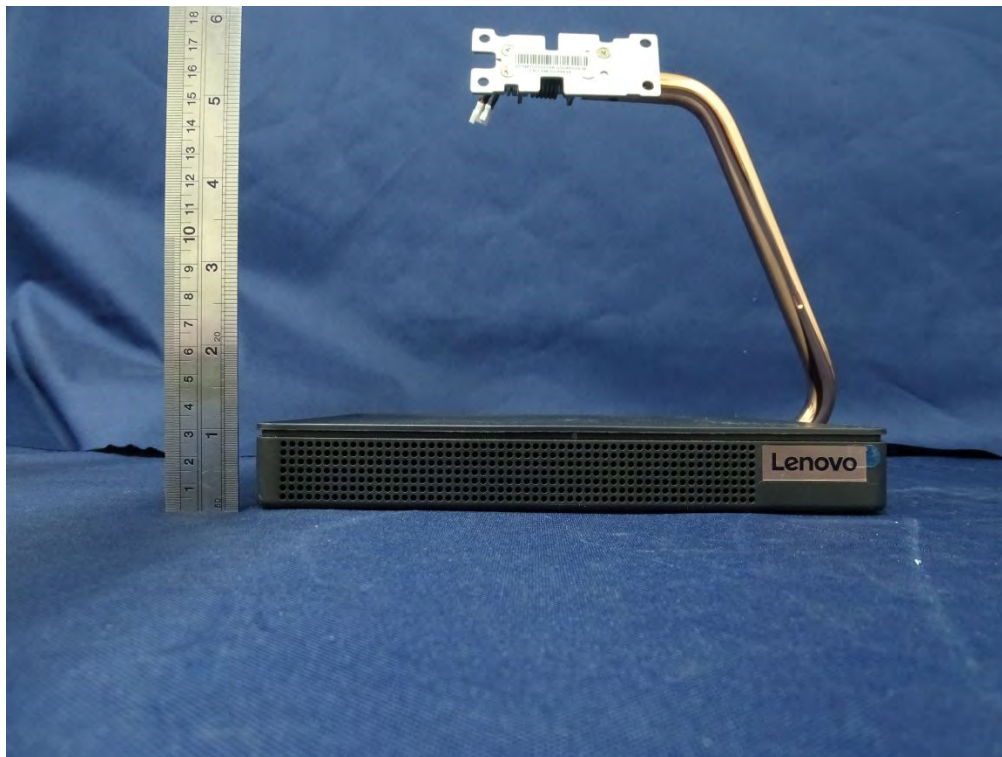
(28) EUT Photo
