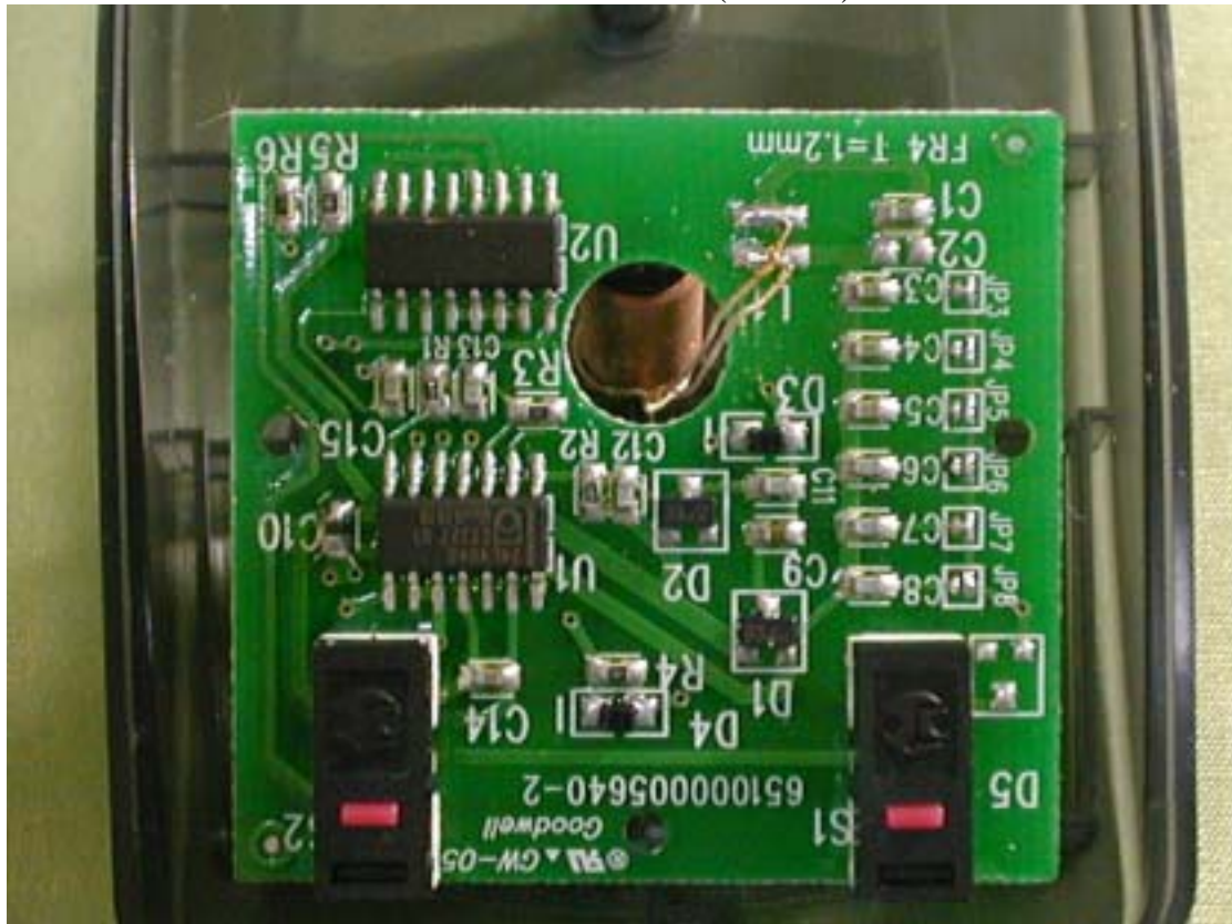
Internal Photo of EUT ( Mouse )
