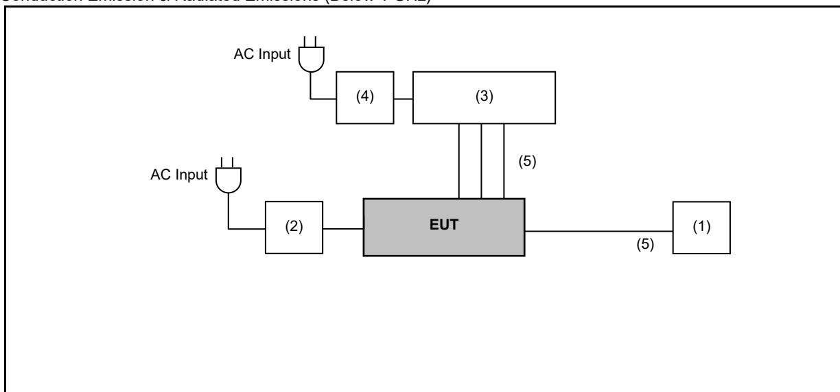
Conduction Emission & Radiated Emissions (Below 1 GHz)
