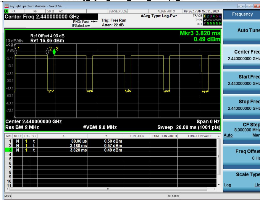
Duty_Cycle_NVNT_ANT1_500kbps_2440
