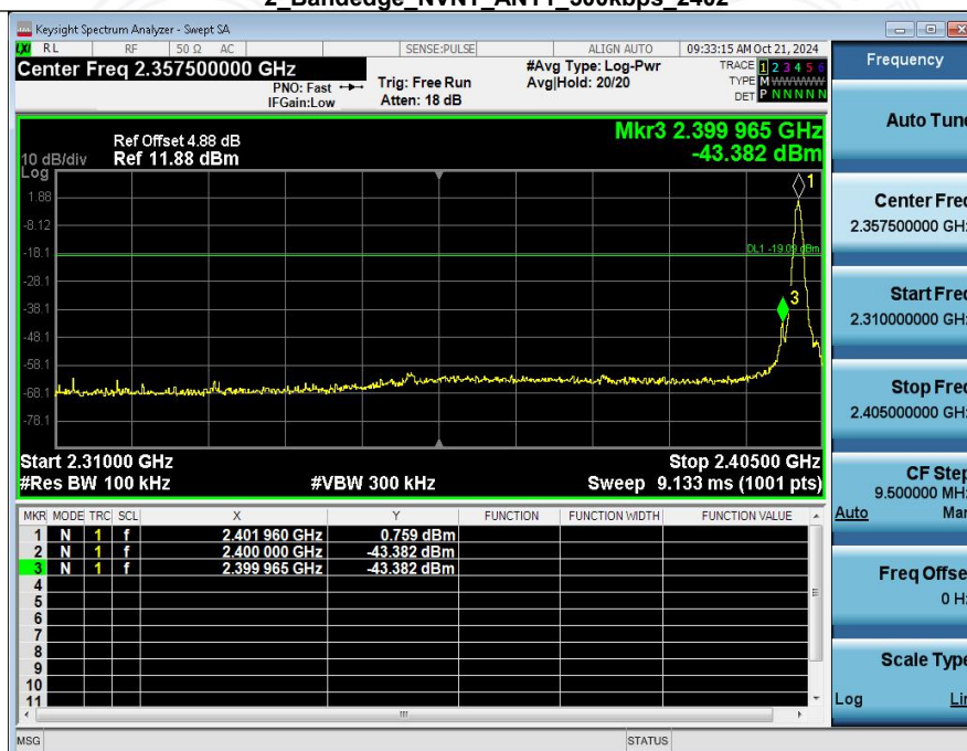
2_Bandedge_NVNT_ANT1_500kbps_2402
