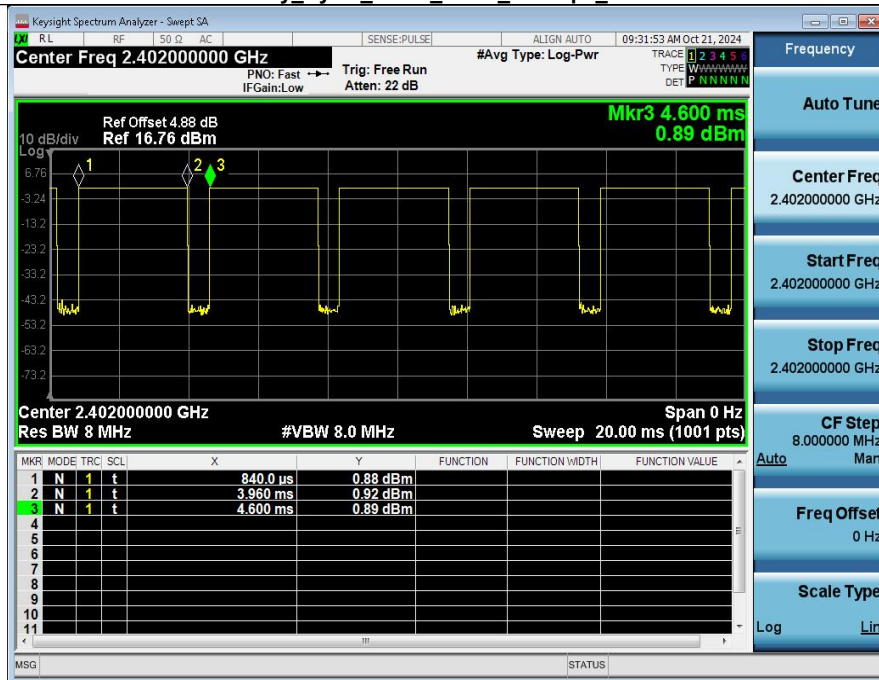
Duty_Cycle_NVNT_ANT1_500kbps_2402
