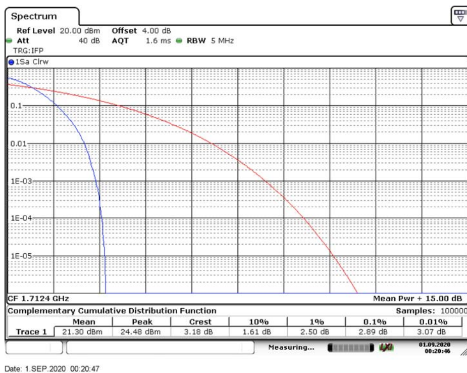
WCDMA_Band 4_RMC_1712.4MHz
