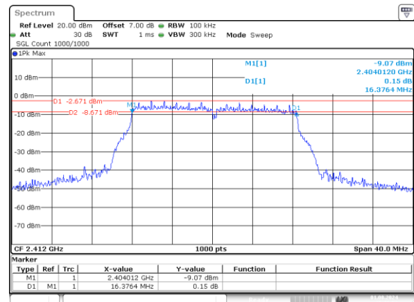
g_2412MHz_Chain 0 16.376MHz
