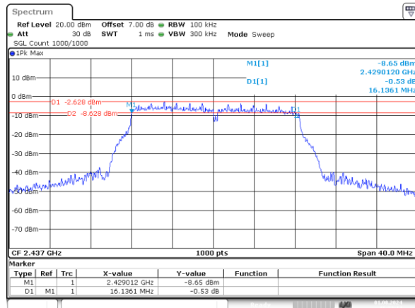
g_2437MHz_Chain 0 16.136MHz
