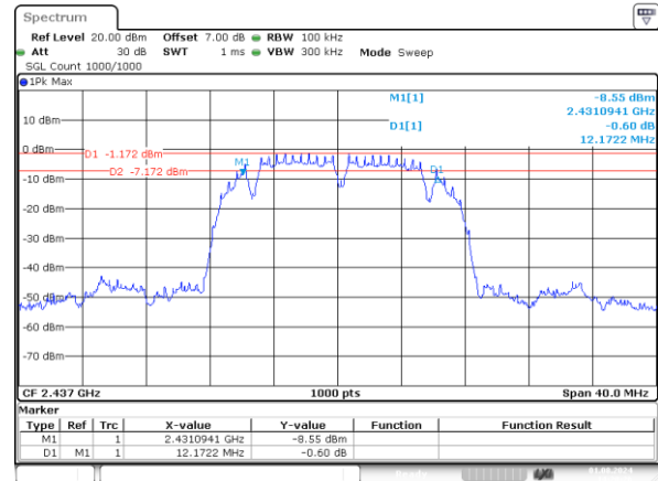
b_2437MHz_Chain 0 12.172MHz
