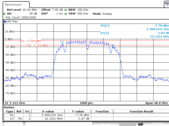
b_2412MHz_Chain 0 12.132MHz
