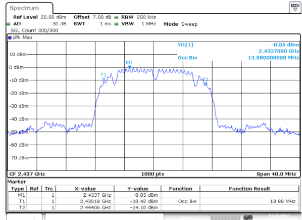
b_2437MHz_Chain 0 13.880MHz
