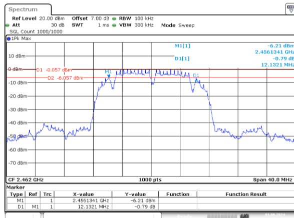
b_2462MHz_Chain 0 12.132MHz
