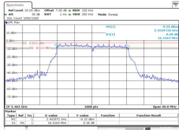
g_2462MHz_Chain 0 16.416MHz
