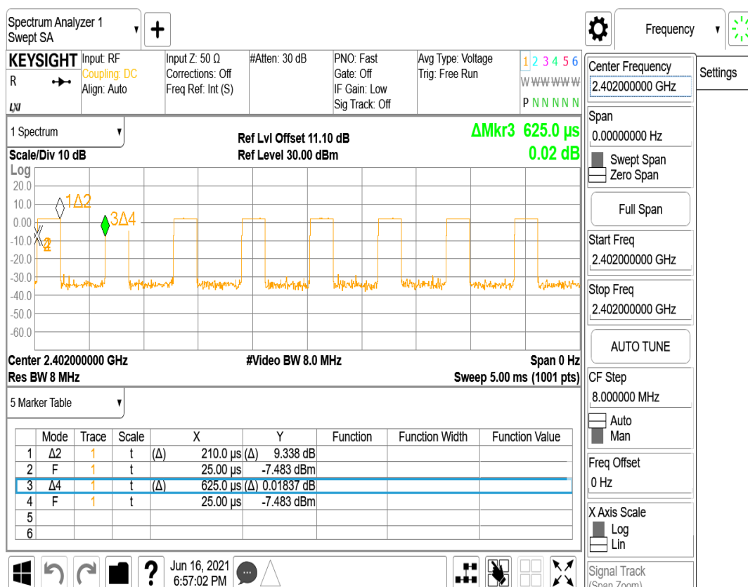
BLE_2M_LowCH00-2402
