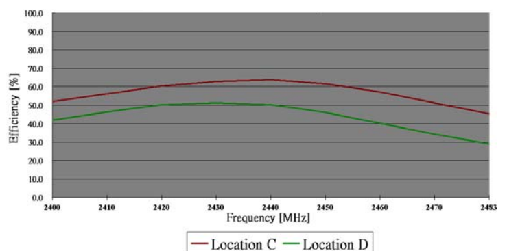
Radiation Efficiency
