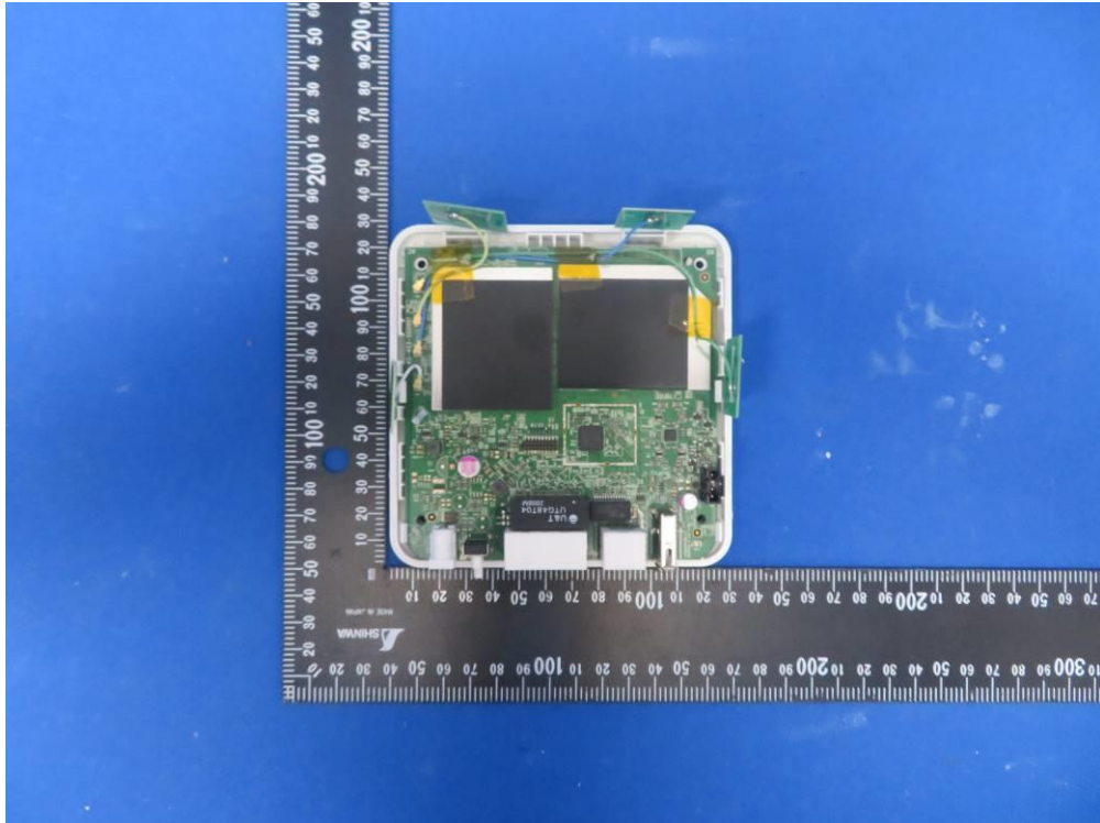
(15) EUT Photo (Model No.: GigaSpire BLAST u4)
