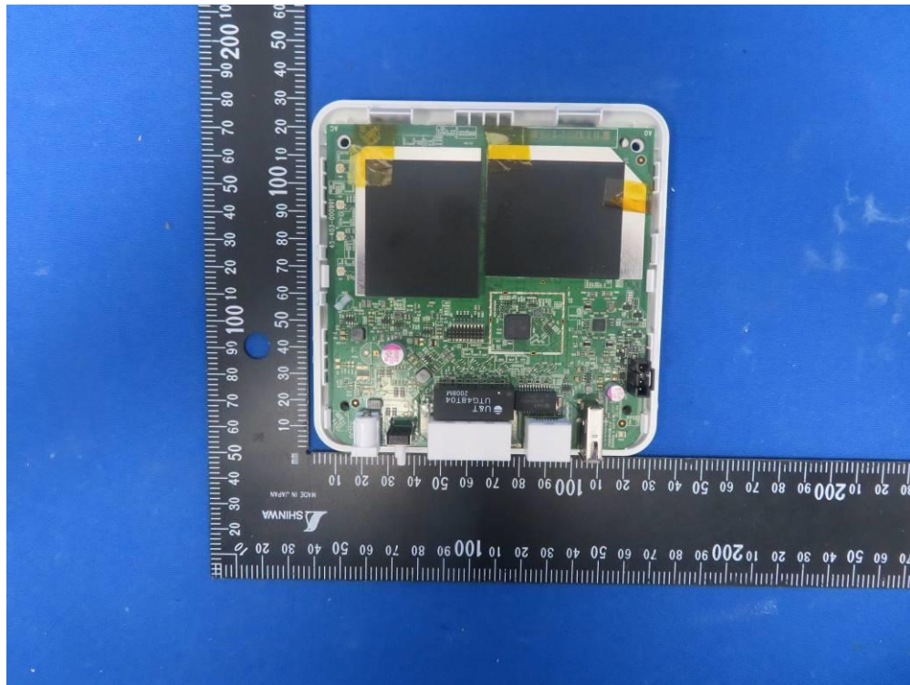
(17) EUT Photo (Model No.: GigaSpire BLAST u4)
