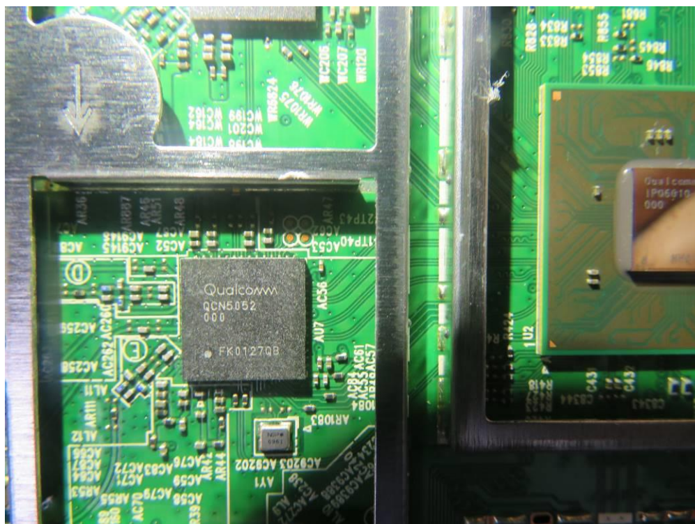
(24) EUT Photo (Model No.: GigaSpire BLAST u4)
