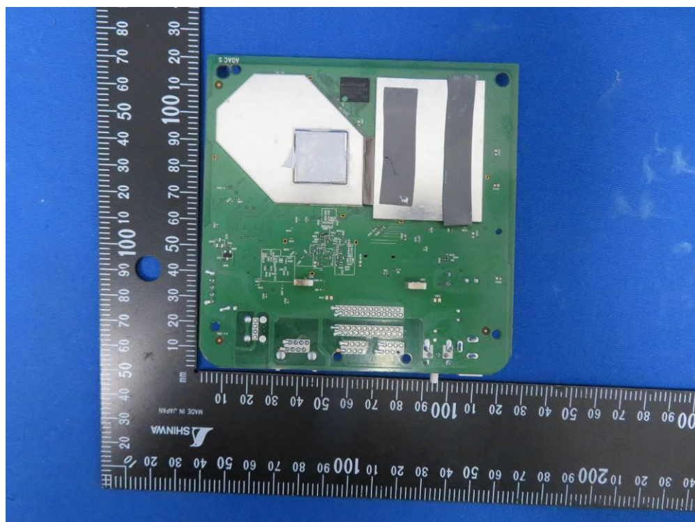
(4) EUT Photo (Model No.: GigaSpire BLAST u4m)
