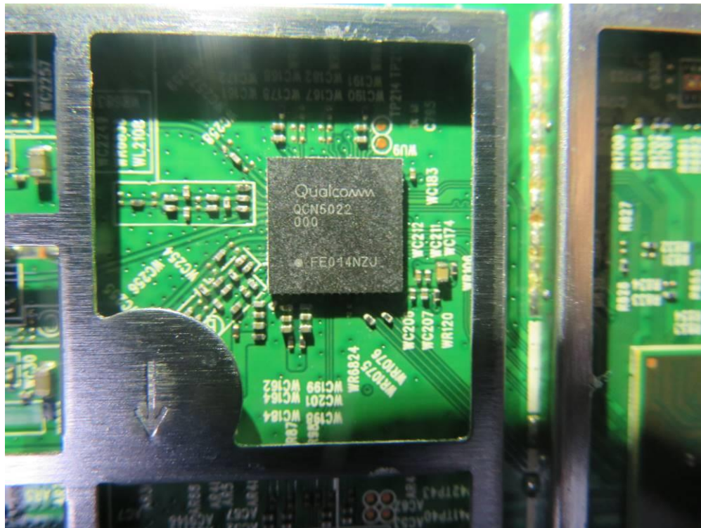
(23) EUT Photo (Model No.: GigaSpire BLAST u4)
