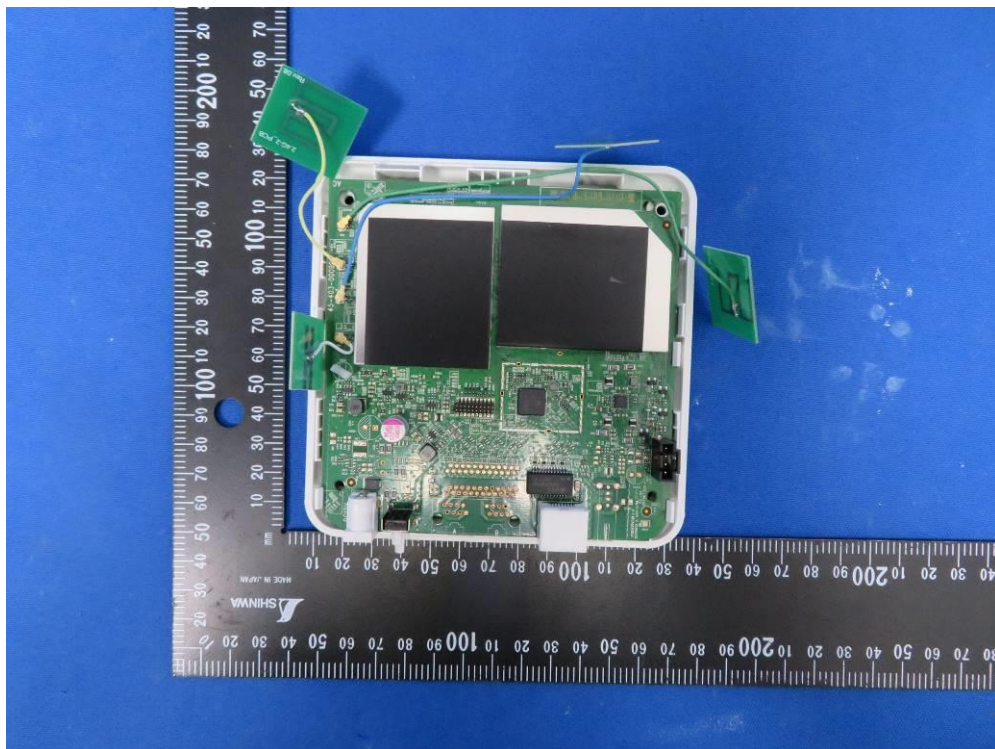
(2) EUT Photo (Model No.: GigaSpire BLAST u4m)
