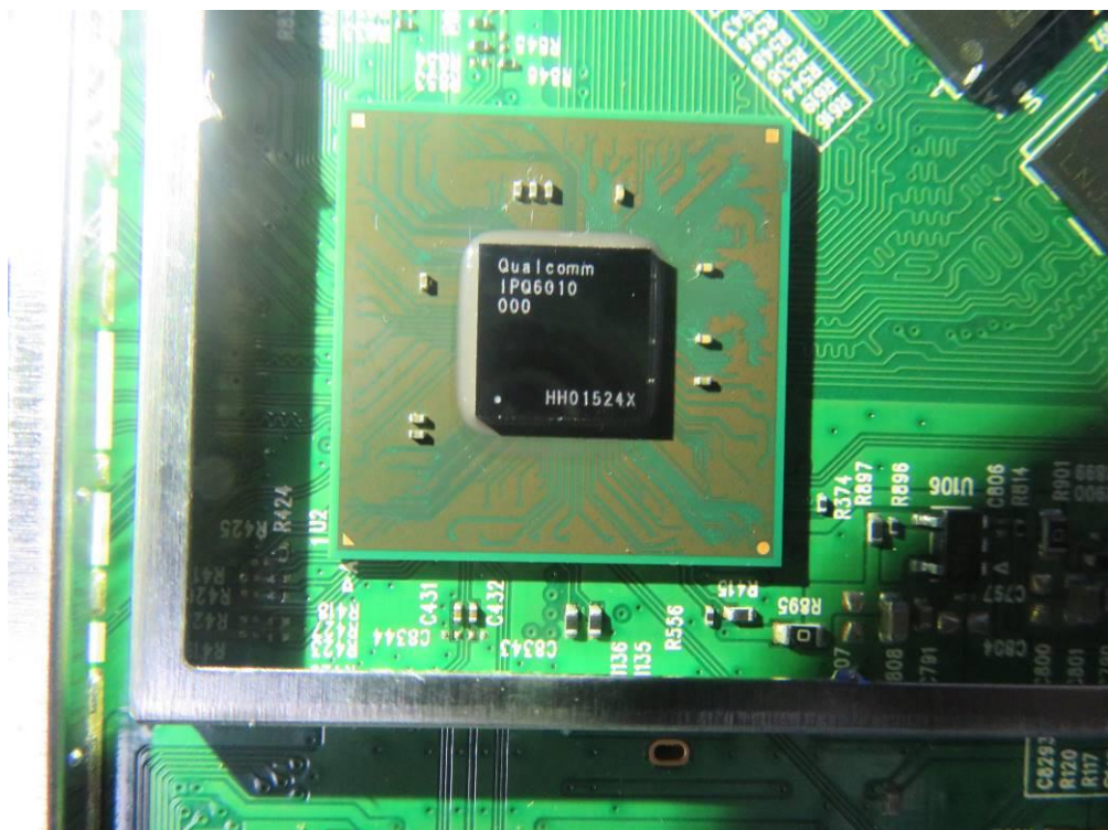
(22) EUT Photo (Model No.: GigaSpire BLAST u4)
