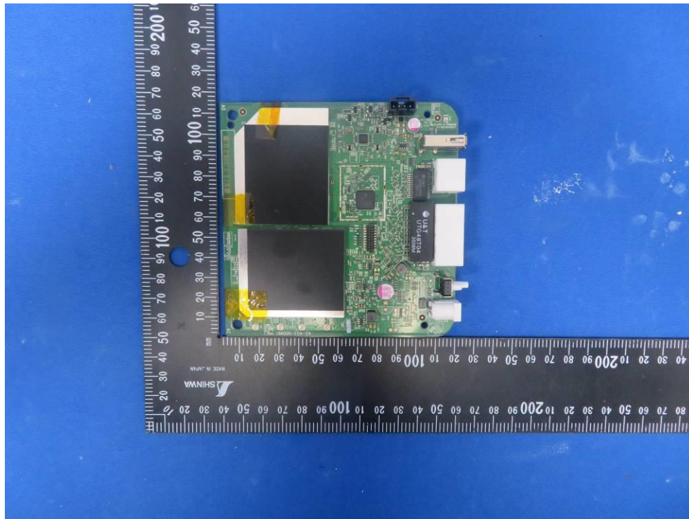
(19) EUT Photo (Model No.: GigaSpire BLAST u4)
