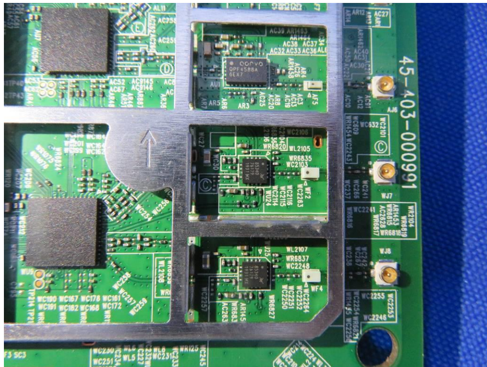
(13) EUT Photo (Model No.: GigaSpire BLAST u4m)
