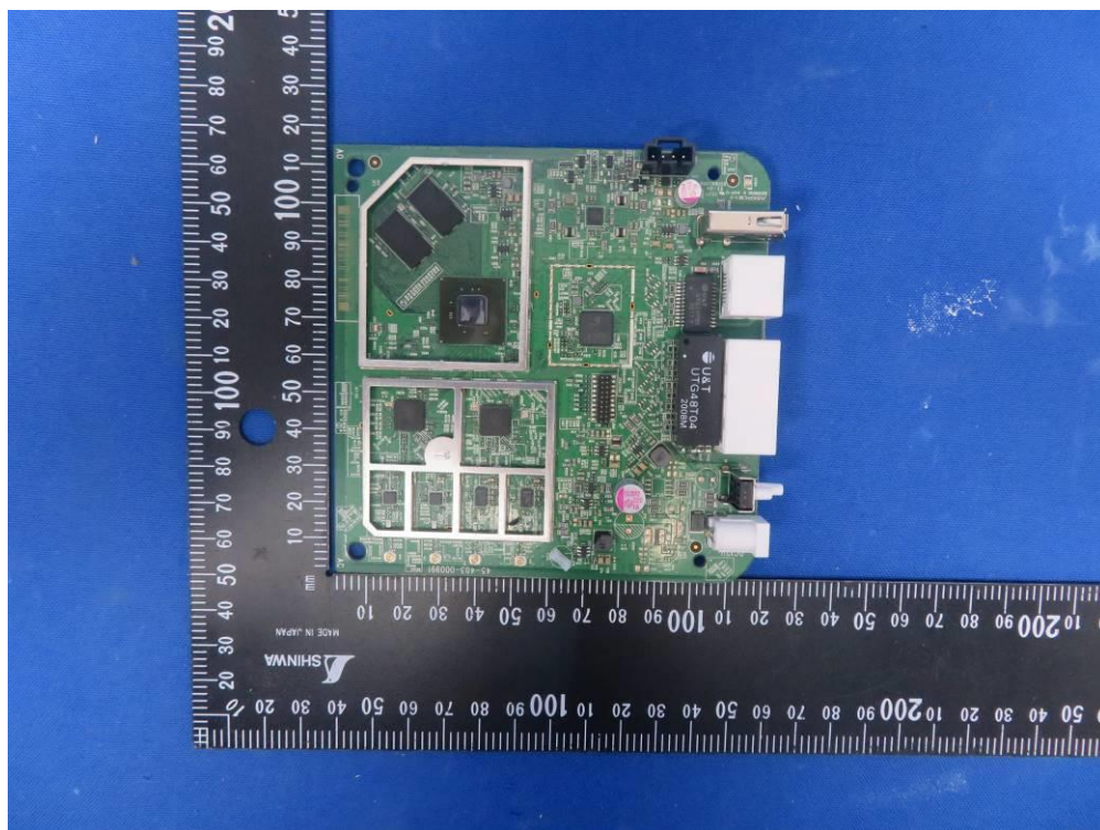
(20) EUT Photo (Model No.: GigaSpire BLAST u4)
