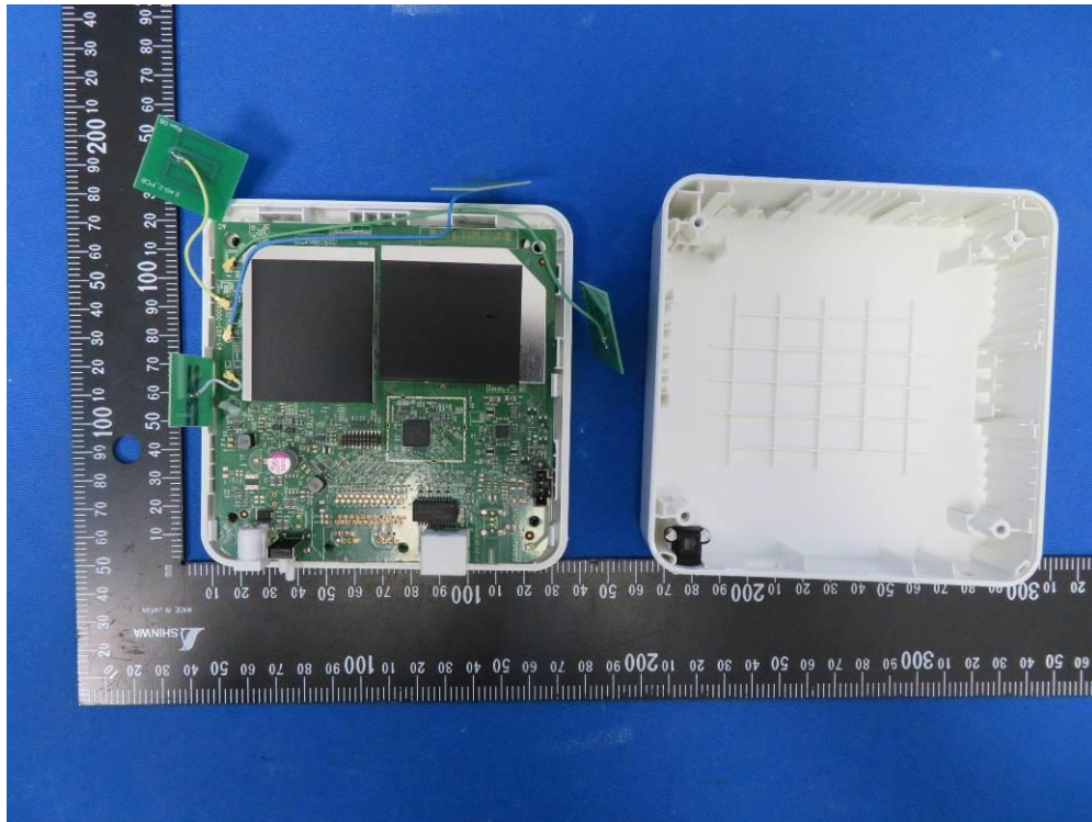
(1) EUT Photo (Model No.: GigaSpire BLAST u4m)
