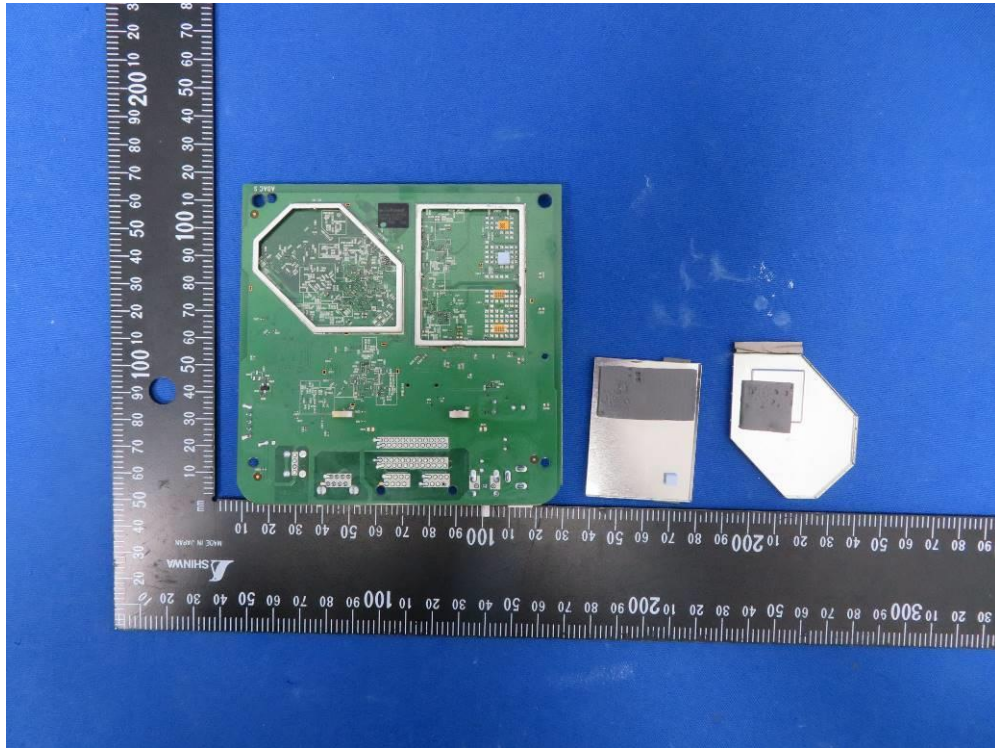
(5) EUT Photo (Model No.: GigaSpire BLAST u4m)
