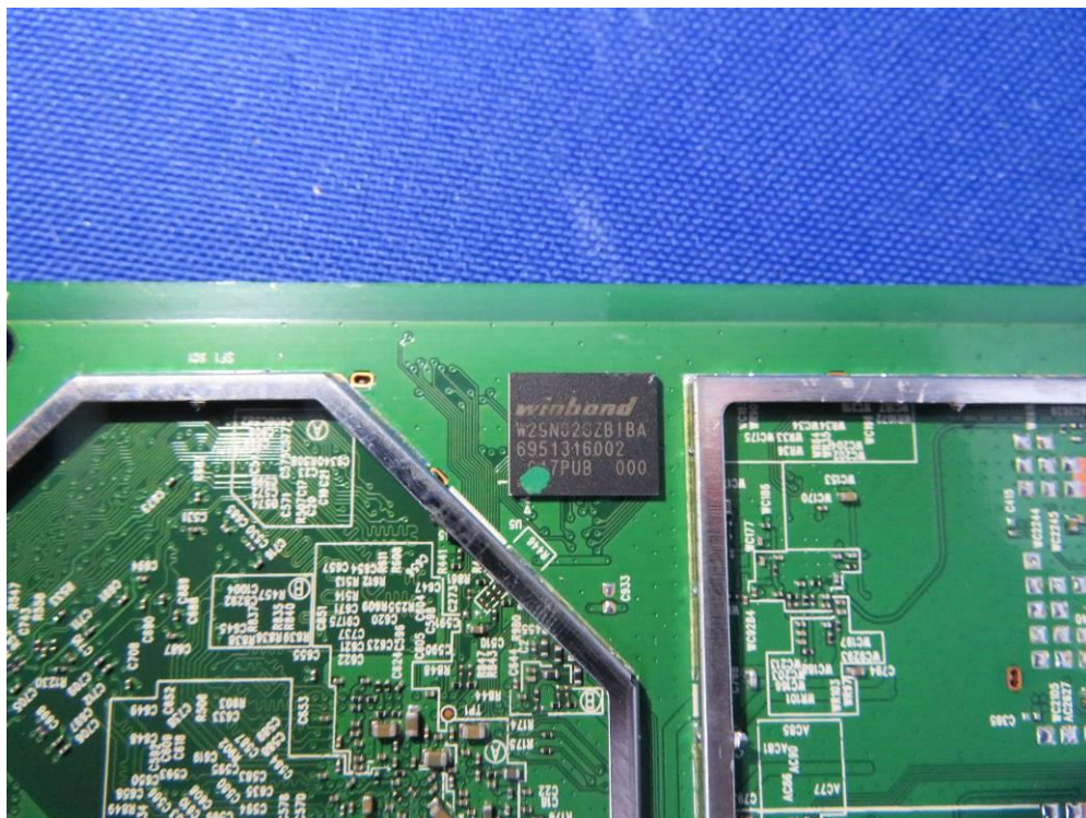
(6) EUT Photo (Model No.: GigaSpire BLAST u4m)
