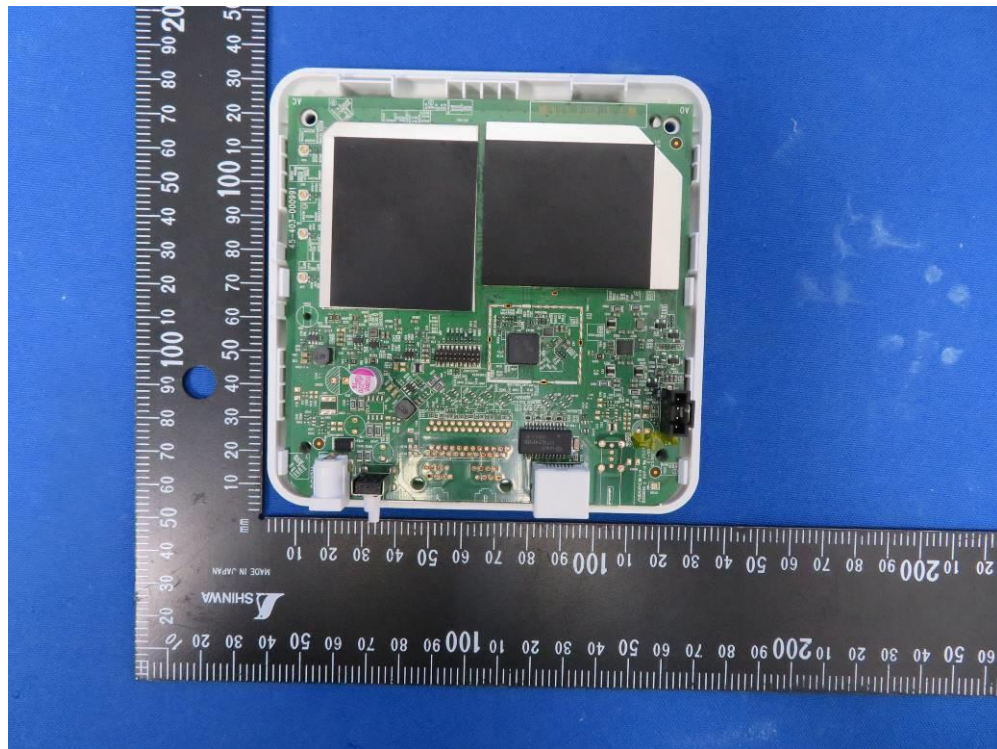
(3) EUT Photo (Model No.: GigaSpire BLAST u4m)
