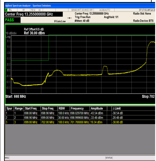
Band12_3MHz_16QAM_23025_1RB#14
