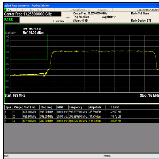
Band12_3MHz_16QAM_23025_15RB#0
