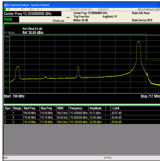
Band12_10MHz_16QAM_23130_1RB#49
