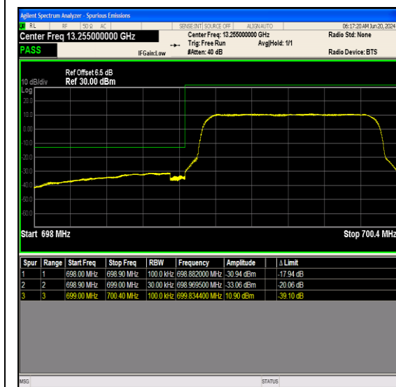
Band12_1.4MHz_QPSK_23017_6RB#0
