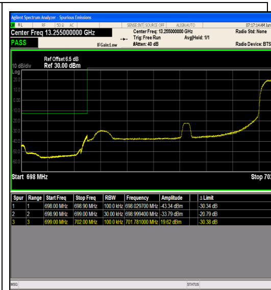
Band12_3MHz_64QAM_23025_1RB#14
