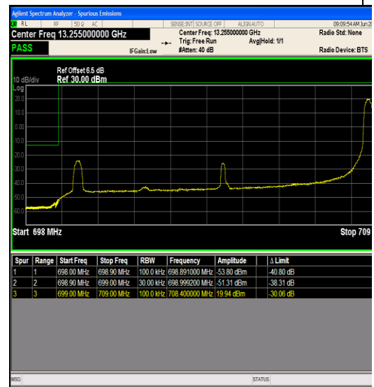
Band12_10MHz_64QAM_23060_1RB#49
