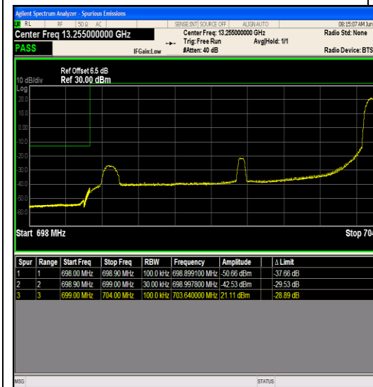
Band12_5MHz_QPSK_23035_1RB#24
