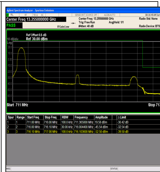
Band12_5MHz_64QAM_23155_1RB#0
