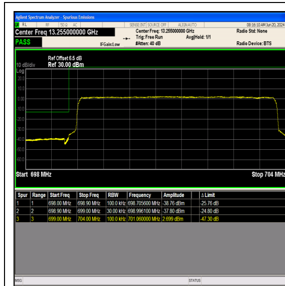
Band12_5MHz_64QAM_23035_25RB#0
