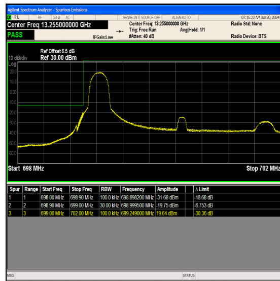
Band12_3MHz_16QAM_23025_1RB#0
