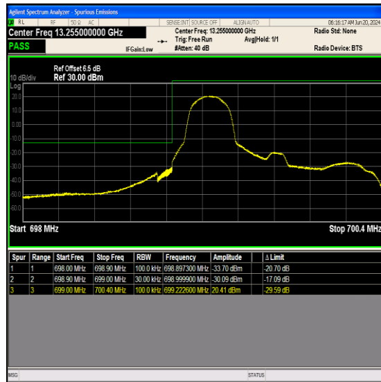
Band12_1.4MHz_16QAM_23017_1RB#0
