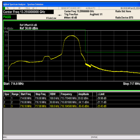
Band12_1.4MHz_64QAM_23173_1RB#5
