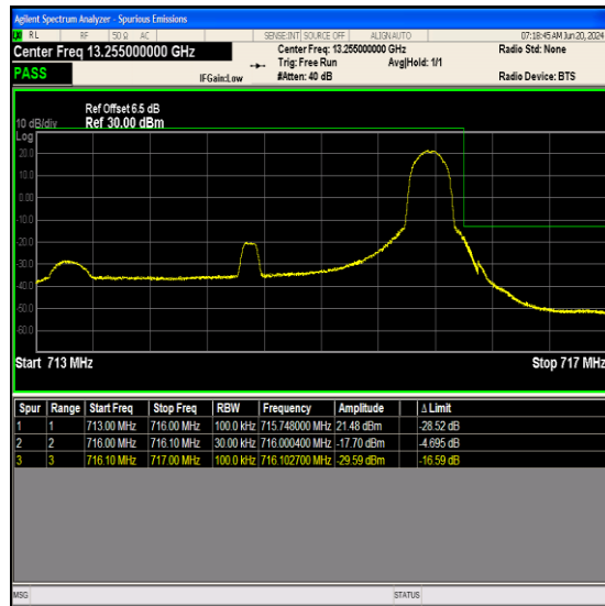
Band12_3MHz_QPSK_23165_1RB#14
