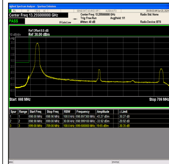
Band12_10MHz_16QAM_23060_1RB#0
