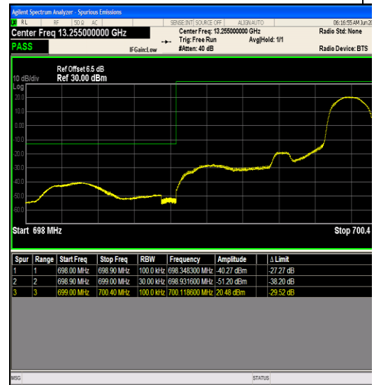
Band12_1.4MHz_16QAM_23017_1RB#5
