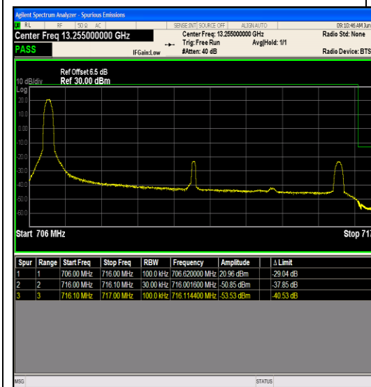
Band12_10MHz_QPSK_23130_1RB#0
