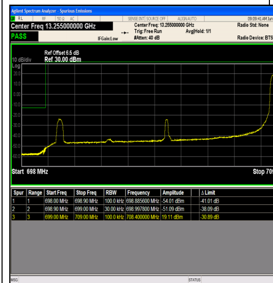
Band12_10MHz_16QAM_23060_1RB#49
