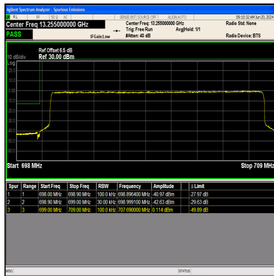
Band12_10MHz_64QAM_23060_50RB#0
