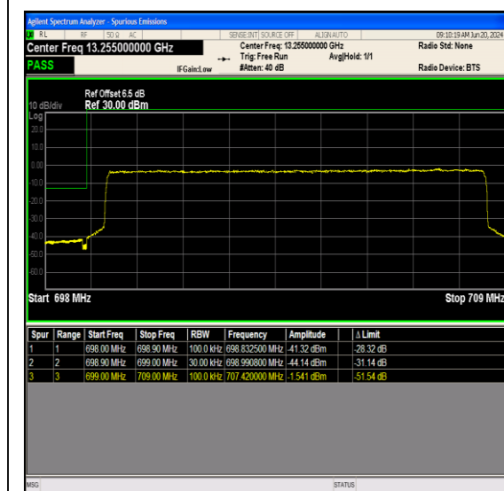
Band12_10MHz_16QAM_23060_1RB#0
