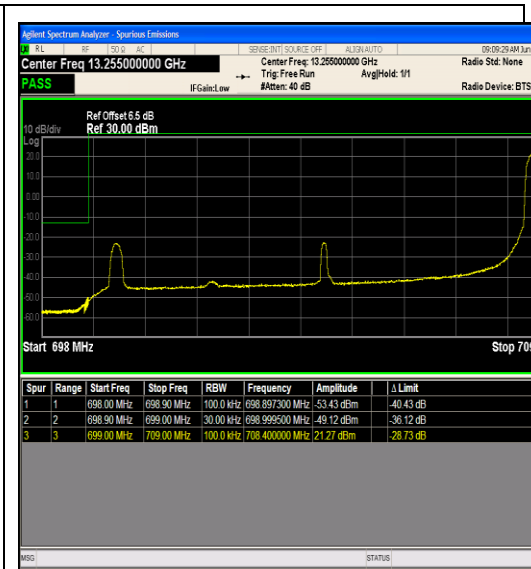
Band12_10MHz_QPSK_23060_1RB#49
