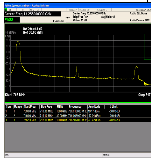
Band12_10MHz_64QAM_23130_1RB#0
