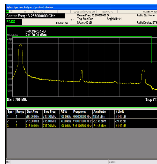
Band12_10MHz_16QAM_23060_1RB#49
