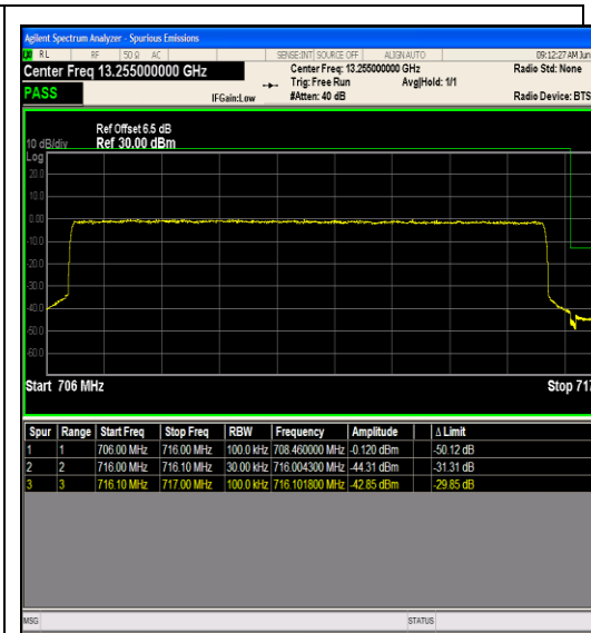
Band12_10MHz_64QAM_23130_50RB#0
