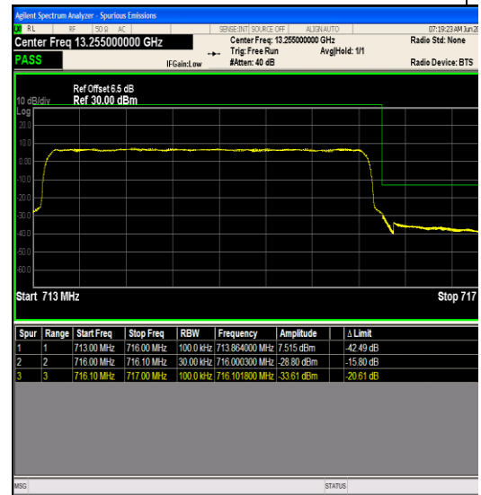
Band12_3MHz_QPSK_23165_15RB#0
