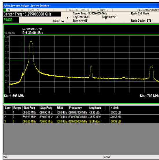
Band12_10MHz_64QAM_23060_1RB#0
