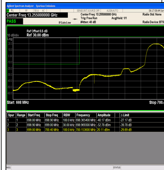
Band12_1.4MHz_64QAM_23017_1RB#5
