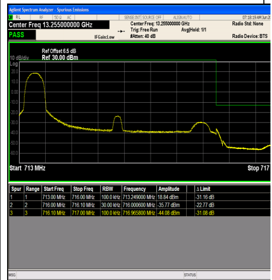
Band12_3MHz_16QAM_23165_1RB#0
