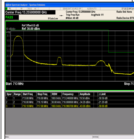
Band12_3MHz_64QAM_23165_1RB#0
