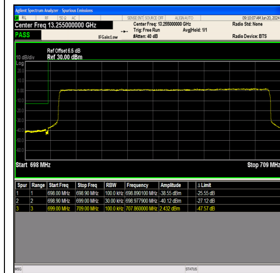
Band12_10MHz_QPSK_23060_50RB#0
