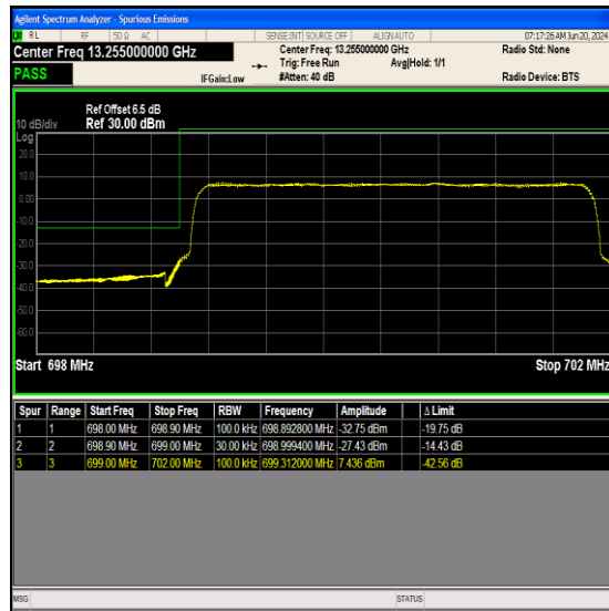
Band12_3MHz_QPSK_23025_15RB#0
