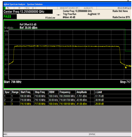
Band12_10MHz_16QAM_23130_50RB#0
