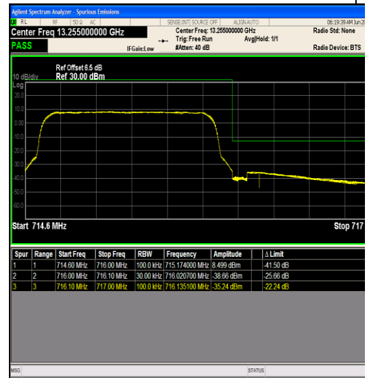
Band12_1.4MHz_64QAM_23173_6RB#0
