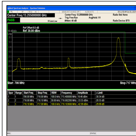
Band12_10MHz_64QAM_23130_1RB#49
