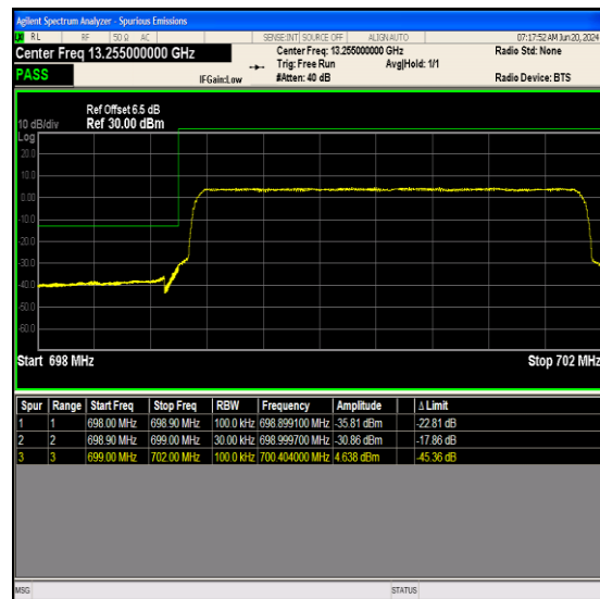
Band12_3MHz_64QAM_23025_15RB#0
