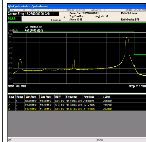
Band12_10MHz_QPSK_23060_50RB#0
