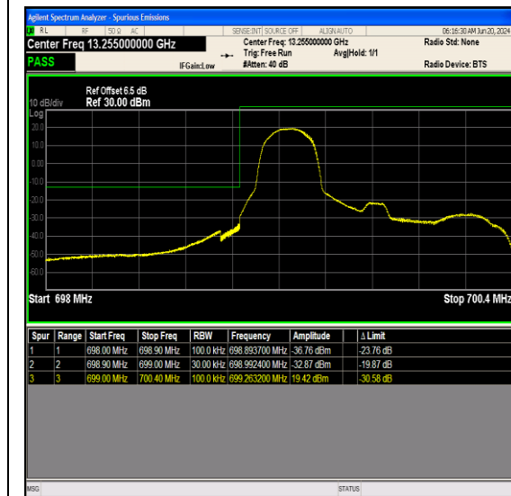
Band12_1.4MHz_64QAM_23017_1RB#0
