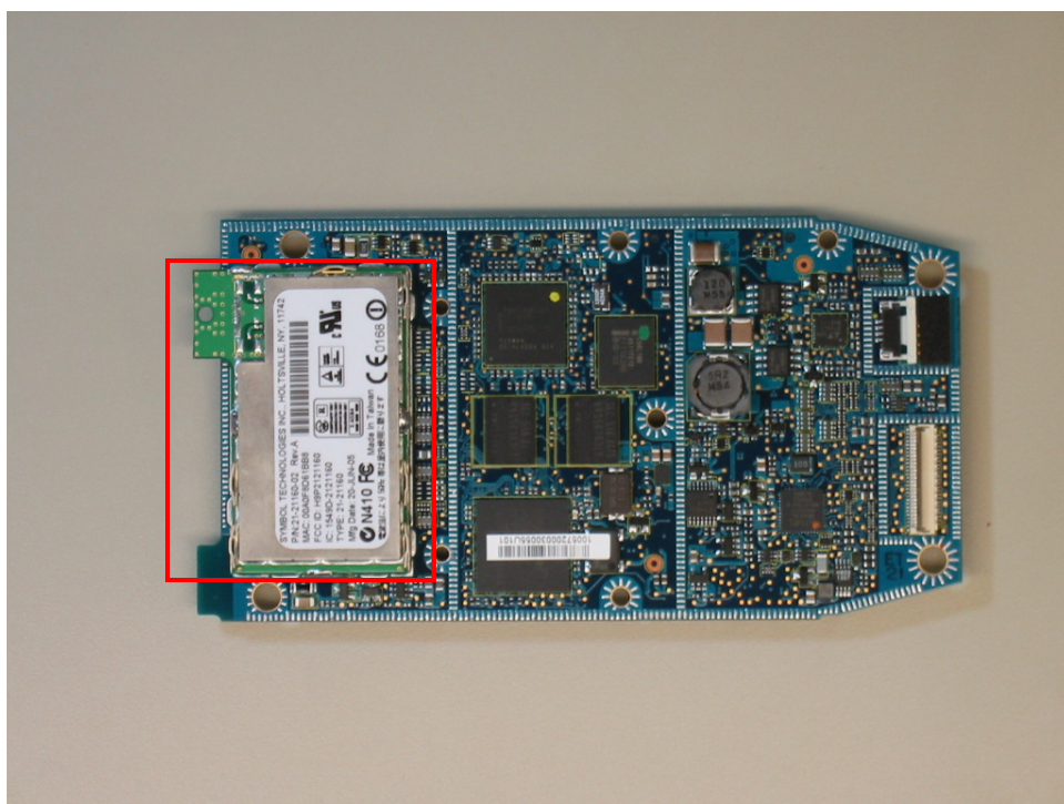
WLAN radio
