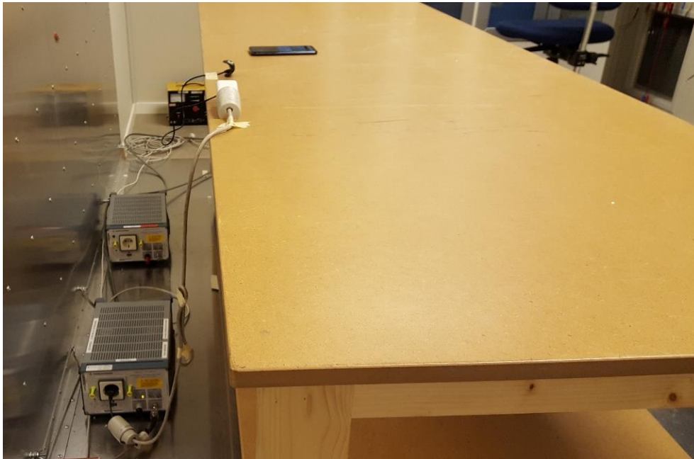
Photo 5 - Conducted emission test setup.
