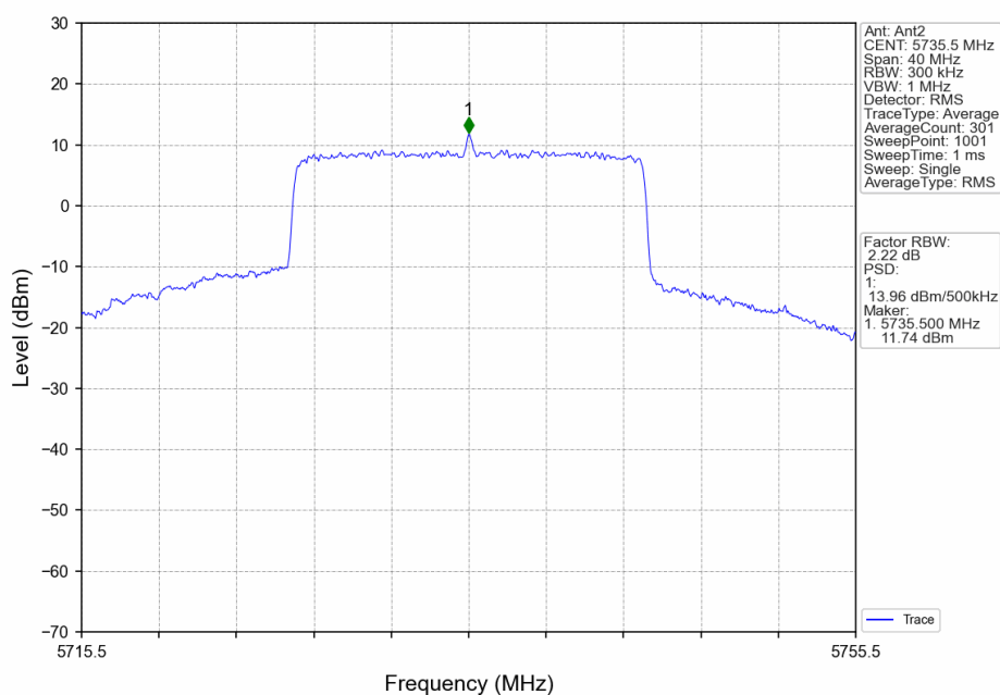
20M_LCH_5735.5MHz_Ant2_NTNV
