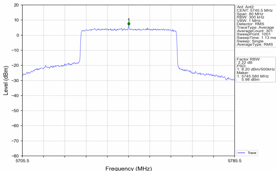
40M_LCH_5745.5MHz_MIMO_NTNV
