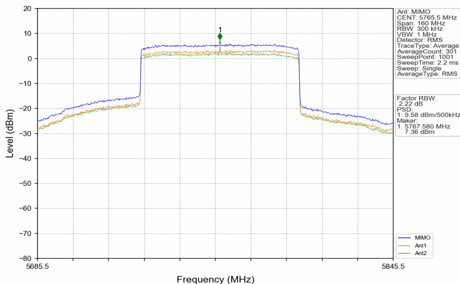
80M_LCH_5765.5MHz_MIMO_NTNV
