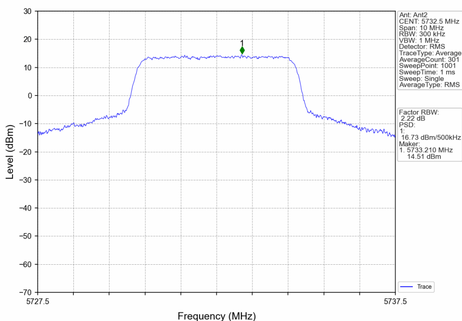
5M_LCH_5732.5MHz_Ant2_NTNV
