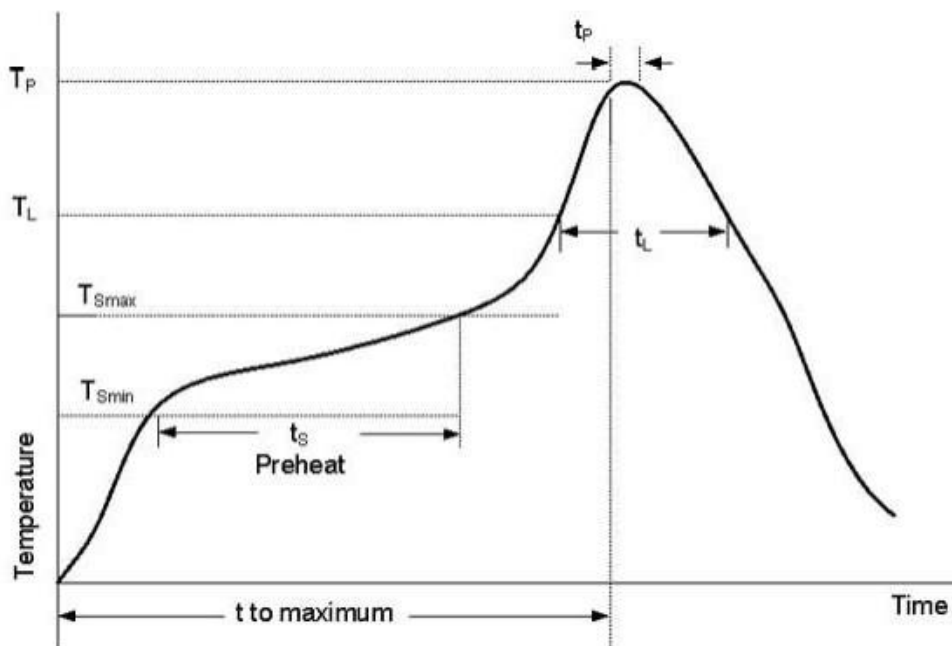
Figure 5-2-3: Reflow Profile
