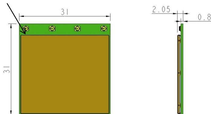
Figure 5-1-1Top & side view
