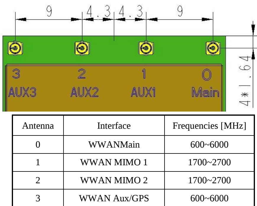
Figure 2-2-1 Antenna connector location and type
