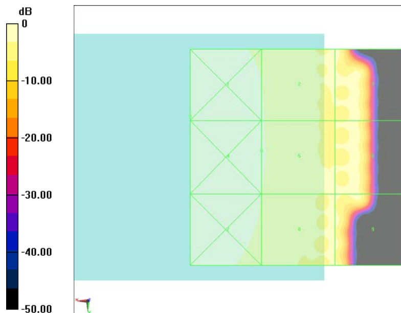
Fig B.9 HAC RF H-Field GSM 850 Low
