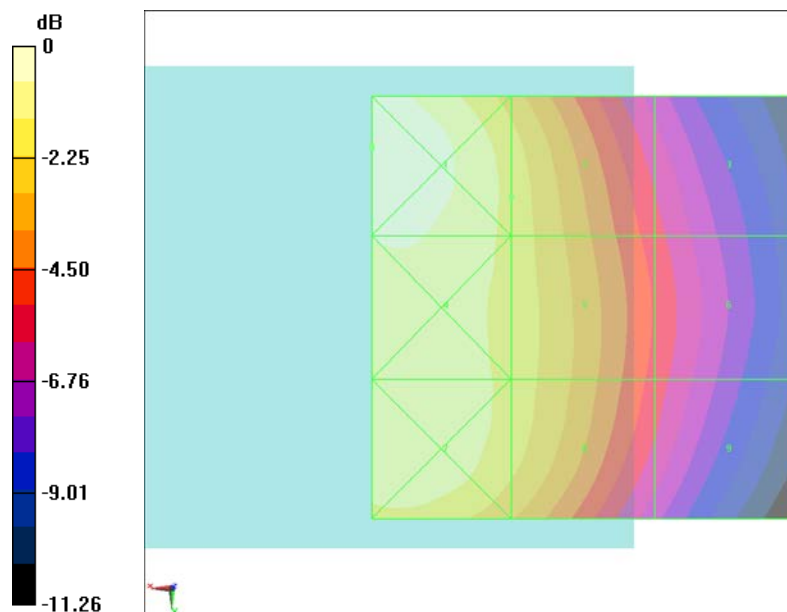
Fig B.10 HAC RF H-Field GSM 1900 High
