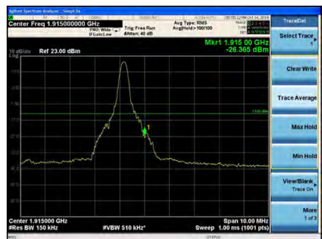
LTE Band 25 15MHz QPSK 1RB CH-High
