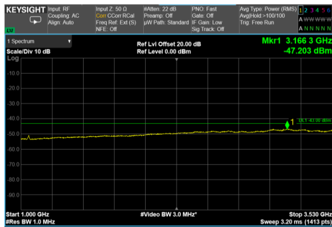
Channel: MIDDLE, Modulation: 64QAM, BW=20MHz, Range: 1000 MHz – 3530 MHz
