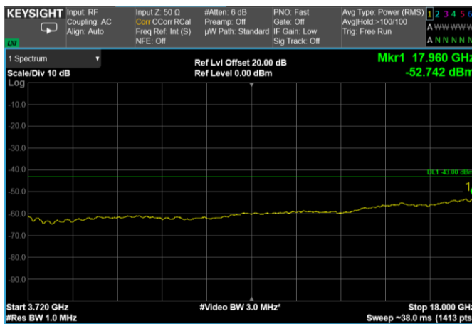
Channel: TOP, Modulation: 64QAM, BW=30MHz, Range: 3720 MHz - 18 GHz
