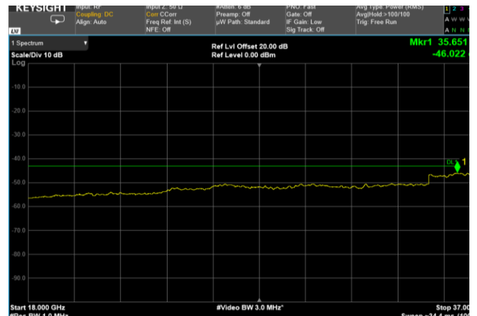
Channel: BOTTOM, Modulation: 64QAM, BW=30MHz, Range: 18 GHz - 37 GHz
