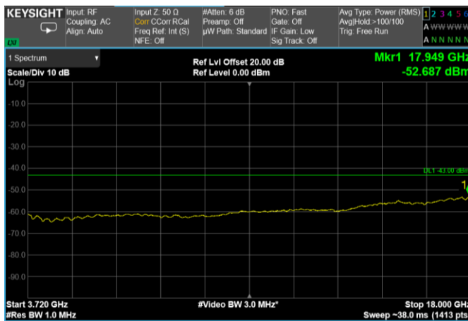
Channel: BOTTOM, Modulation: 64QAM, BW=40MHz, Range: 3720 MHz - 18 GHz
