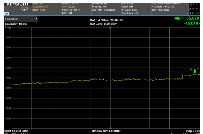
Channel: MIDDLE, Modulation: 64QAM, BW=30MHz, Range: 18 GHz – 37 GHz
