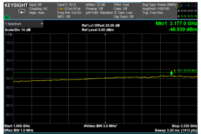
Channel: TOP, Modulation: 64QAM, BW=40MHz, Range: 1000 MHz - 3530 MHz
