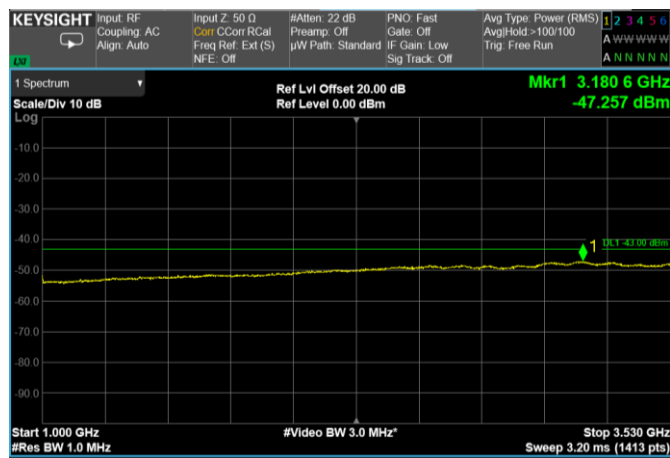
Channel: BOTTOM, Modulation: 64QAM, BW=15MHz, Range: 1000 MHz - 3530 MHz
