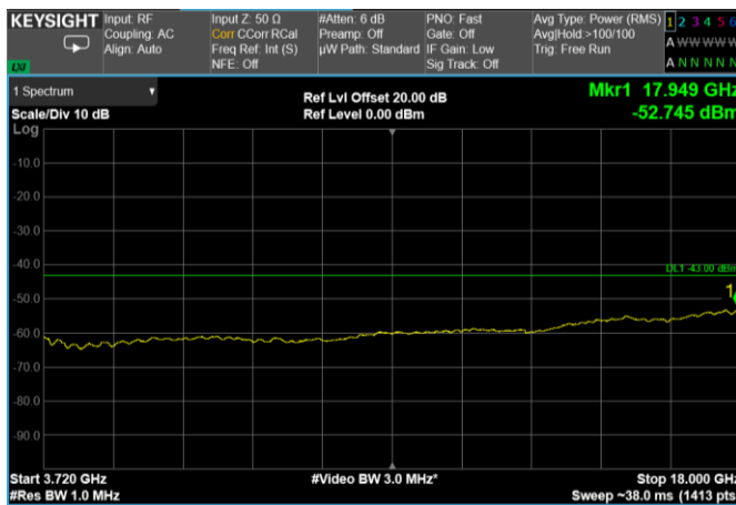
Channel: TOP, Modulation: 64QAM, BW=50MHz, Range: 3720 MHz - 18 GHz
