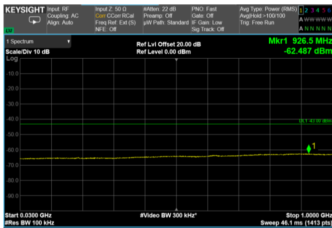
Channel: MIDDLE, Modulation: 64QAM, BW=20MHz, Range: 30 MHz – 1000 MHz
