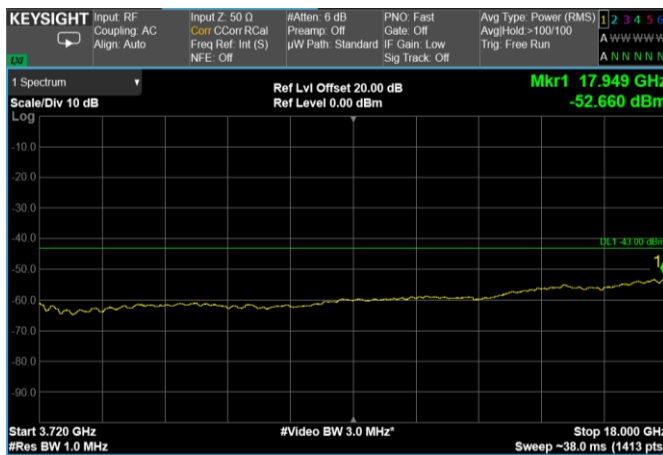
Channel: TOP, Modulation: 64QAM, BW=20MHz, Range: 3720 MHz - 18 GHz
