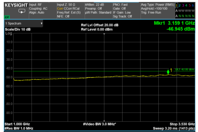
Channel: BOTTOM, Modulation: 64QAM, BW=25MHz, Range: 1000 MHz - 3530 MHz
