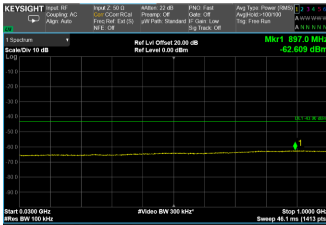
Channel: TOP, Modulation: 64QAM, BW=40MHz, Range: 30 MHz - 1000 MHz
