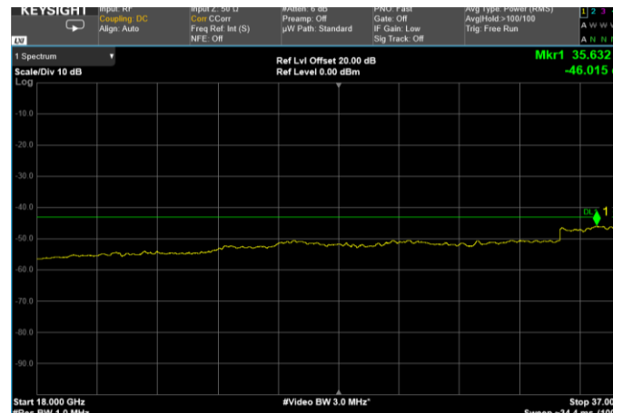
Channel: BOTTOM, Modulation: 64QAM, BW=60MHz, Range: 18 GHz - 37 GHz
