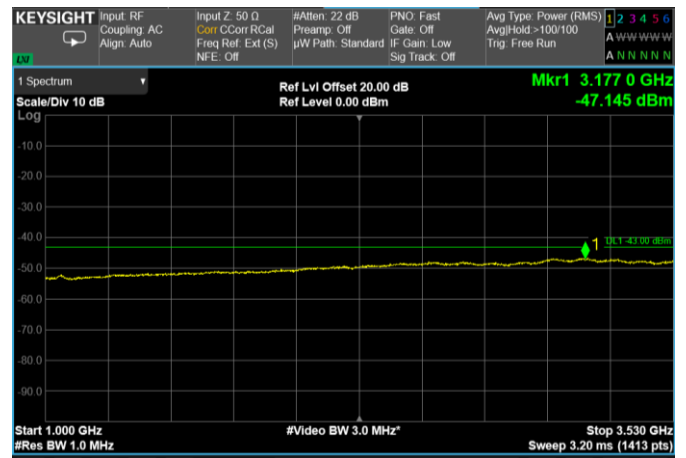
Channel: MIDDLE, Modulation: 64QAM, BW=50MHz, Range: 1000 MHz – 3530 MHz
