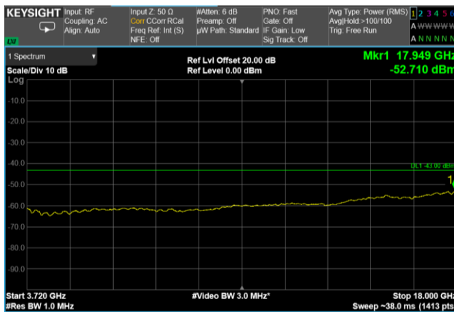
Channel: BOTTOM, Modulation: 64QAM, BW=60MHz, Range: 3720 MHz - 18 GHz
