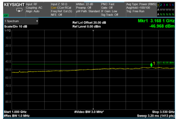
Channel: TOP, Modulation: 64QAM, BW=30MHz, Range: 1000 MHz - 3530 MHz
