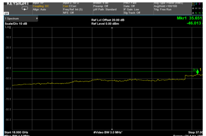
Channel: MIDDLE, Modulation: 64QAM, BW=15MHz, Range: 18 GHz - 37 GHz
