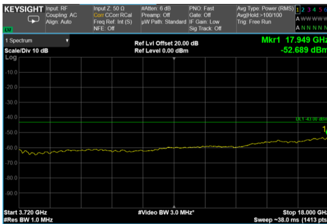
Channel: TOP, Modulation: 64QAM, BW=25MHz, Range: 3720 MHz - 18 GHz
