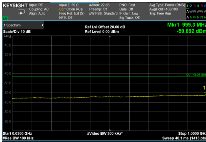
Channel: BOTTOM, Modulation: 64QAM, BW=20MHz, Range: 30 MHz - 1000 MHz
