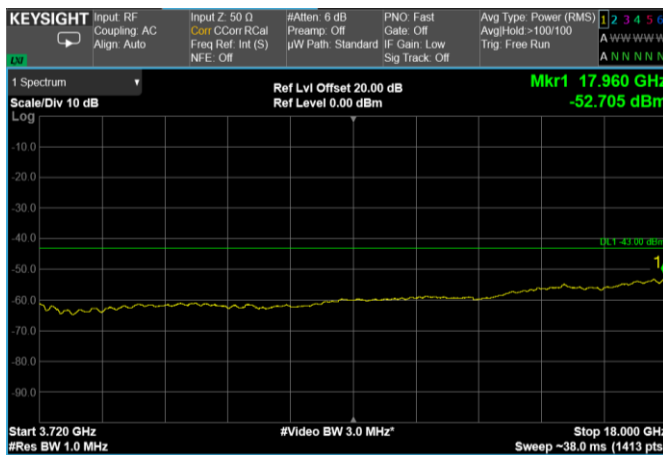
Channel: MIDDLE, Modulation: 64QAM, BW=50MHz, Range: 3720 MHz – 18 GHz
