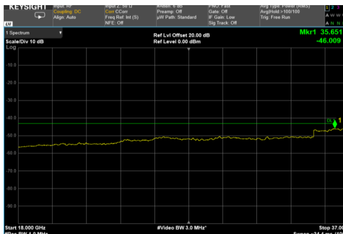
Channel: BOTTOM, Modulation: 64QAM, BW=15MHz, Range: 18 GHz - 37 GHz
