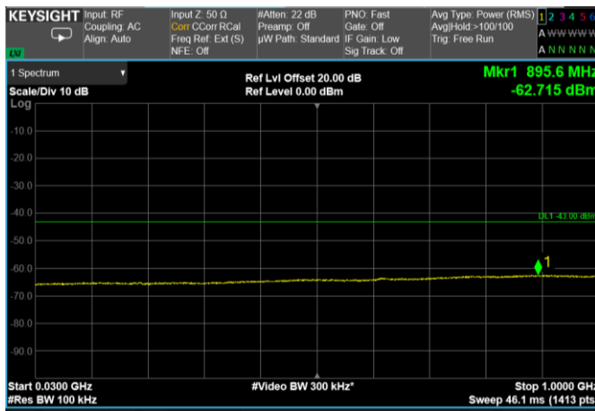
Channel: MIDDLE, Modulation: 64QAM, BW=15MHz, Range: 30 MHz - 1000 MHz
