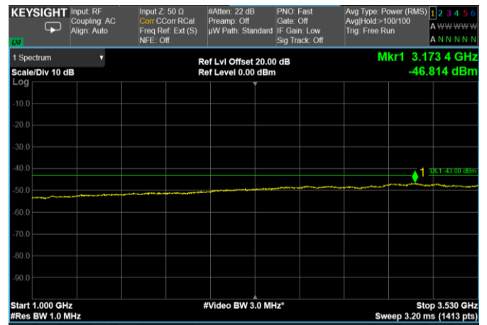
Channel: TOP, Modulation: 64QAM, BW=50MHz, Range: 1000 MHz - 3530 MHz
