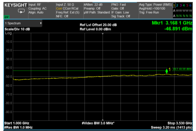
Channel: BOTTOM, Modulation: 64QAM, BW=20MHz, Range: 1000 MHz - 3530 MHz
