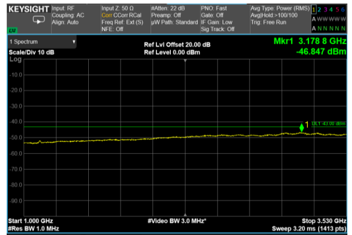
Channel: TOP, Modulation: 64QAM, BW=25MHz, Range: 1000 MHz - 3530 MHz
