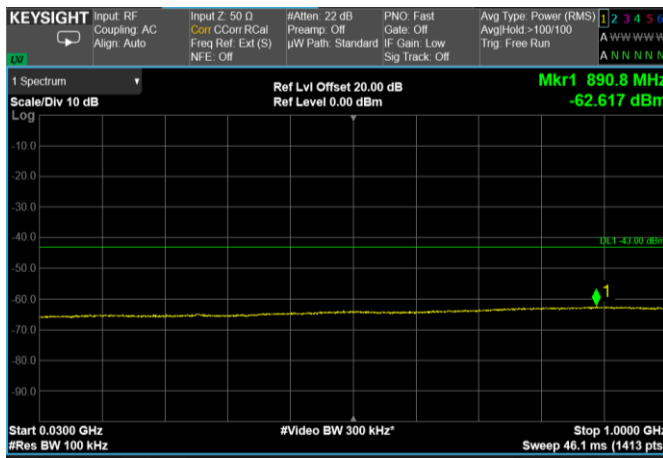
Channel: TOP, Modulation: 64QAM, BW=20MHz, Range: 30 MHz - 1000 MHz
