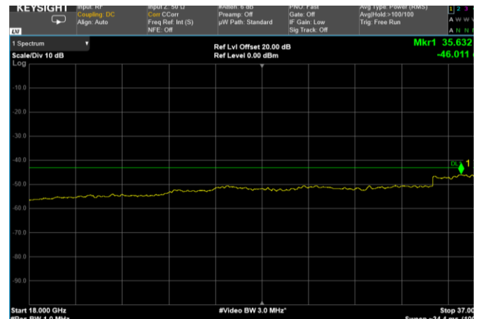
Channel: TOP, Modulation: 64QAM, BW=25MHz, Range: 18 GHz - 37 GHz
