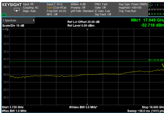
Channel: BOTTOM, Modulation: 64QAM, BW=25MHz, Range: 3720 MHz - 18 GHz
