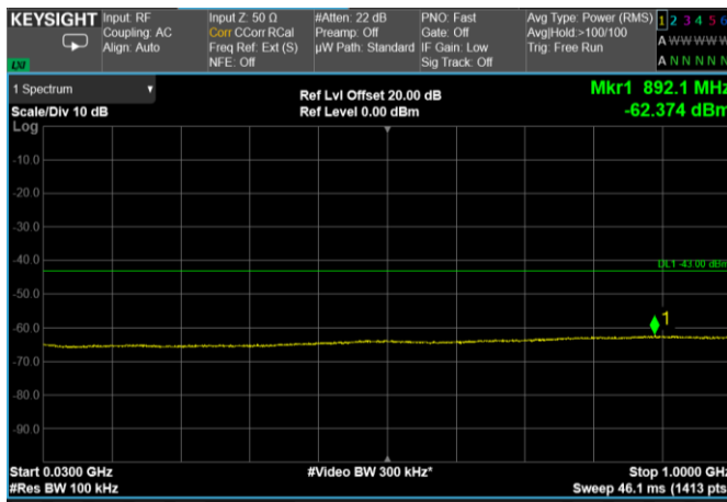
Channel: BOTTOM, Modulation: 64QAM, BW=60MHz, Range: 30 MHz - 1000 MHz
