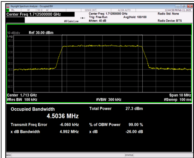
Band4-5MHz-64QAM-20375-25RB#0
