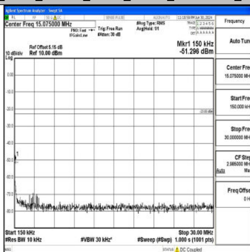
Band26_3MHz_16QAM_27025_1RB#0_0.15~30_0.15~30
