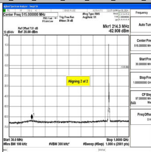
Band26_5MHz_16QAM_26915_1RB#0_30~1000_30~1000
