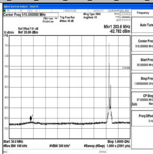
Band26_15MHz_16QAM_26915_1RB#0_30~1000_30~1000
