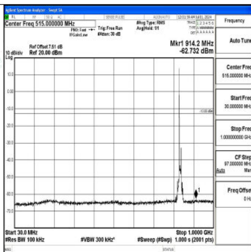
Band26_10MHz_QPSK_26915_1RB#0_30~1000_30~1000
