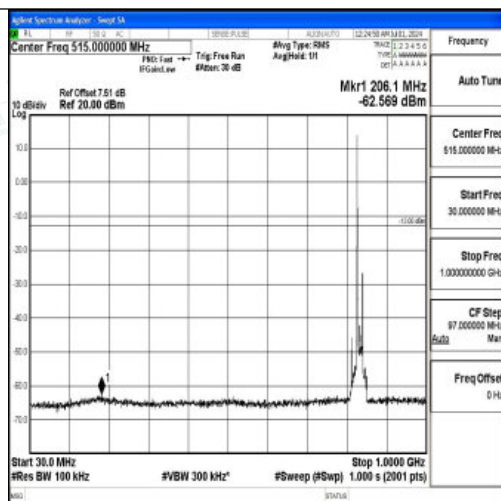
Band26_15MHz_QPSK_26915_1RB#0_30~1000_30~1000
