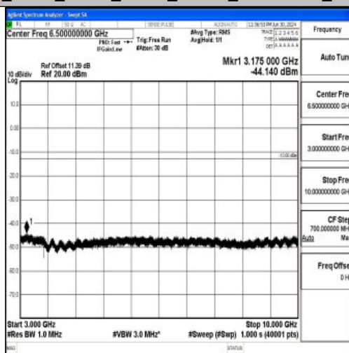
Band26_5MHz_QPSK_26915_1RB#0_3000~10000_3000~10000
