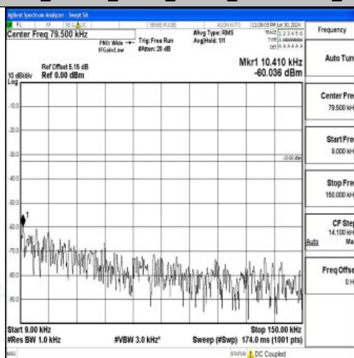
Band26_3MHz_QPSK_26915_1RB#0_0.009~0.15_0.009~0.15
