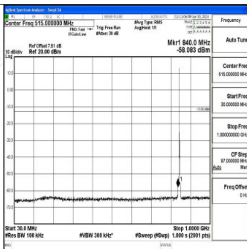
Band26_3MHz_16QAM_27025_1RB#0_30~1000_30~1000
