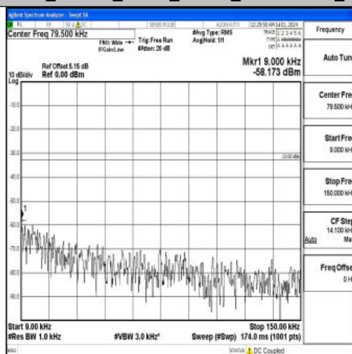
Band26_15MHz_QPSK_26965_1RB#0_0.009~0.15_0.009~0.15
