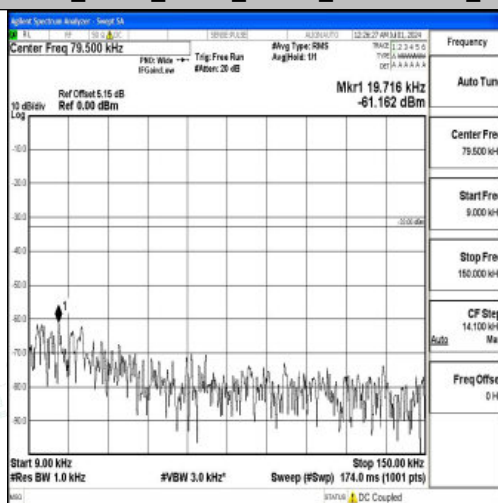
Band26_15MHz_16QAM_26965_1RB#0_0.009~0.15_0.009~0.15
