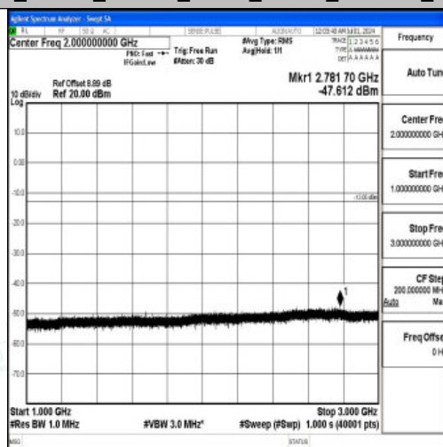
Band26_10MHz_16QAM_26990_1RB#0_1000~3000_1000~3000
