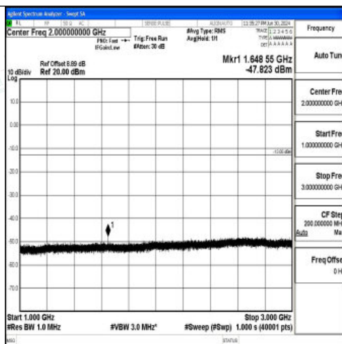
Band26_5MHz_QPSK_26815_1RB#0_1000~3000_1000~3000
