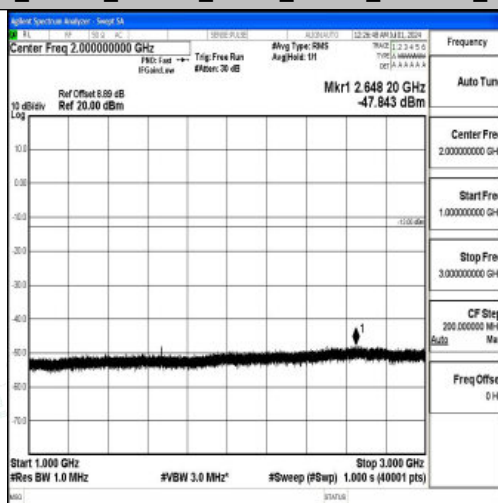
Band26_15MHz_16QAM_26965_1RB#0_1000~3000_1000~3000
