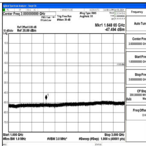
Band26_3MHz_QPSK_26805_1RB#0_1000~3000_1000~3000
