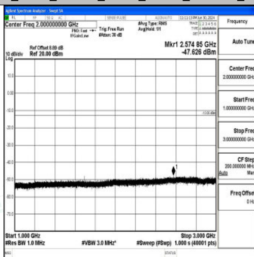
Band26_3MHz_16QAM_27025_1RB#0_1000~3000_1000~3000
