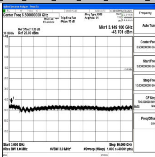
Band26_3MHz_16QAM_26915_1RB#0_3000~10000_3000~10000
