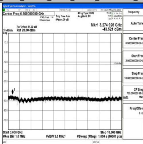
Band26_3MHz_16QAM_27025_1RB#0_3000~10000_3000~10000
