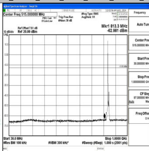
Band26_10MHz_QPSK_26990_1RB#0_30~1000_30~1000
