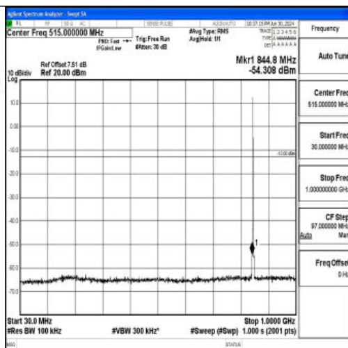
Band26_1.4MHz_16QAM_27033_1RB#0_30~1000_30~1000
