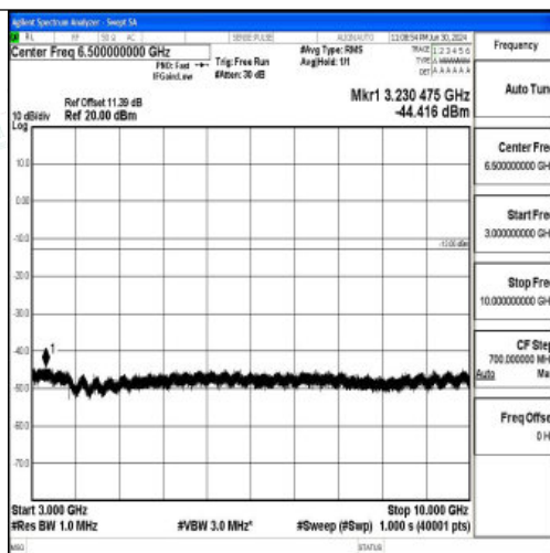
Band26_3MHz_16QAM_26805_1RB#0_3000~10000_3000~10000
