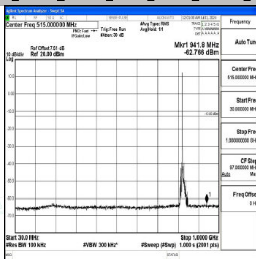
Band26_10MHz_16QAM_26840_1RB#0_30~1000_30~1000
