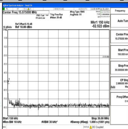
Band26_3MHz_16QAM_26915_1RB#0_0.15~30_0.15~30
