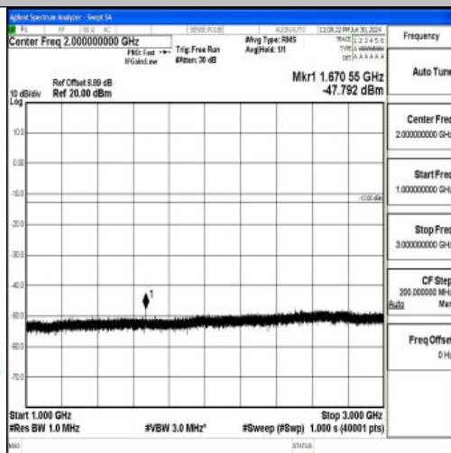
Band26_3MHz_QPSK_26915_1RB#0_1000~3000_1000~3000
