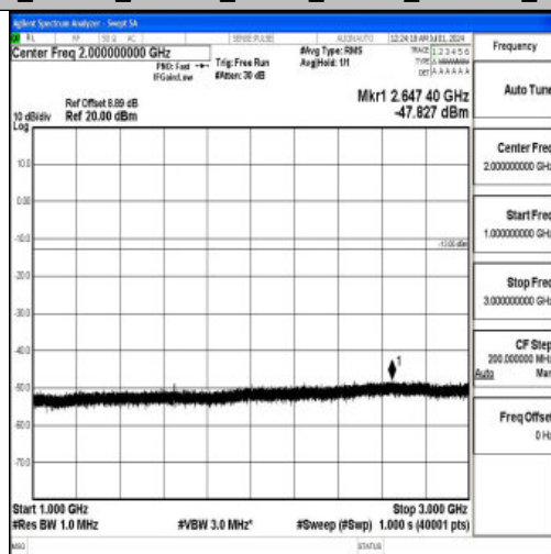
Band26_15MHz_16QAM_26865_1RB#0_1000~3000_1000~3000
