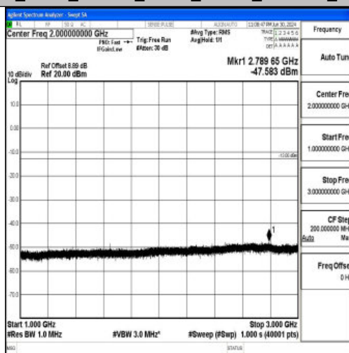
Band26_3MHz_16QAM_26805_1RB#0_1000~3000_1000~3000
