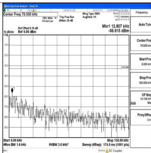
Band26_5MHz_16QAM_26915_1RB#0_0.009~0.15_0.009~0.15
