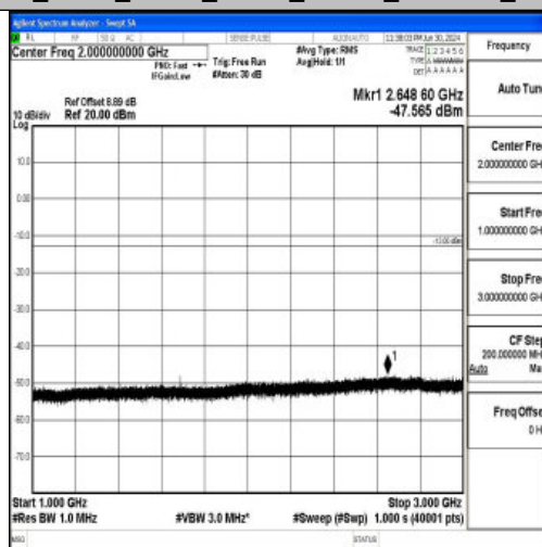
Band26_5MHz_QPSK_27015_1RB#0_1000~3000_1000~3000
