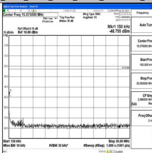
Band26_3MHz_QPSK_26915_1RB#0_0.15~30_0.15~30
