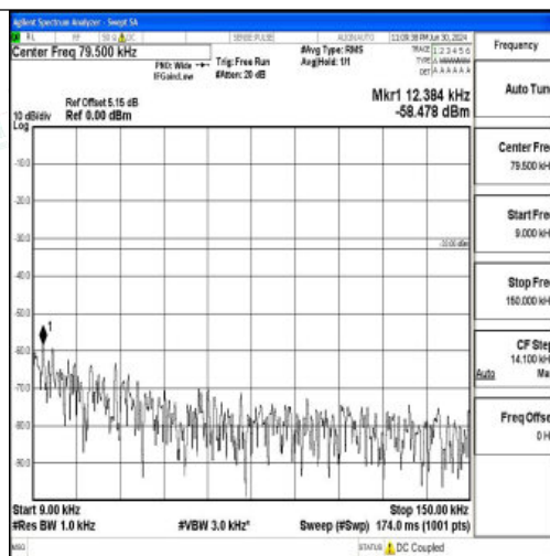
Band26_3MHz_16QAM_26915_1RB#0_0.009~0.15_0.009~0.15
