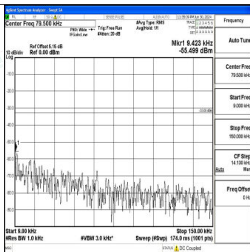
Band26_5MHz_QPSK_26815_1RB#0_0.009~0.15_0.009~0.15
