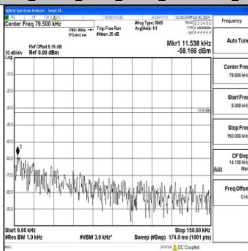
Band26_5MHz_QPSK_26915_1RB#0_0.009~0.15_0.009~0.15
