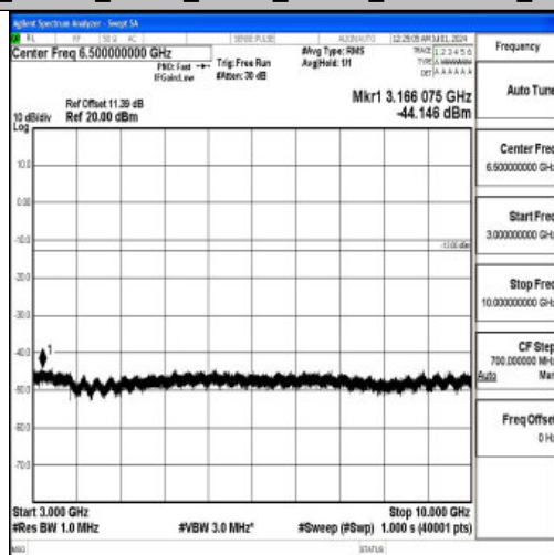
Band26_15MHz_QPSK_26915_1RB#0_3000~10000_3000~10000
