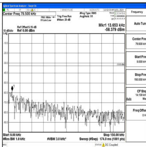
Band26_10MHz_16QAM_26915_1RB#0_0.009~0.15_0.009~0.15
