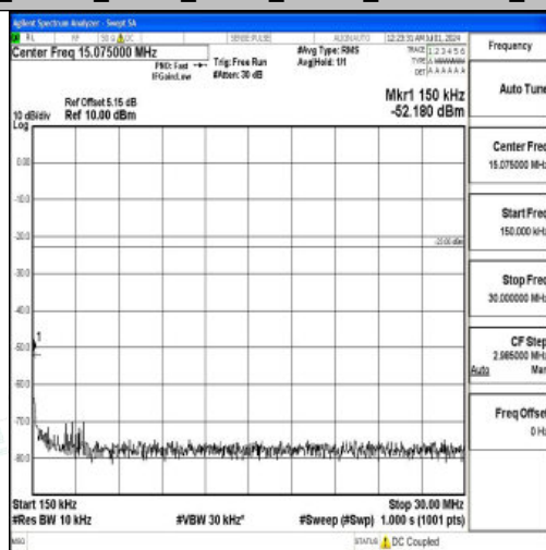
Band26_15MHz_QPSK_26865_1RB#0_0.15~30_0.15~30
