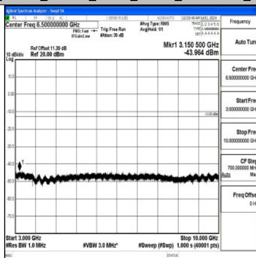
Band26_10MHz_16QAM_26990_1RB#0_3000~10000_3000~10000
