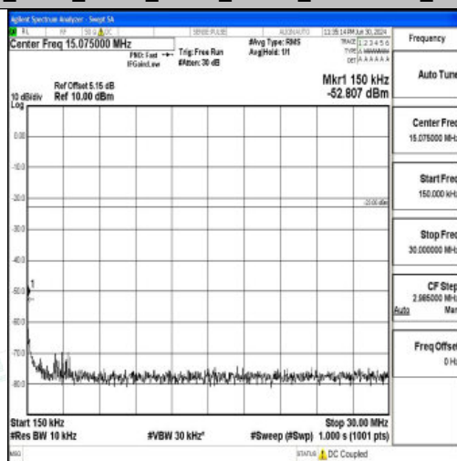
Band26_5MHz_QPSK_26815_1RB#0_0.15~30_0.15~30
