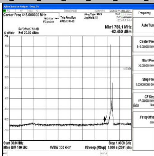
Band26_15MHz_QPSK_26965_1RB#0_30~1000_30~1000
