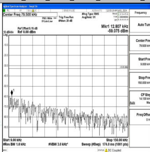
Band26_10MHz_16QAM_26990_1RB#0_0.009~0.15_0.009~0.15
