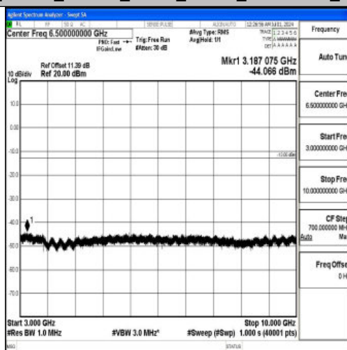
Band26_15MHz_16QAM_26965_1RB#0_3000~10000_3000~10000
