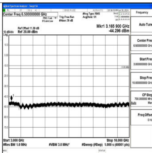
Band26_1.4MHz_QPSK_27033_1RB#0_3000~10000_3000~10000
