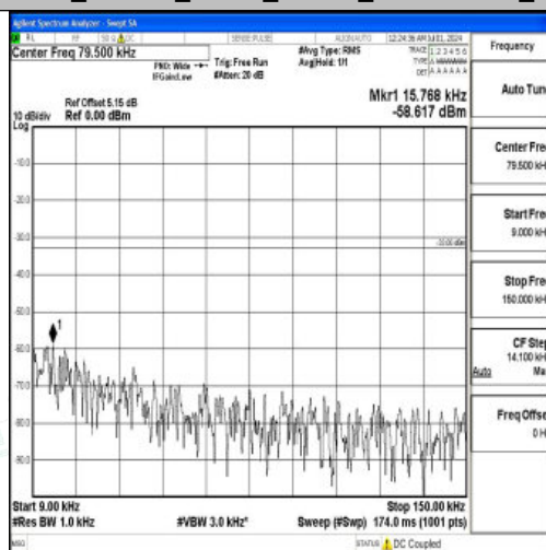
Band26_15MHz_QPSK_26915_1RB#0_0.009~0.15_0.009~0.15
