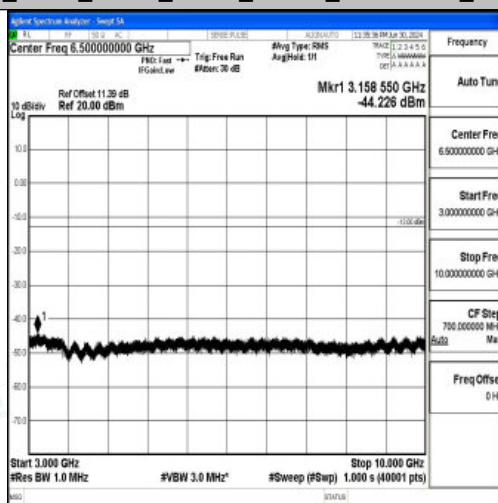
Band26_5MHz_QPSK_26815_1RB#0_3000~10000_3000~10000
