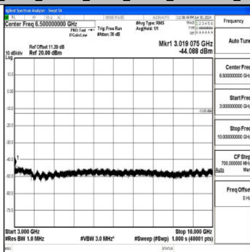
Band26_5MHz_16QAM_27015_1RB#0_3000~10000_3000~10000
