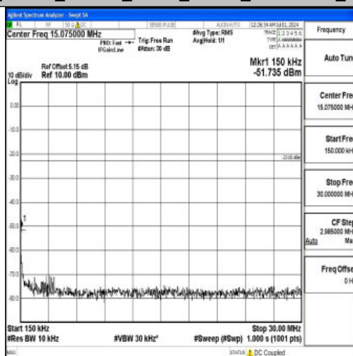
Band26_15MHz_16QAM_26965_1RB#0_0.15~30_0.15~30
