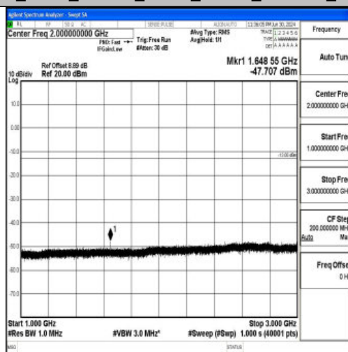
Band26_5MHz_16QAM_26815_1RB#0_1000~3000_1000~3000
