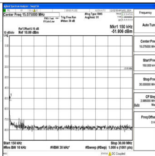
Band26_10MHz_QPSK_26990_1RB#0_0.15~30_0.15~30
