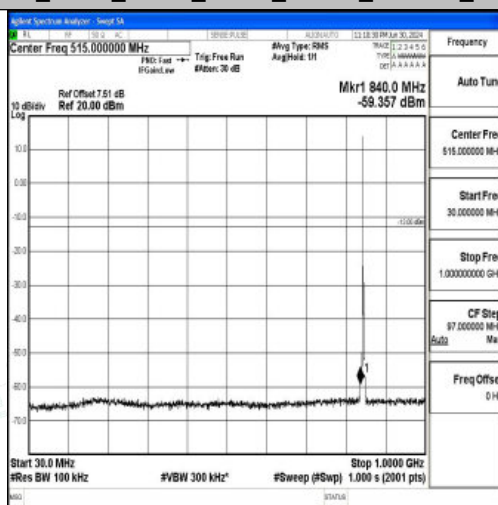
Band26_3MHz_QPSK_27025_1RB#0_30~1000_30~1000
