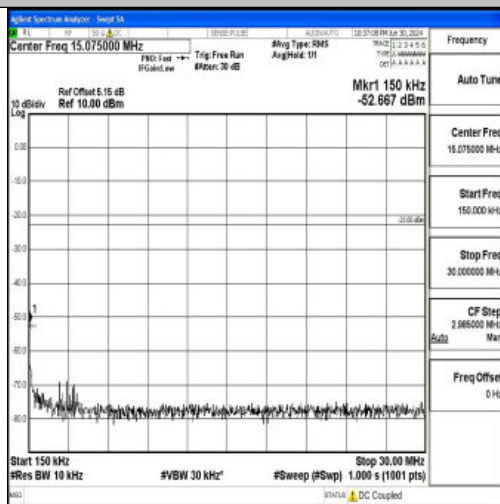
Band26_1.4MHz_16QAM_27033_1RB#0_0.15~30_0.15~30
