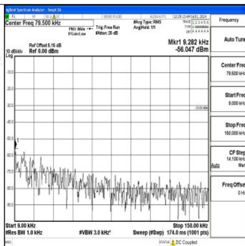
Band26_15MHz_16QAM_26915_1RB#0_0.009~0.15_0.009~0.15
