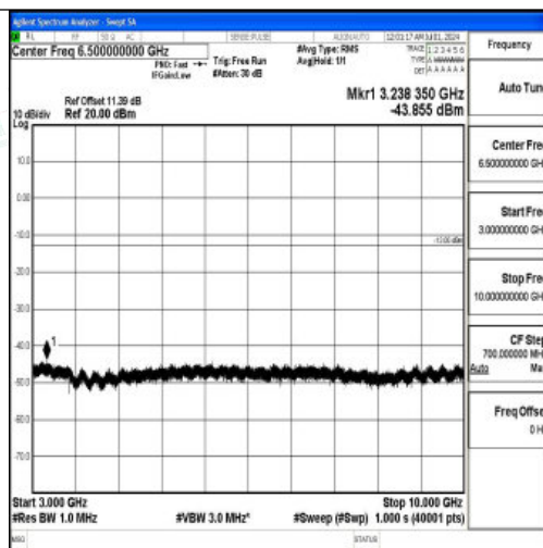
Band26_10MHz_16QAM_26840_1RB#0_3000~10000_3000~10000
