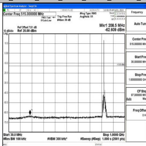
Band26_10MHz_QPSK_26840_1RB#0_30~1000_30~1000
