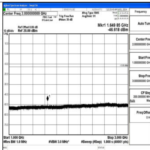
Band26_15MHz_QPSK_26865_1RB#0_1000~3000_1000~3000
