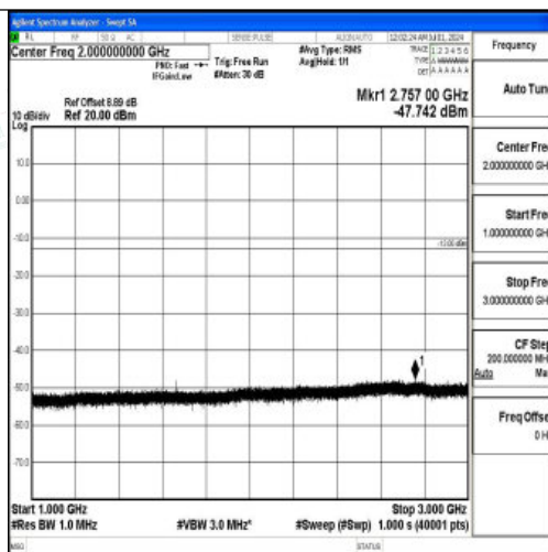
Band26_10MHz_16QAM_26915_1RB#0_1000~3000_1000~3000
