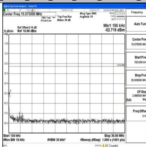
Band26_15MHz_QPSK_26915_1RB#0_0.15~30_0.15~30
