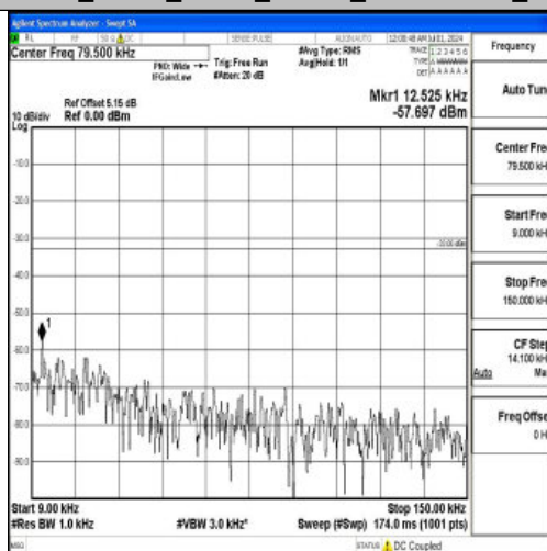
Band26_10MHz_16QAM_26840_1RB#0_0.009~0.15_0.009~0.15
