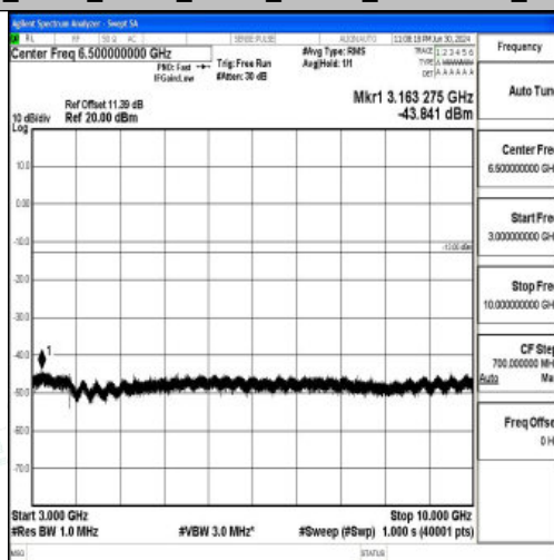
Band26_3MHz_QPSK_26805_1RB#0_3000~10000_3000~10000
