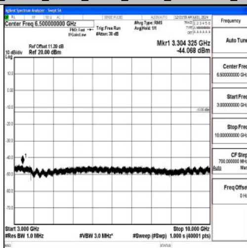
Band26_10MHz_QPSK_26915_1RB#0_3000~10000_3000~10000
