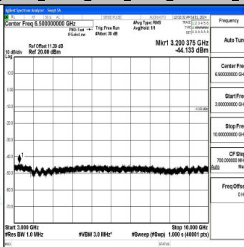
Band26_10MHz_16QAM_26915_1RB#0_3000~10000_3000~10000
