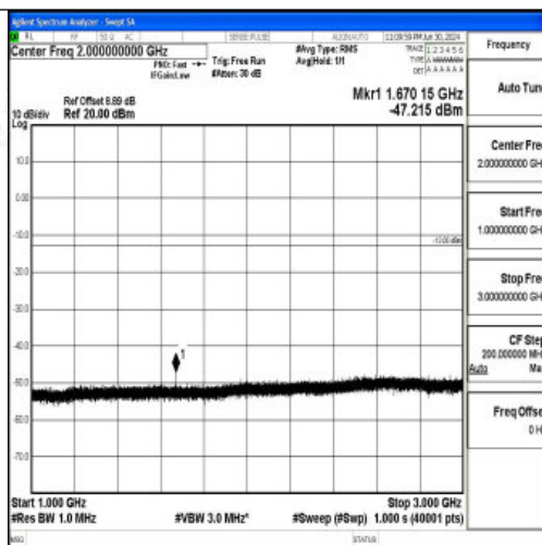
Band26_3MHz_16QAM_26915_1RB#0_1000~3000_1000~3000
