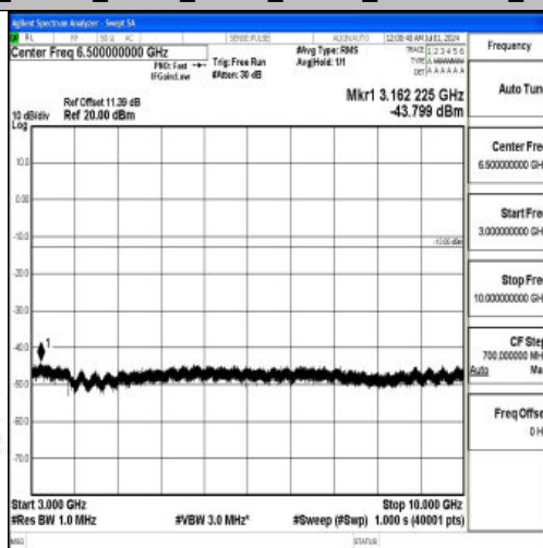
Band26_10MHz_QPSK_26840_1RB#0_3000~10000_3000~10000
