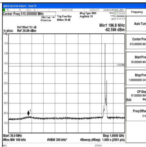
Band26_15MHz_16QAM_26965_1RB#0_30~1000_30~1000
