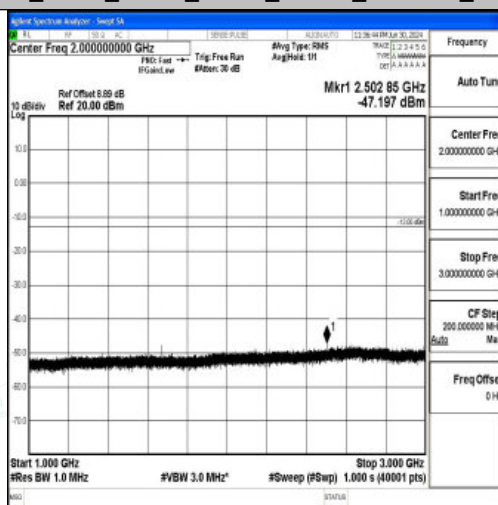
Band26_5MHz_QPSK_26915_1RB#0_1000~3000_1000~3000
