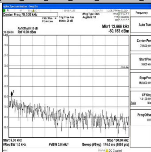
Band26_3MHz_16QAM_26805_1RB#0_0.009~0.15_0.009~0.15
