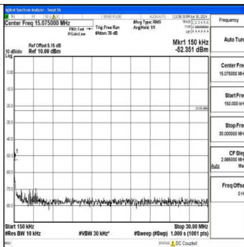
Band26_3MHz_16QAM_26805_1RB#0_0.15~30_0.15~30
