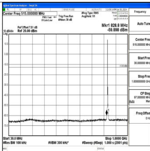
Band26_3MHz_QPSK_26915_1RB#0_30~1000_30~1000
