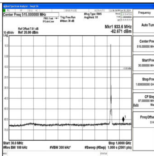
Band26_5MHz_QPSK_26915_1RB#0_30~1000_30~1000
