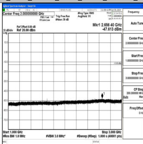
Band26_5MHz_16QAM_27015_1RB#0_1000~3000_1000~3000
