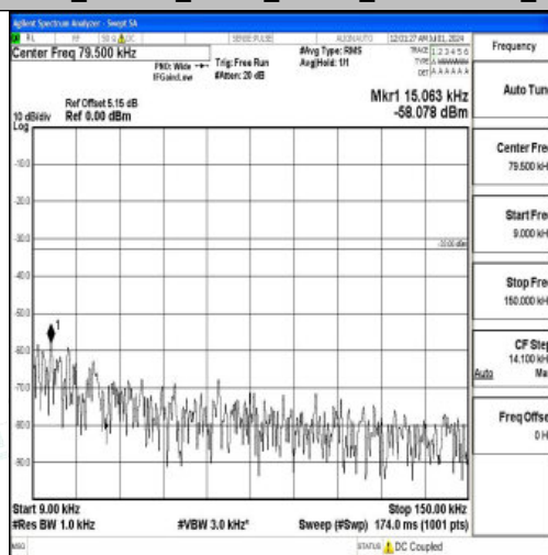
Band26_10MHz_QPSK_26915_1RB#0_0.009~0.15_0.009~0.15
