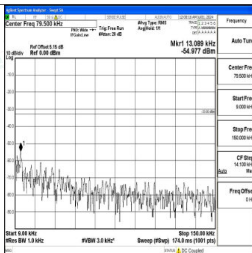
Band26_10MHz_QPSK_26840_1RB#0_0.009~0.15_0.009~0.15
