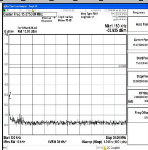
Band26_5MHz_16QAM_26915_1RB#0_0.15~30_0.15~30
