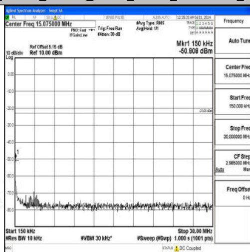
Band26_15MHz_16QAM_26915_1RB#0_0.15~30_0.15~30
