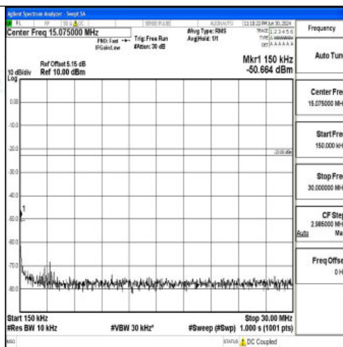
Band26_3MHz_QPSK_27025_1RB#0_0.15~30_0.15~30
