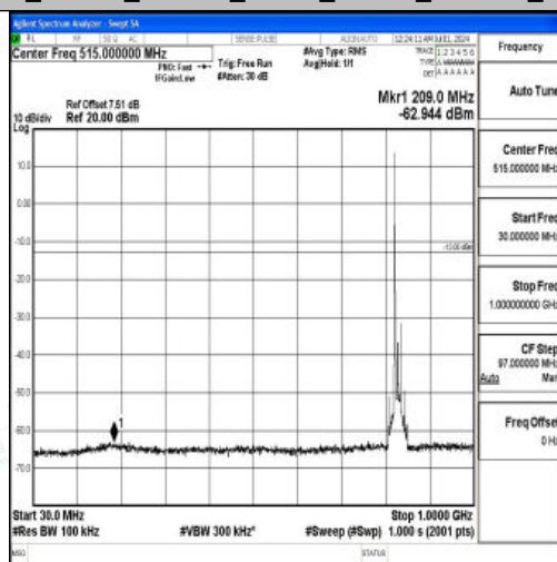
Band26_15MHz_16QAM_26865_1RB#0_30~1000_30~1000
