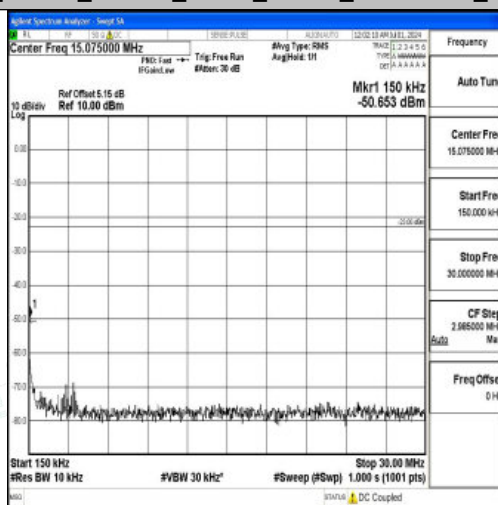
Band26_10MHz_16QAM_26915_1RB#0_0.15~30_0.15~30
