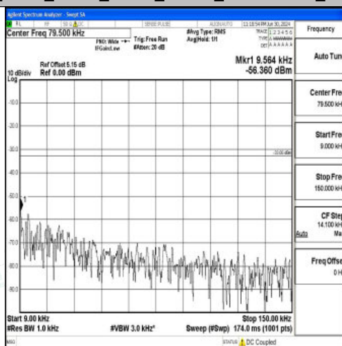
Band26_3MHz_16QAM_27025_1RB#0_0.009~0.15_0.009~0.15
