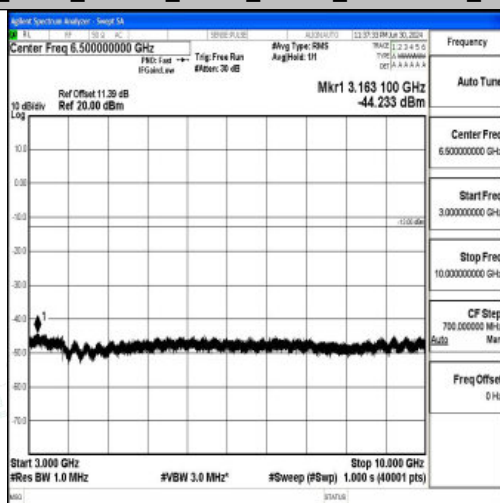
Band26_5MHz_16QAM_26915_1RB#0_3000~10000_3000~10000
