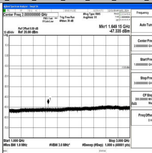
Band26_10MHz_16QAM_26840_1RB#0_1000~3000_1000~3000
