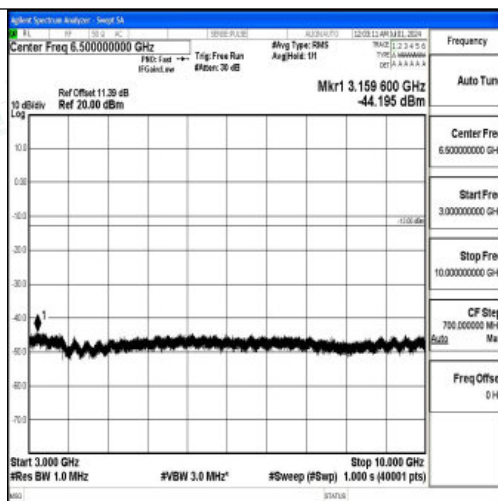
Band26_10MHz_QPSK_26990_1RB#0_3000~10000_3000~10000
