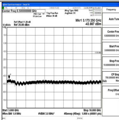
Band26_3MHz_QPSK_26915_1RB#0_3000~10000_3000~10000
