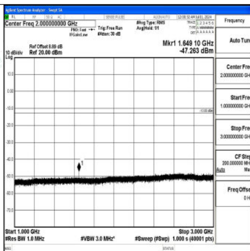
Band26_10MHz_QPSK_26840_1RB#0_1000~3000_1000~3000
