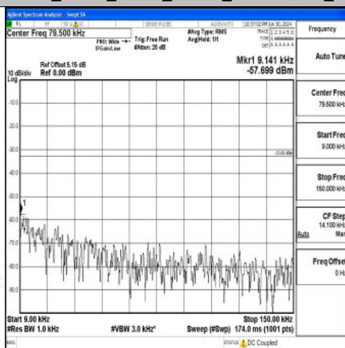
Band26_1.4MHz_16QAM_27033_1RB#0_0.009~0.15_0.009~0.15
