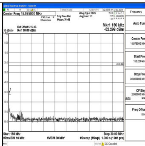
Band26_15MHz_QPSK_26965_1RB#0_0.15~30_0.15~30
