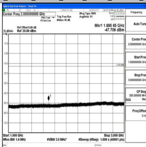
Band26_1.4MHz_16QAM_27033_1RB#0_1000~3000_1000~3000
