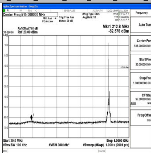
Band26_10MHz_16QAM_26915_1RB#0_30~1000_30~1000
