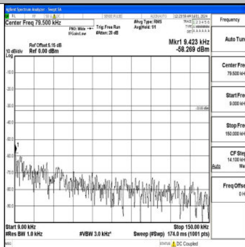
Band26_15MHz_16QAM_26865_1RB#0_0.009~0.15_0.009~0.15
