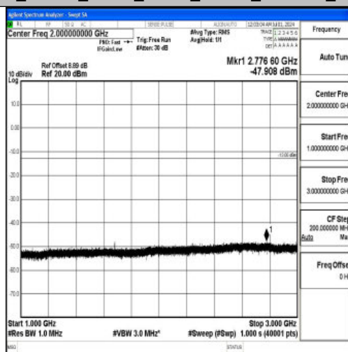
Band26_10MHz_QPSK_26990_1RB#0_1000~3000_1000~3000
