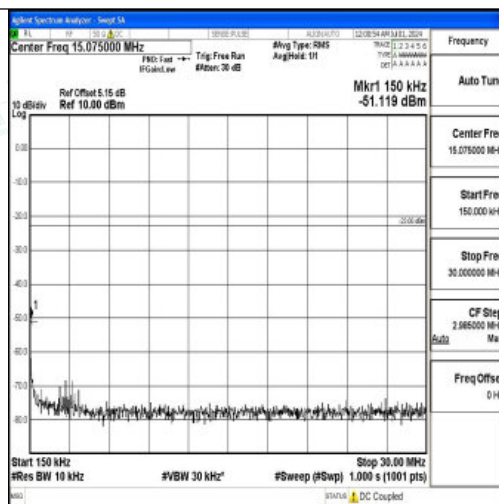
Band26_10MHz_16QAM_26840_1RB#0_0.15~30_0.15~30
