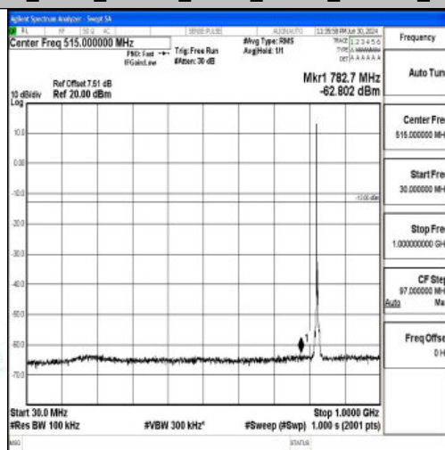
Band26_5MHz_16QAM_26815_1RB#0_30~1000_30~1000
