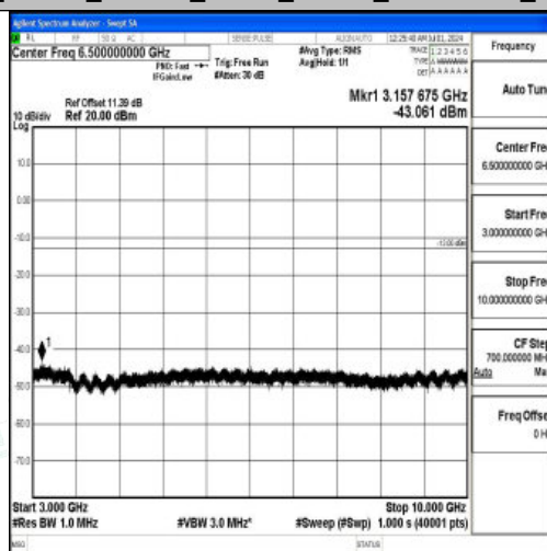
Band26_15MHz_16QAM_26915_1RB#0_3000~10000_3000~10000
