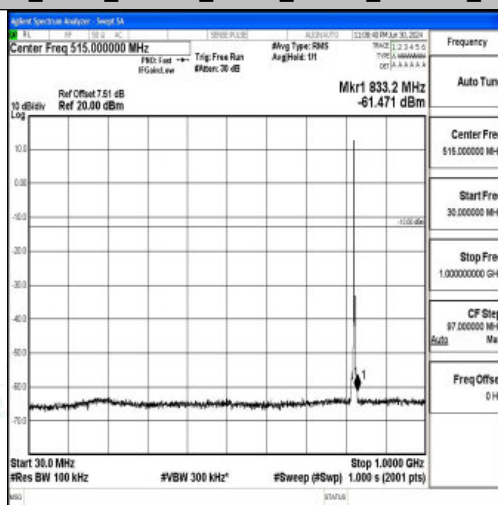
Band26_3MHz_16QAM_26805_1RB#0_30~1000_30~1000
