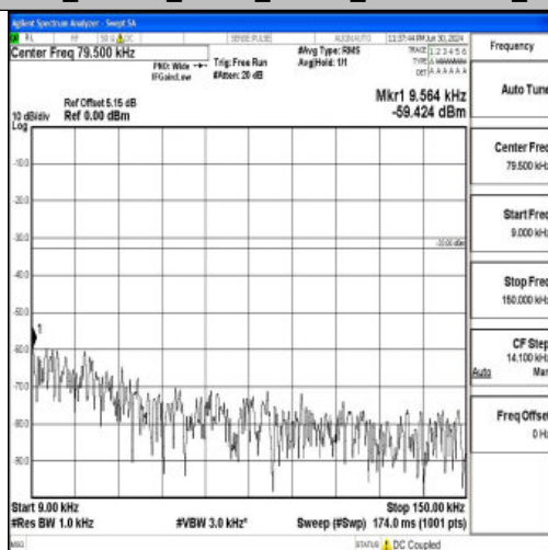
Band26_5MHz_QPSK_27015_1RB#0_0.009~0.15_0.009~0.15
