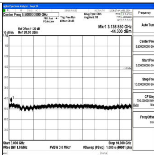
Band26_15MHz_QPSK_26965_1RB#0_3000~10000_3000~10000
