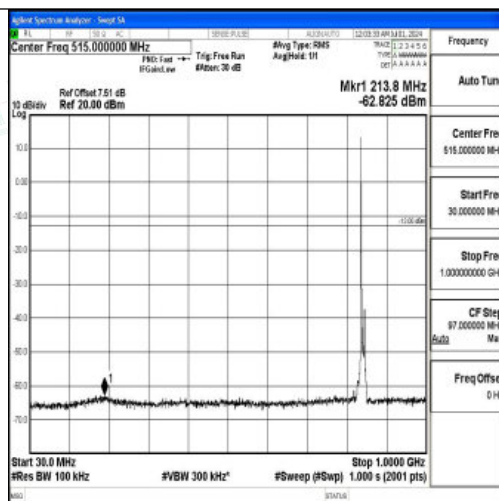
Band26_10MHz_16QAM_26990_1RB#0_30~1000_30~1000
