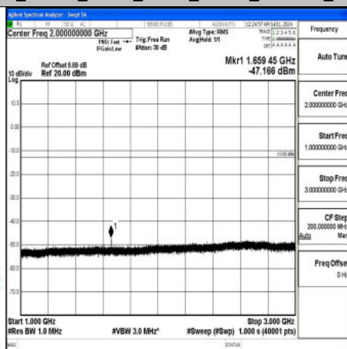
Band26_15MHz_QPSK_26915_1RB#0_1000~3000_1000~3000
