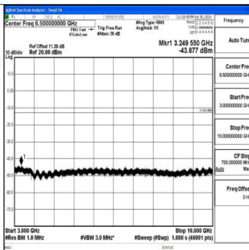
Band26_3MHz_QPSK_27025_1RB#0_3000~10000_3000~10000
