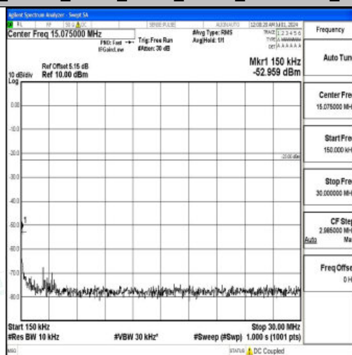
Band26_10MHz_QPSK_26840_1RB#0_0.15~30_0.15~30
