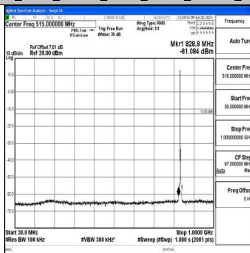
Band26_3MHz_16QAM_26915_1RB#0_30~1000_30~1000
