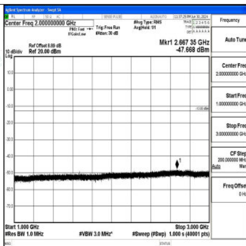
Band26_5MHz_16QAM_26915_1RB#0_1000~3000_1000~3000
