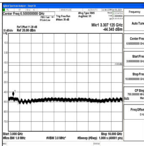
Band26_5MHz_16QAM_26815_1RB#0_3000~10000_3000~10000
