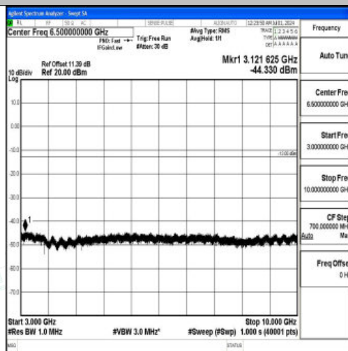
Band26_15MHz_QPSK_26865_1RB#0_3000~10000_3000~10000
