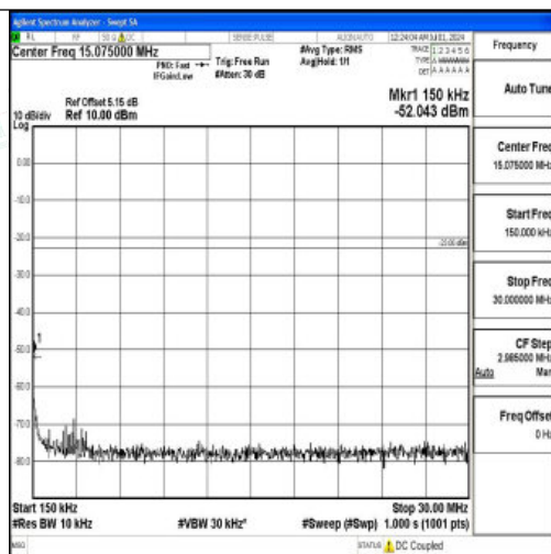
Band26_15MHz_16QAM_26865_1RB#0_0.15~30_0.15~30
