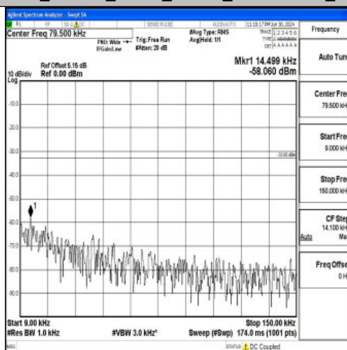
Band26_3MHz_QPSK_27025_1RB#0_0.009~0.15_0.009~0.15
