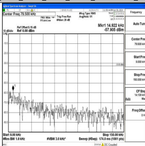
Band26_5MHz_16QAM_26815_1RB#0_0.009~0.15_0.009~0.15
