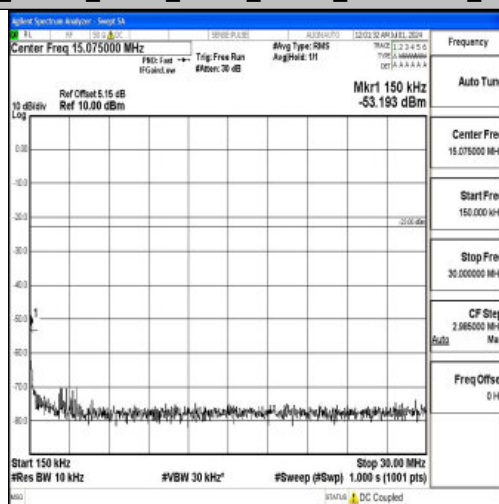
Band26_10MHz_QPSK_26915_1RB#0_0.15~30_0.15~30
