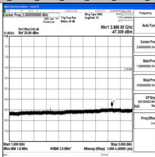
Band26_15MHz_QPSK_26965_1RB#0_1000~3000_1000~3000
