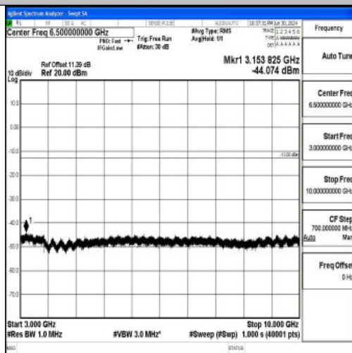
Band26_1.4MHz_16QAM_27033_1RB#0_3000~10000_3000~10000
