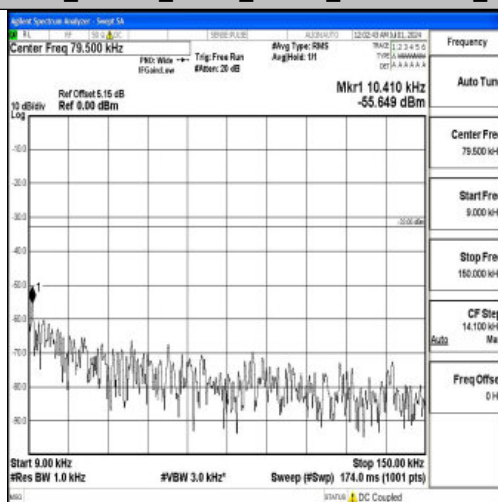
Band26_10MHz_QPSK_26990_1RB#0_0.009~0.15_0.009~0.15
