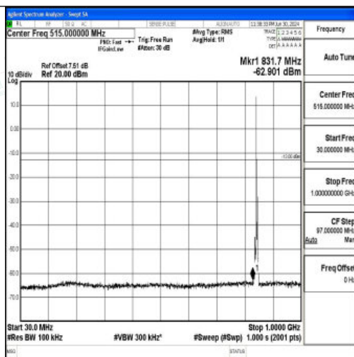
Band26_5MHz_16QAM_27015_1RB#0_30~1000_30~1000
