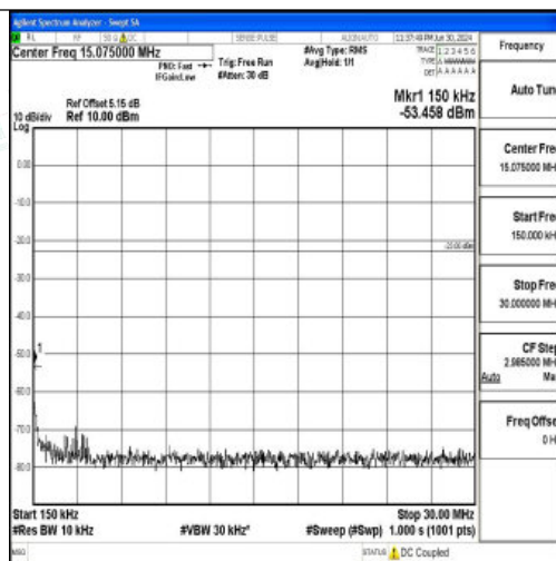
Band26_5MHz_QPSK_27015_1RB#0_0.15~30_0.15~30
