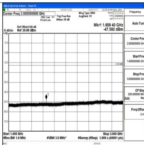
Band26_15MHz_16QAM_26915_1RB#0_1000~3000_1000~3000
