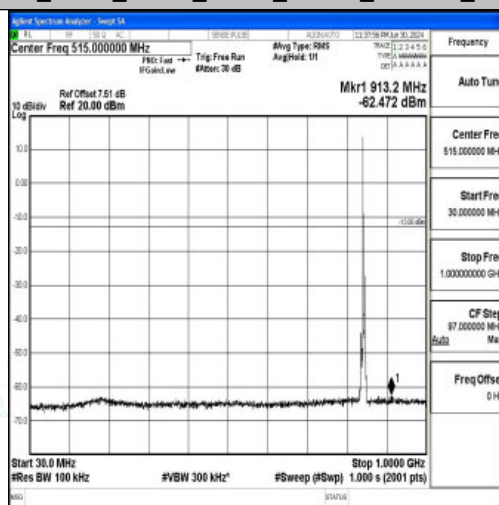
Band26_5MHz_QPSK_27015_1RB#0_30~1000_30~1000
