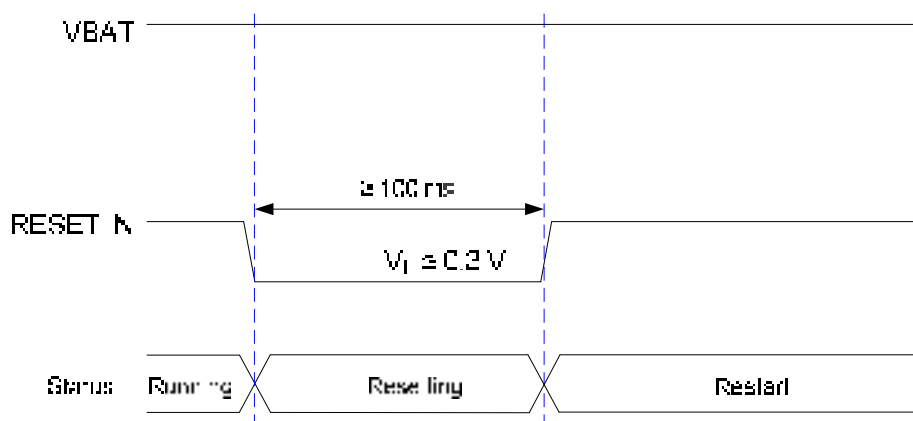
Figure 9: Reset Timing
