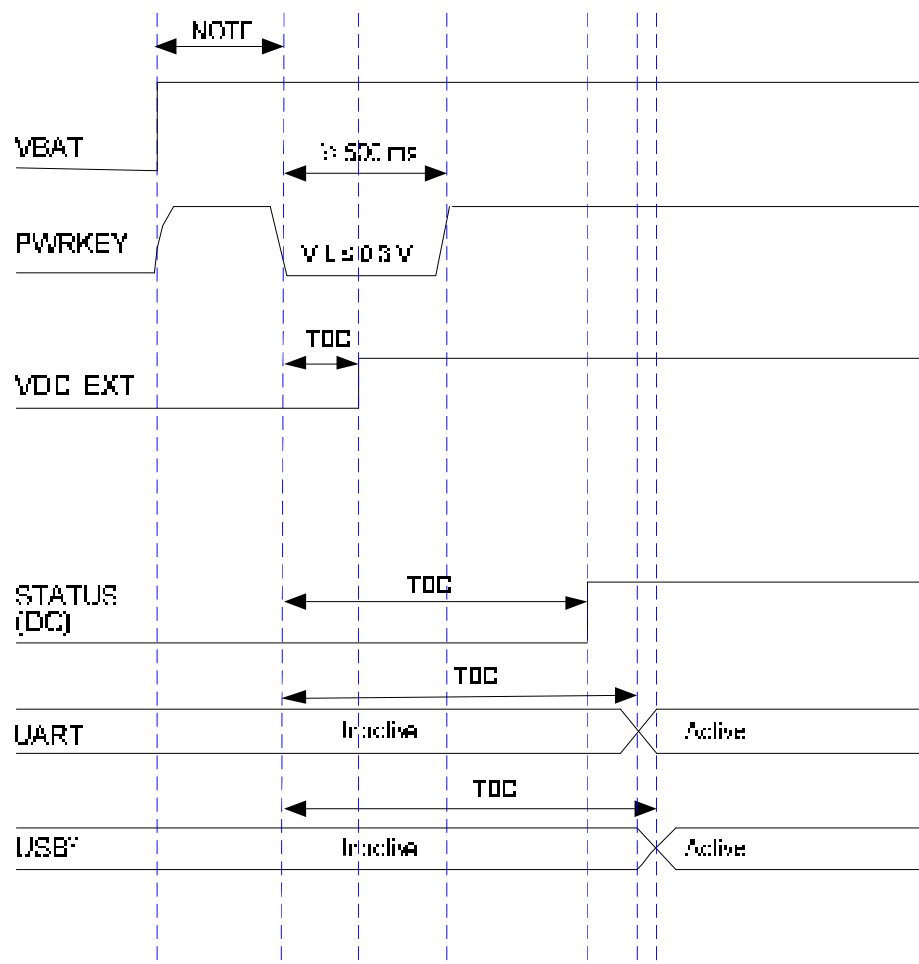
Figure 7: Power-up Timing
