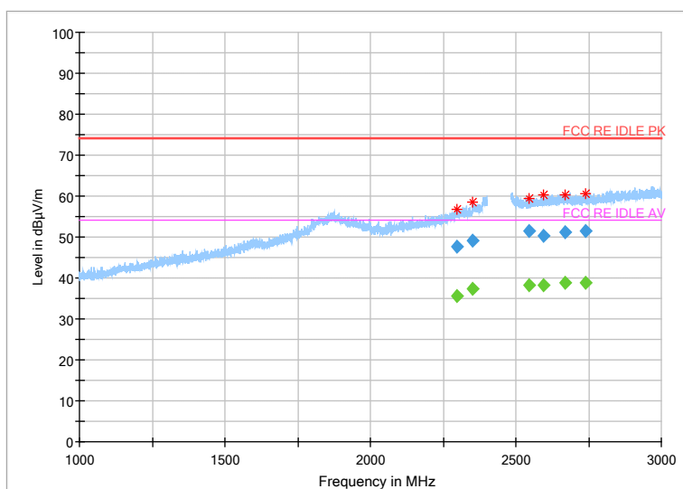
Fig.19 Radiated emission: Ch39, 1GHz~3GHz
