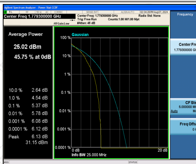
Band66-1.4MHz-QPSK-132665-1RB#0
