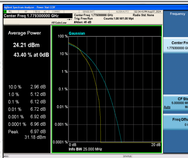
Band66-1.4MHz-16QAM-132665-1RB#0
