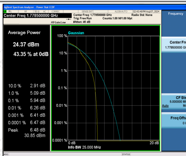
Band66-3MHz-16QAM-132657-1RB#0
