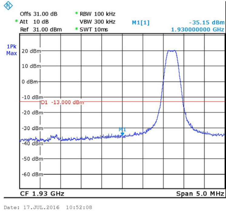
Figure 54. — GSM - 1931.2 MHz
