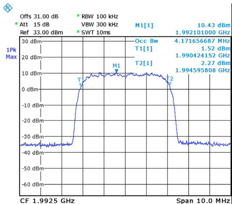
Figure 38. — W-CDMA - Input 1992.5 MHz
