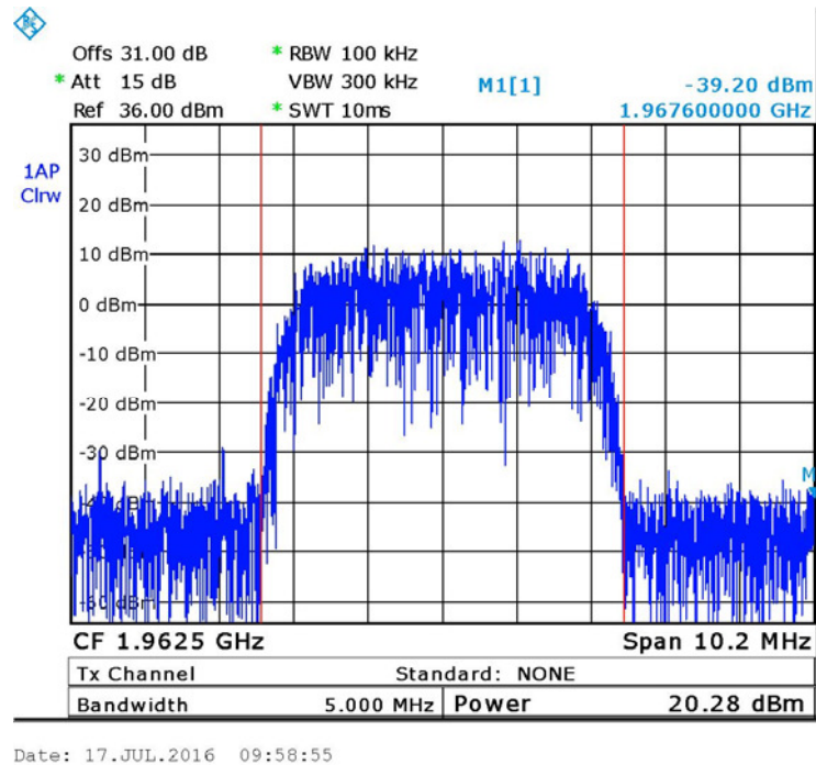
Figure 18. — W-CDMA - 1962.5 MHz
