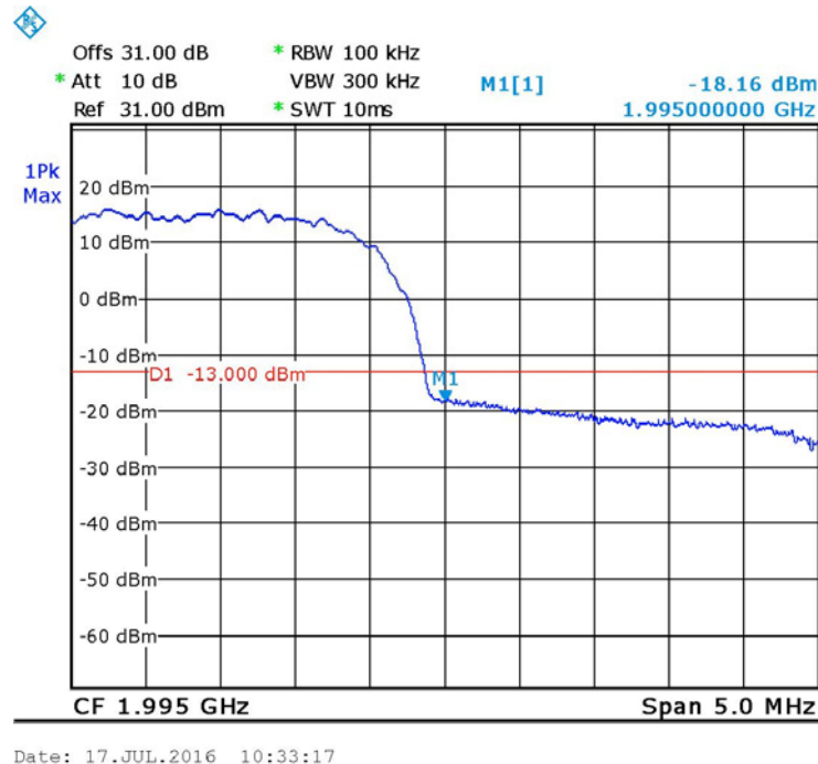
Figure 57. — W-CDMA - 1992.5 MHz
