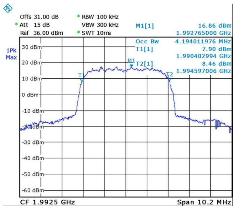
Figure 39. — W-CDMA - Output 1992.5 MHz
