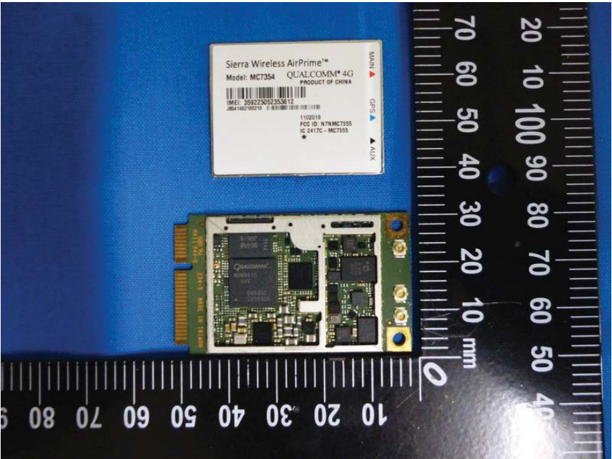
EUT –Subboard 8 Uncover View
