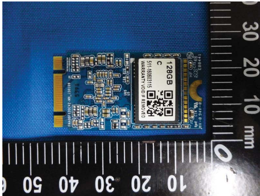
EUT –Subboard 5 Bottom View
