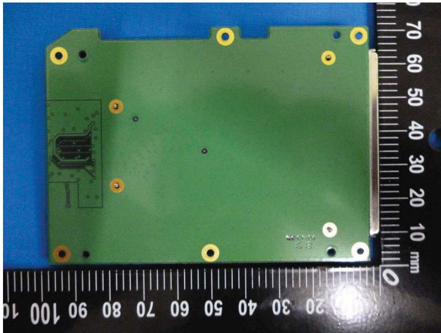
EUT –Subboard 4 Top View
