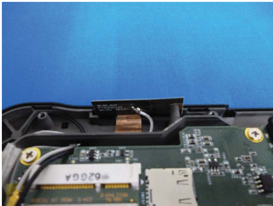
EUT –BT & Wlan Antenna 2 View
