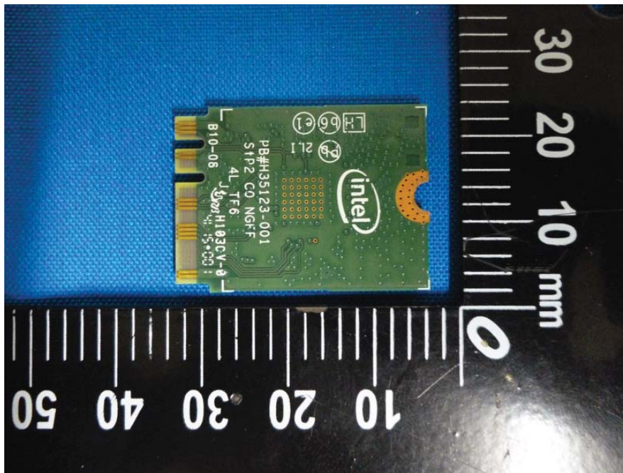
EUT –Subboard 7 Top View
