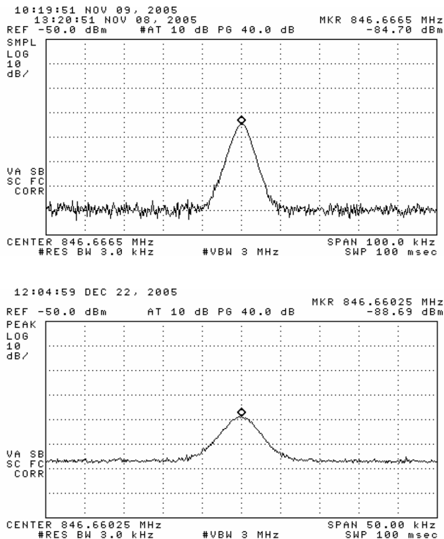
Figure 6.1. Receiver emissions: ECU-Y (top) and ECU-Z (bottom).
