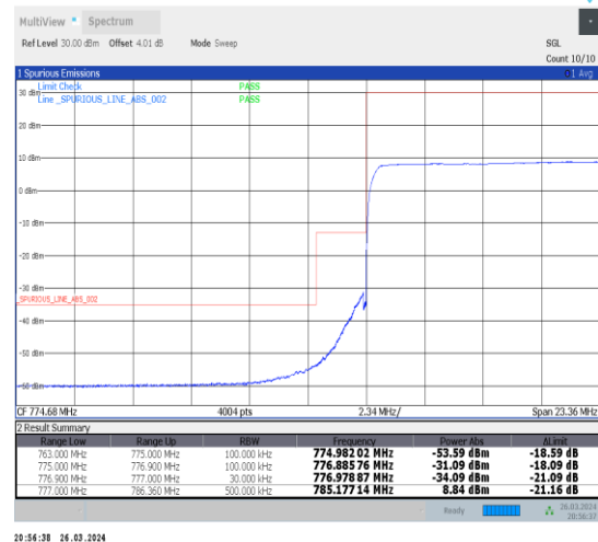
1-N13-15-10-L-6-CP-QPSK-Outer_Full-52@0-Ant1-1--PASS-see graph
