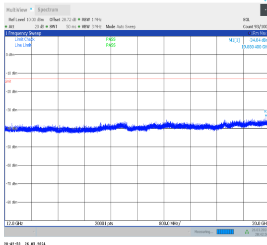
1-N13-15-10-L-1-DFT-PI2BPSK-Inner_1RB_Left-1@ 1-12000-20000-Ant1-19880.40--34.04--13-PASS
