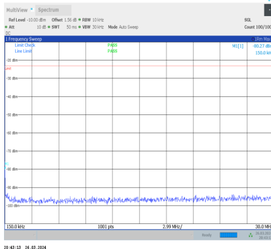
1-N13-15-10-M-1-DFT-PI2BPSK-Inner_1RB_Left-1@ 1-0.15-30-Ant1-0.15--80.27--23-PASS
