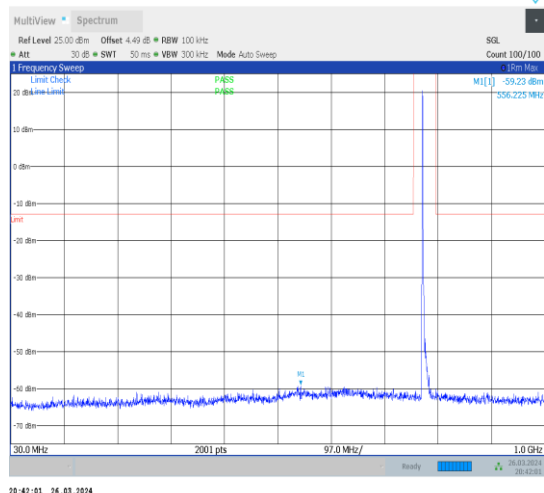
1-N13-15-10-L-1-DFT-PI2BPSK-Inner_1RB_Left-1@ 1-30-1000-Ant1-556.23--59.23--13-PASS
