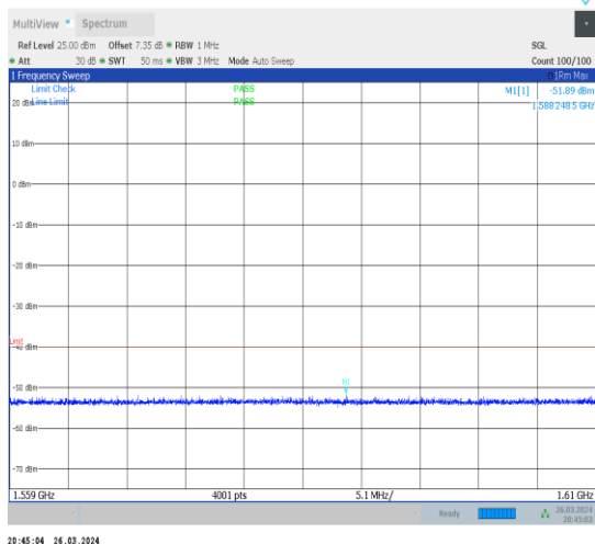
1-N13-15-10-H-1-DFT-PI2BPSK-Inner_1RB_Left-1 @1-1559-1610-Ant1-1588.25--51.89--40-PASS
