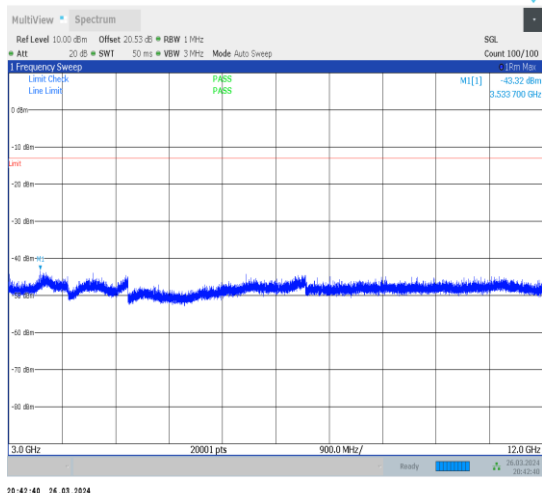
1-N13-15-10-L-1-DFT-PI2BPSK-Inner_1RB_Left-1@ 1-3000-12000-Ant1-3533.70--43.32--13-PASS
