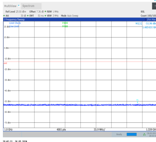
1-N13-15-10-L-1-DFT-PI2BPSK-Inner_1RB_Left-1@ 1-1000-1559-Ant1-1485.63--51.96--13-PASS
