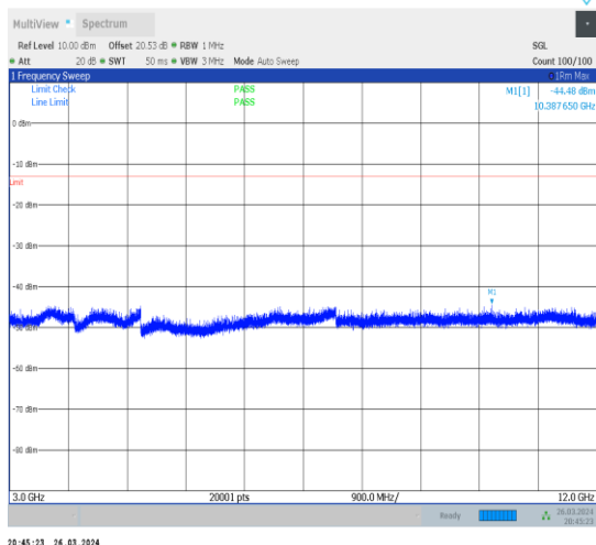
1-N13-15-10-H-1-DFT-PI2BPSK-Inner_1RB_Left-1 @1-3000-12000-Ant1-10387.65--44.48--13-PASS
