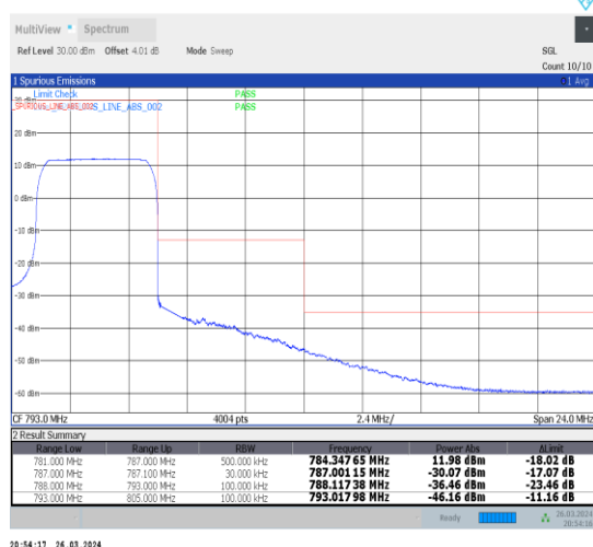
1-N13-15-5-H-6-CP-QPSK-Outer_Full-25@0-Ant1-1--PASS-see graph
