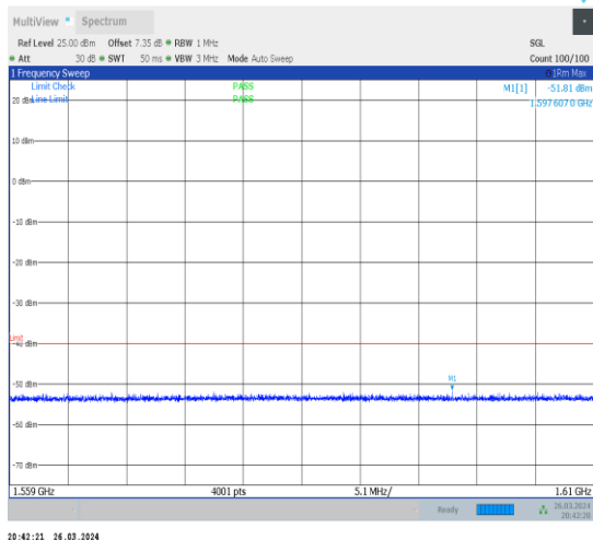
1-N13-15-10-L-1-DFT-PI2BPSK-Inner_1RB_Left-1@ 1-1559-1610-Ant1-1597.61--51.81--40-PASS
