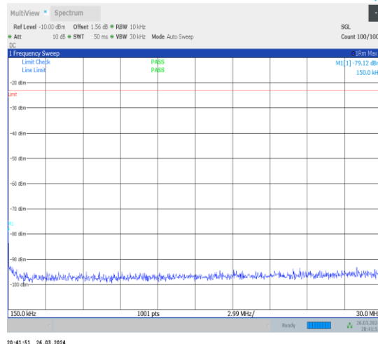
1-N13-15-10-L-1-DFT-PI2BPSK-Inner_1RB_Left-1@ 1-0.15-30-Ant1-0.15--79.12--23-PASS
