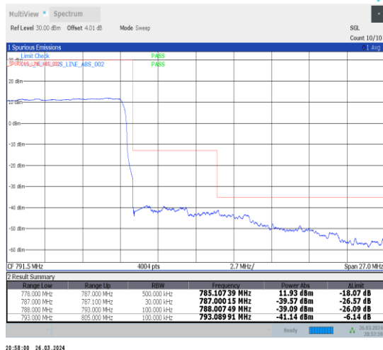
1-N13-15-10-H-3-DFT-PI2BPSK-Outer_Full-50@0-Ant1-1--PASS-see graph
