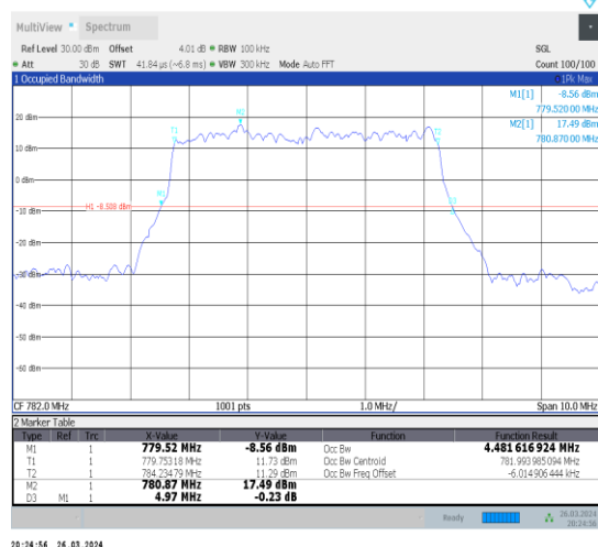
1-N13-15-5-M-2-DFT-PI2BPSK-Outer_Full-25@0-An t1-4.482-4.970-≤5-PASS
