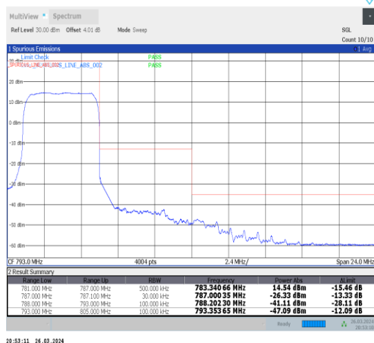
1-N13-15-5-H-3-DFT-PI2BPSK-Outer_Full-25@0-Ant1-1--PASS-see graph
