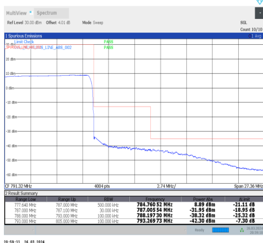
1-N13-15-10-H-6-CP-QPSK-Outer_Full-52@0-Ant1-1--PASS-see graph
