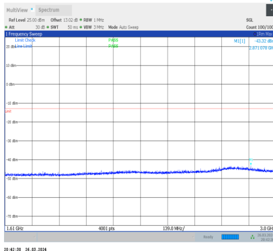
1-N13-15-10-L-1-DFT-PI2BPSK-Inner_1RB_Left-1@ 1-1610-3000-Ant1-2871.08--43.32--13-PASS
