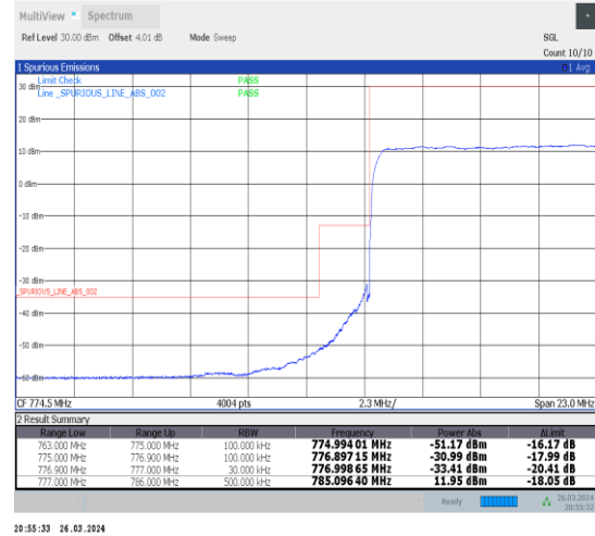
1-N13-15-10-L-3-DFT-PI2BPSK-Outer_Full-50@0-Ant1-1--PASS-see graph
