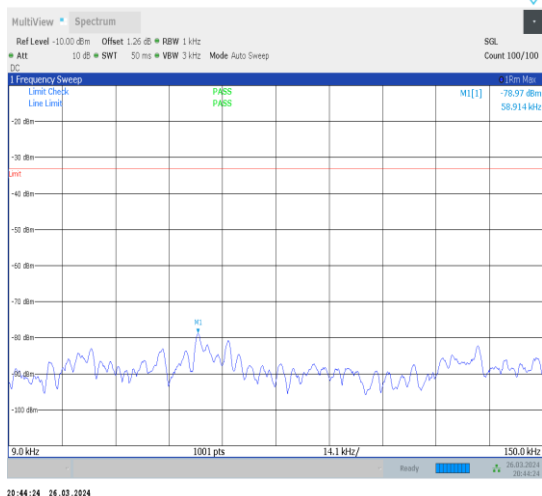
1-N13-15-10-H-1-DFT-PI2BPSK-Inner_1RB_Left-1 @1-0.009-0.15-Ant1-0.06--78.97--33-PASS
