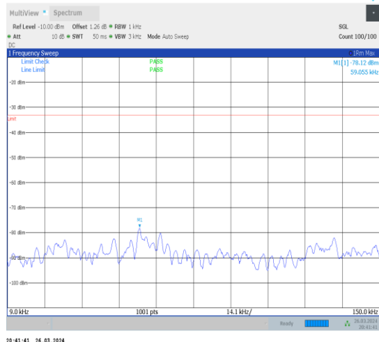
1-N13-15-10-L-1-DFT-PI2BPSK-Inner_1RB_Left-1@ 1-0.009-0.15-Ant1-0.06--78.12--33-PASS
