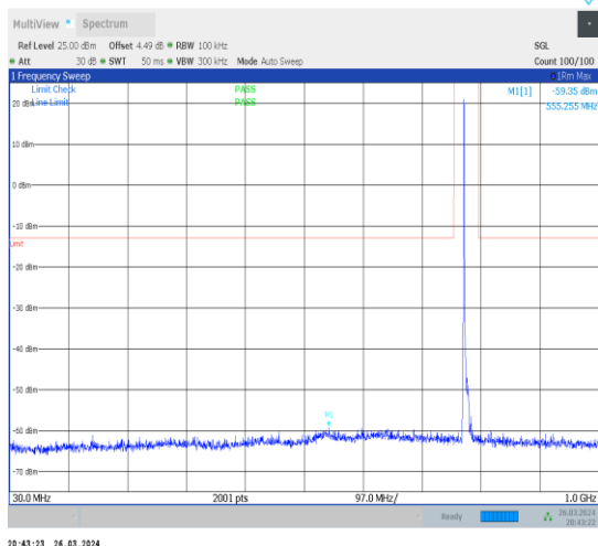
1-N13-15-10-M-1-DFT-PI2BPSK-Inner_1RB_Left-1 @1-30-1000-Ant1-555.26--59.35--13-PASS
