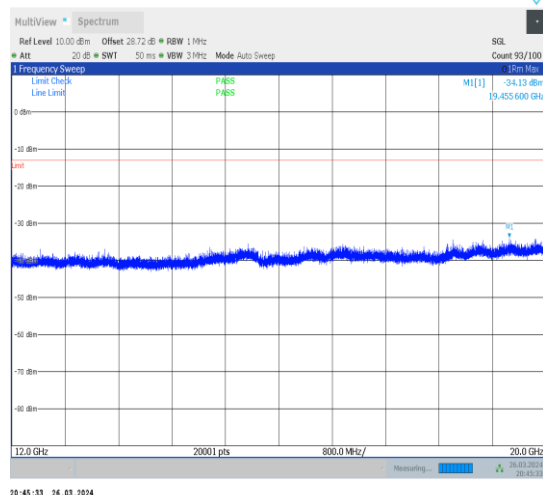
1-N13-15-10-H-1-DFT-PI2BPSK-Inner_1RB_Left-1@ 1-12000-20000-Ant1-19455.60--34.13--13-PASS
