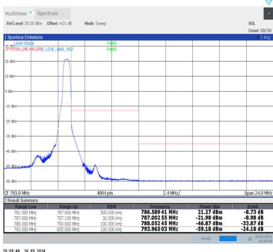
1-N13-15-10-H-5-CP-QPSK-Edge_1RB_Right-1@51-Ant1-1--PASS-see graph
