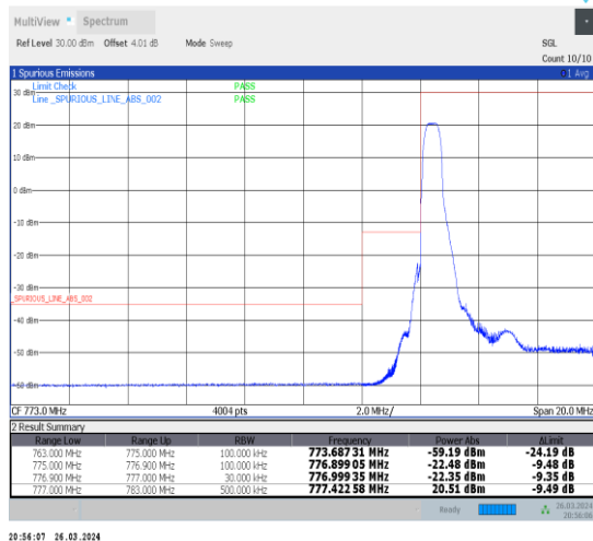
1-N13-15-10-L-4-CP-QPSK-Edge_1RB_Left-1@0-Ant1-1--PASS-see graph
