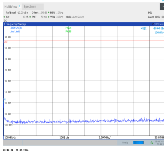
1-N13-15-10-H-1-DFT-PI2BPSK-Inner_1RB_Left-1@ 1-0.15-30-Ant1-0.15--80.04--23-PASS
