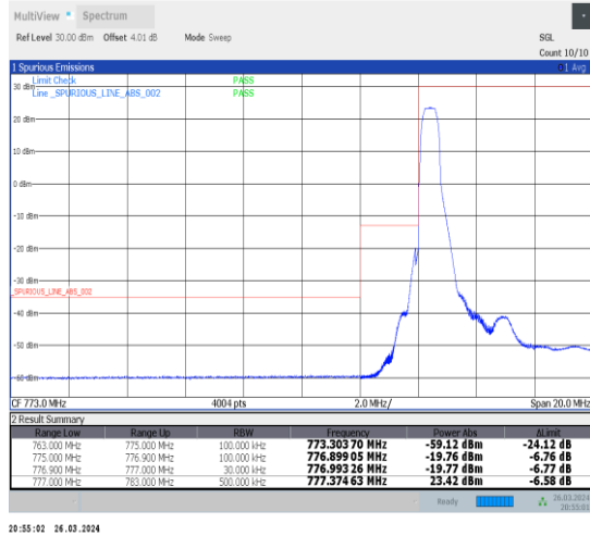
1-N13-15-10-L-1-DFT-PI2BPSK-Edge_1RB_Left-1@0-Ant1-1--PASS-see graph
