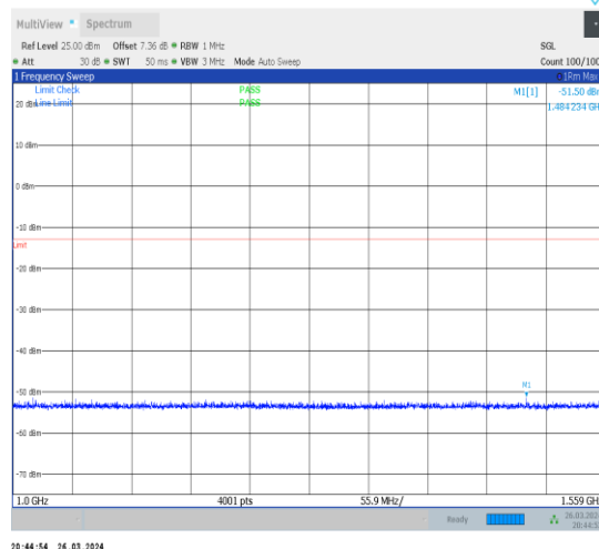
1-N13-15-10-H-1-DFT-PI2BPSK-Inner_1RB_Left-1@ 1-1000-1559-Ant1-1484.23--51.50--13-PASS
