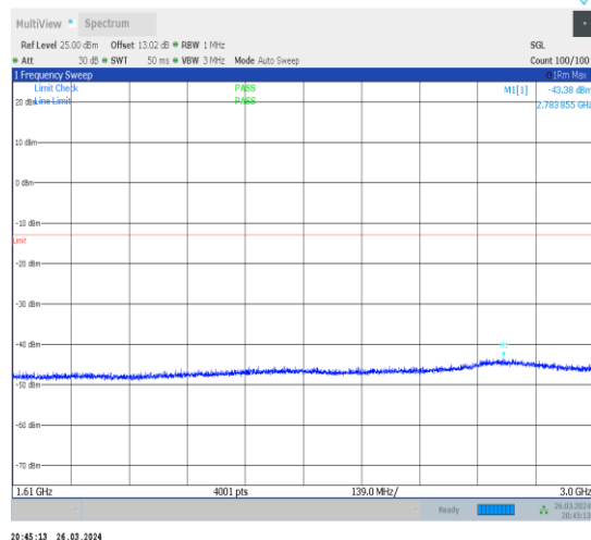
1-N13-15-10-H-1-DFT-PI2BPSK-Inner_1RB_Left-1@ 1-1610-3000-Ant1-2783.86--43.38--13-PASS
