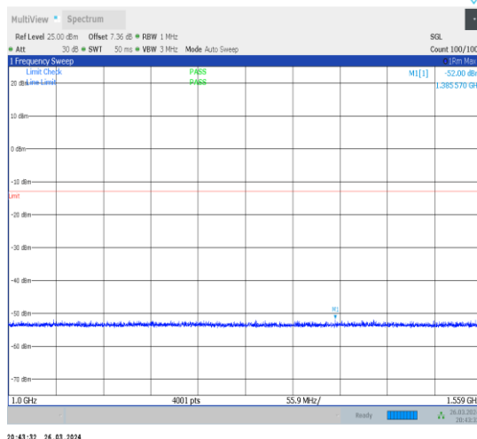
1-N13-15-10-M-1-DFT-PI2BPSK-Inner_1RB_Left-1@ 1-1000-1559-Ant1-1385.57--52.00--13-PASS
