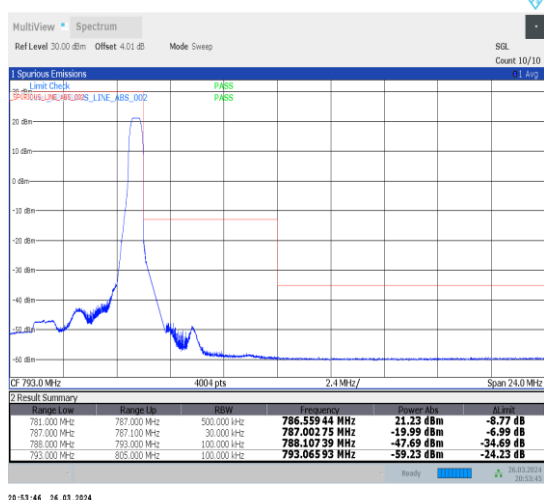
1-N13-15-5-H-5-CP-QPSK-Edge_1RB_Right-1@24-Ant1-1--PASS-see graph
