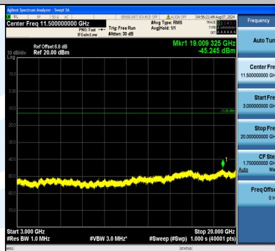
Band4_5MHz_QPSK_20175_25RB#0_3000~20000_3000~20000
