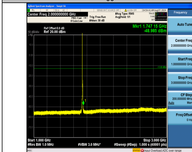
Band4_5MHz_QPSK_20175_1RB#0_1000~3000_1000~3000
