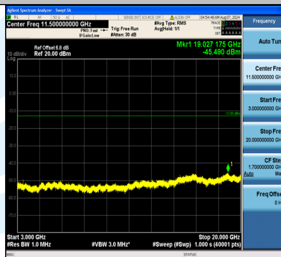
Band4_5MHz_QPSK_20175_1RB#0_3000~20000_3000~20000
