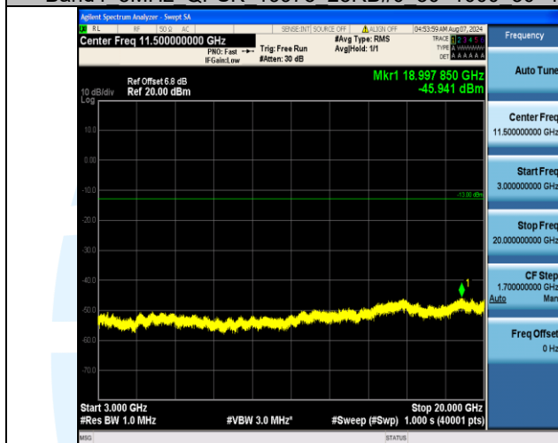
Band4_5MHz_QPSK_19975_25RB#0_3000~20000_3000~20000
