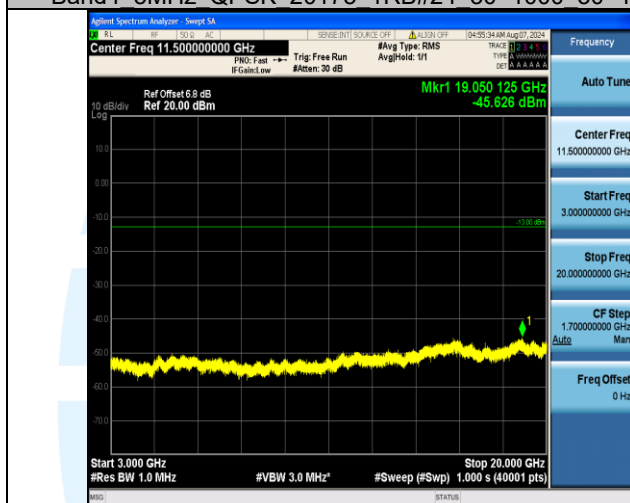
Band4_5MHz_QPSK_20175_1RB#24_3000~20000_3000~20000
