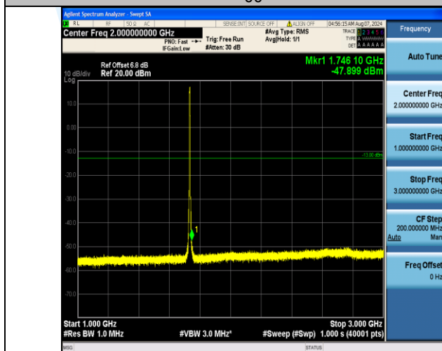
Band4_5MHz_QPSK_20175_25RB#0_1000~3000_1000~3000
