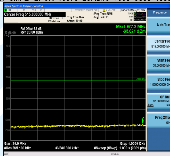
Band4_5MHz_QPSK_20175_1RB#0_30~1000_30~1000
