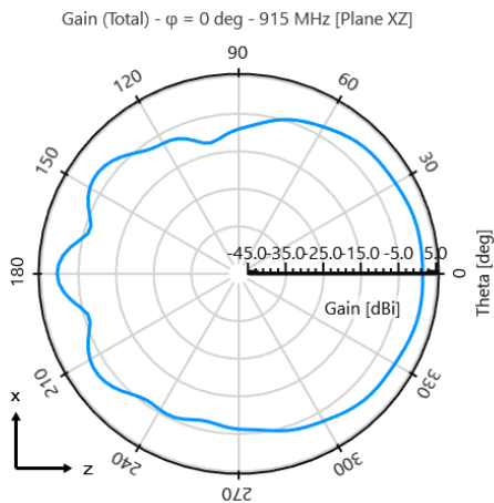
Phi = 0° Plane
