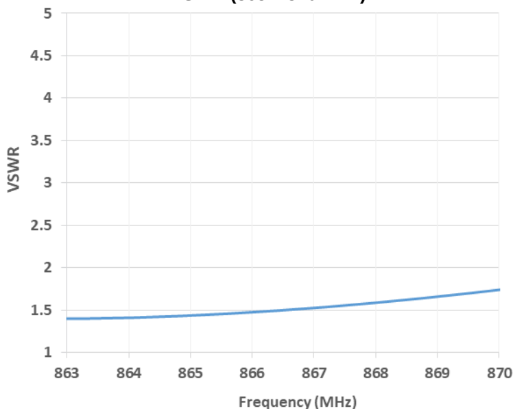
VSWR (863 – 870 MHz)
