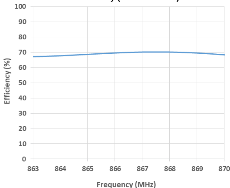
Efficiency (863 – 870 MHz)
