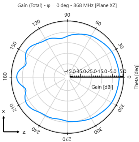
Phi = 0° Plane
