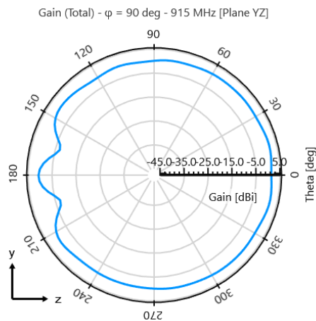
Phi = 90° Plane
