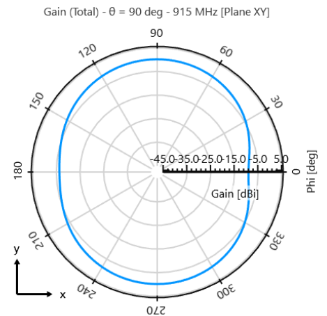
Theta = 90° Plane
