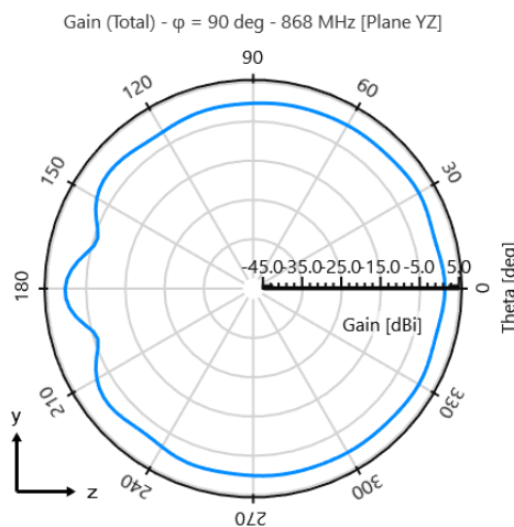
Phi = 90° Plane
