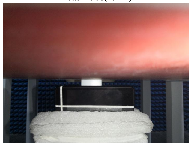
Right side(10mm)
