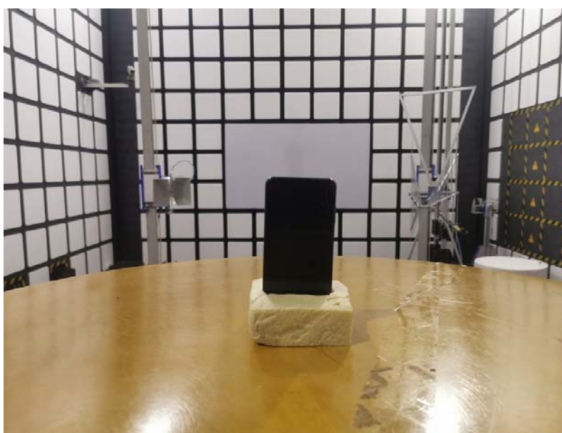
Spurious Radiated Emissions Test setup
