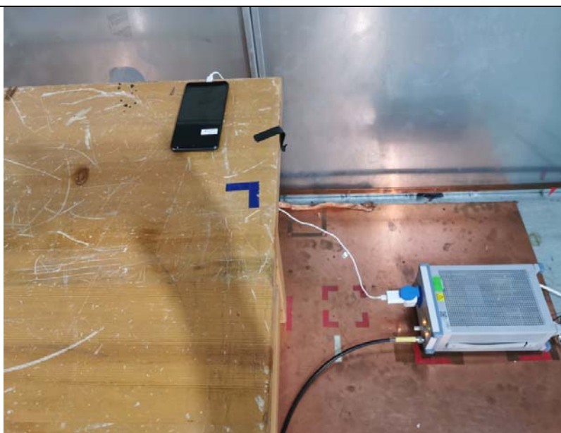
Conducted Emissions Test Setup (with charger)
