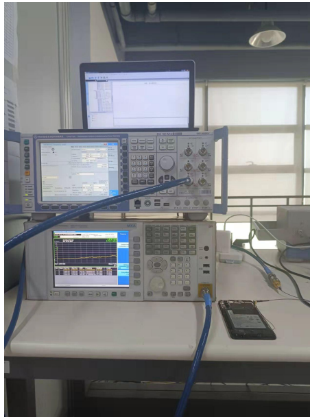
'RF Conducted Test setup (GSM/WCDMA/LTE)
