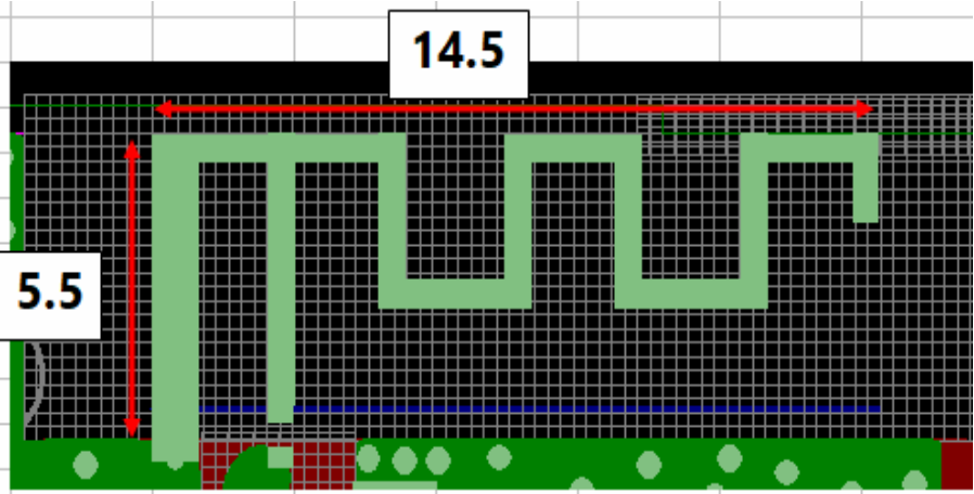
EL52203 BS BT Antenna Dimensions in mm
