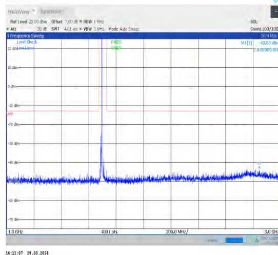
1-N70-15-15-L-1-DFT-PI2BPSK-Inner_1RB_Left-1@ 1-1000-3000-Ant1-2845.00--43.53--13-PASS
