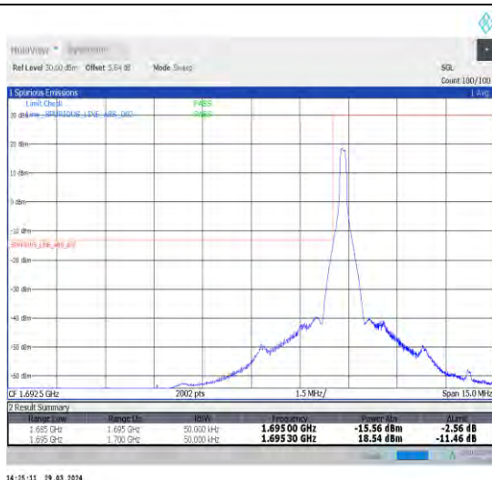
1-N70-15-5-L-1-DFT-PI2BPSK-Edge_1RB_Left-1@0-A nt1-1-seegraph-PASS-see graph
