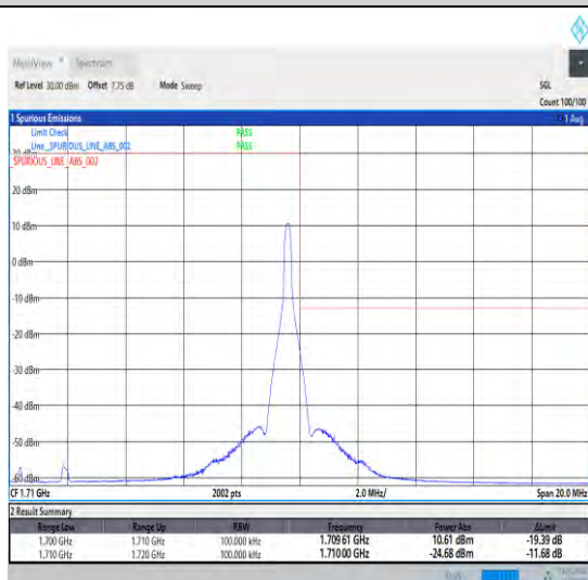
1-N70-15-10-H-5-CP-QPSK-Edge_1RB_Right-1@51-Ant1 1-1-seegraph-PASS-see graph
