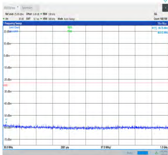
1-N70-15-15-L-1-DFT-PI2BPSK-Inner_1RB_Left-1@ 1-30-1000-Ant1-48.92--56.75--23-PASS
