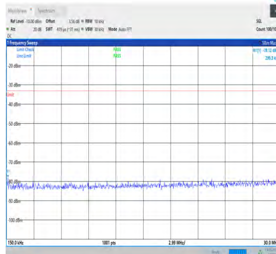
1-N70-15-15-L-1-DFT-PI2BPSK-Inner_1RB_Left-1@ 1-0.15-30-Ant1-0.30--78.12--33-PASS
