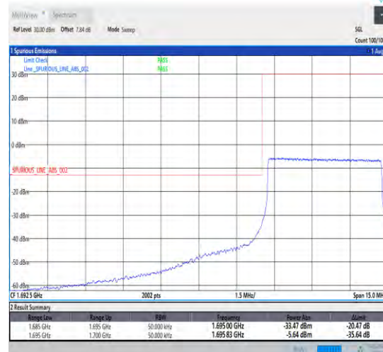
1-N70-15-5-L-6-CP-QPSK-Outer_Full-25@0-Ant1- 1-seegraph-PASS-see graph
