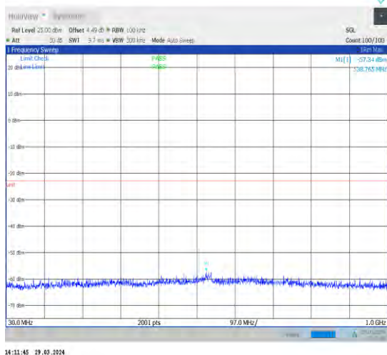
1-N70-15-15-L-1-DFT-PI2BPSK-Inner_1RB_Left-1@ 1-30-1000-Ant1-538.77--57.34--23-PASS
