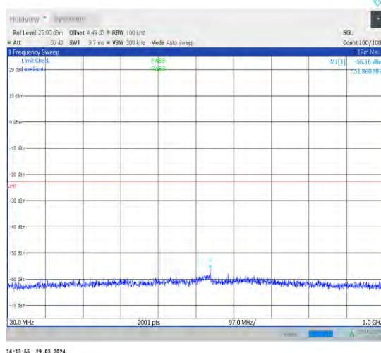
1-N70-15-15-M-1-DFT-PI2BPSK-Inner_1RB_Left-1@ 1-30-1000-Ant1-551.86--56.16--23-PASS
