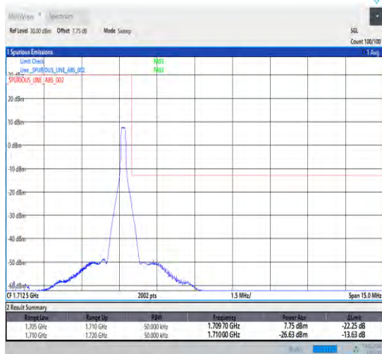
1-N70-15-5-H-5-CP-QPSK-Edge_1RB_Right-1@24-An t1-1-seegraph-PASS-see graph
