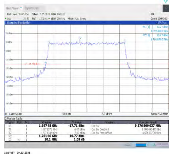
1-N70-15-10-M-7-CP-16QAM-Outer_Full-52@0-Ant1 -9.277-10.100-≤10-PASS
