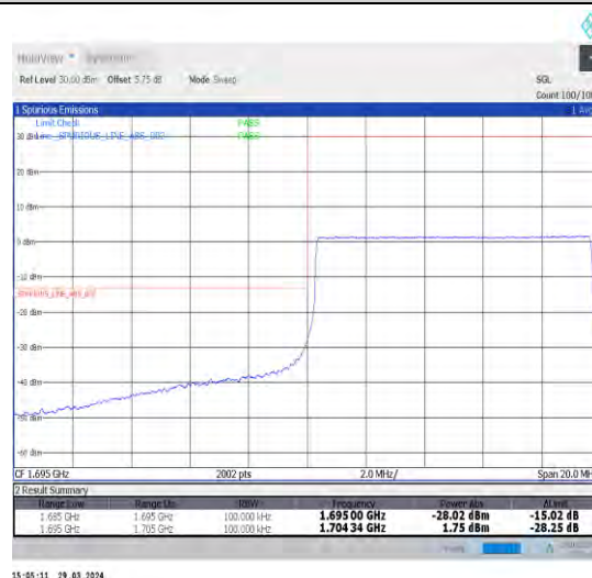
1-N70-15-10-L-6-CP-QPSK-Outer_Full-52@0-Ant1-1-seegraph-PASS-see graph
