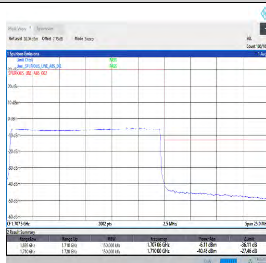
1-N70-15-15-H-6-CP-QPSK-Outer_Full-79@0-Ant1 1-1-seegraph-PASS-see graph
