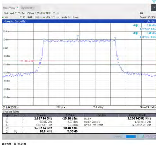
1-N70-15-10-M-6-CP-QPSK-Outer_Full-52@0-Ant1 9.287-10.000-≤10-PASS
