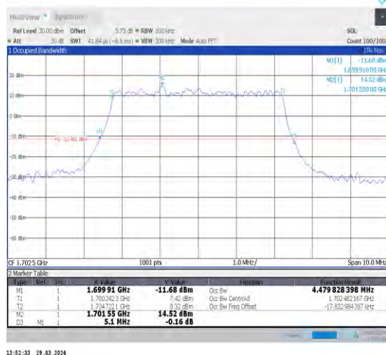
1-N70-15-5-M-6-CP-QPSK-Outer_Full-25@0-Ant1-4. 48-5.100-≤5-PASS
