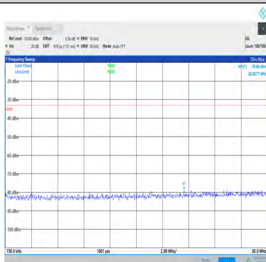
1-N70-15-15-H-1-DFT-PI2BPSK-Inner_1RB_Left-1@ 1-0.15-30-Ant1-20.51--78.64--33-PASS
