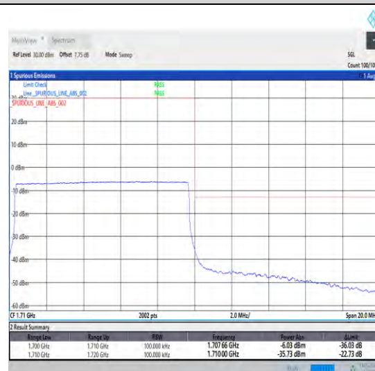
1-N70-15-10-H-6-CP-QPSK-Outer_Full-52@0-Ant1 1-1-seegraph-PASS-see graph
