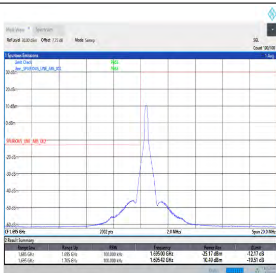
1-N70-15-10-L-4-CP-QPSK-Edge_1RB_Left-1@0-Ant1 -1-seegraph-PASS-see graph
