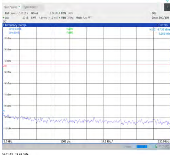
1-N70-15-15-L-1-DFT-PI2BPSK-Inner_1RB_Left-1@ 1-0.009-0.15-Ant1-0.01--87.59--43-PASS
