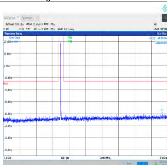
1-N70-15-15-H-1-DFT-PI2BPSK-Inner_1RB_Left-1@ 1-1000-3000-Ant1-2929.50--40.07--13-PASS
