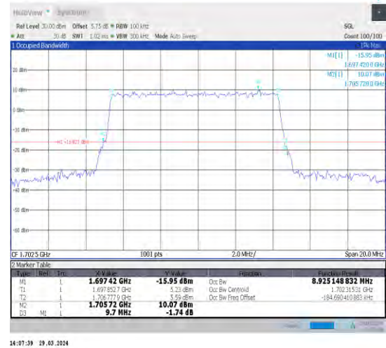
1-N70-15-10-M-5-DFT-256QAM-Outer_Full-50@0-A nt1-8.925-9.700-≤10-PASS
