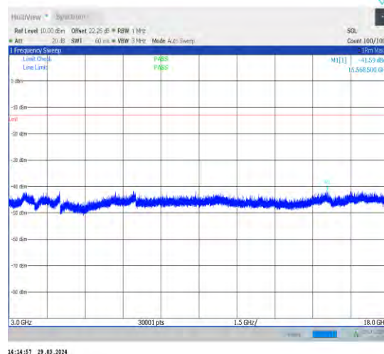
1-N70-15-15-M-1-DFT-PI2BPSK-Inner_1RB_Left-1@ 1-3000-18000-Ant1-15568.50--41.59--13-PASS
