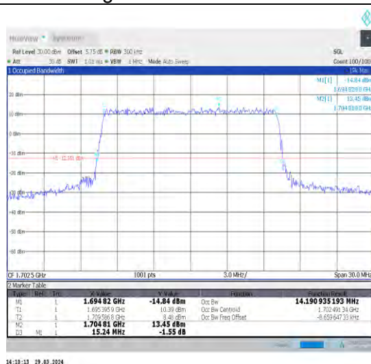
1-N70-15-15-M-8-CP-64QAM-Outer_Full-79@0-Ant1 -14.191-15.240≤15-PASS
