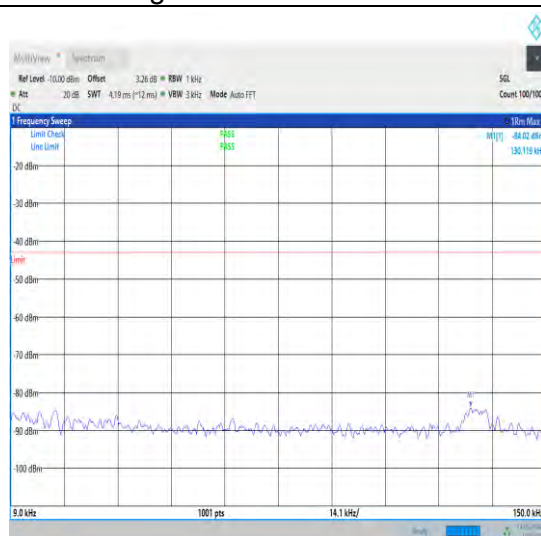
1-N70-15-15-M-1-DFT-PI2BPSK-Inner_1RB_Left-1 @1-0.009-0.15-Ant1-0.13--84.02--43-PASS
