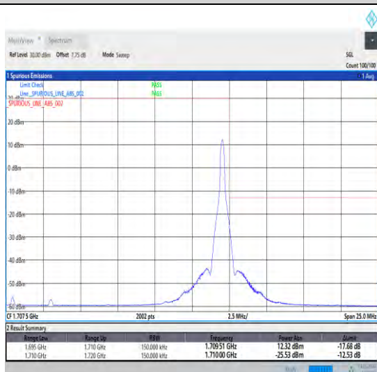
1-N70-15-15-H-5-CP-QPSK-Edge_1RB_Right-1@78-Ant1 1-1-seegraph-PASS-see graph
