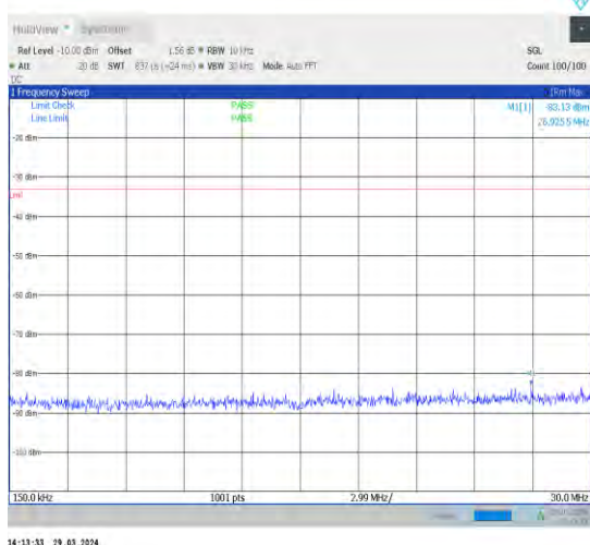
1-N70-15-15-M-1-DFT-PI2BPSK-Inner_1RB_Left-1 @1-0.15-30-Ant1-26.93--83.13--33-PASS
