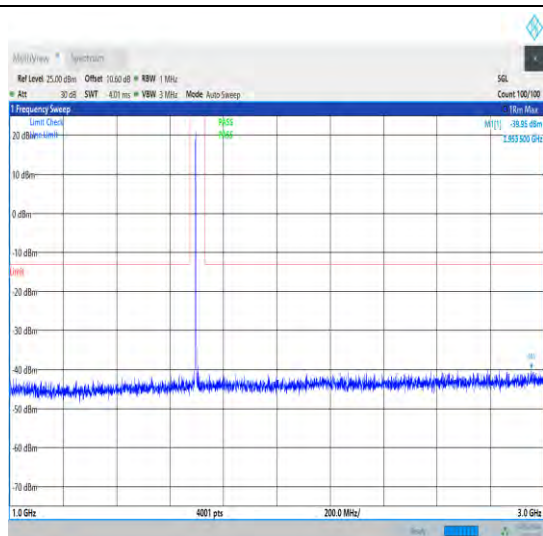
1-N70-15-15-M-1-DFT-PI2BPSK-Inner_1RB_Left-1 @1-1000-3000-Ant1-2953.50--39.95--13-PASS
