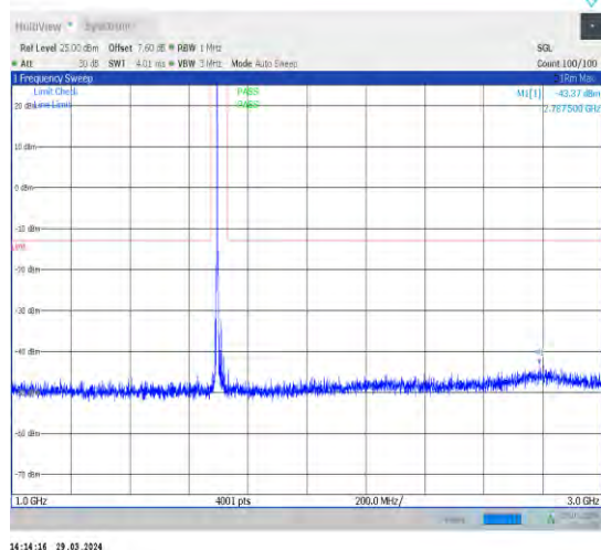
1-N70-15-15-M-1-DFT-PI2BPSK-Inner_1RB_Left-1 @1-1000-3000-Ant1-2787.50--43.37--13-PASS
