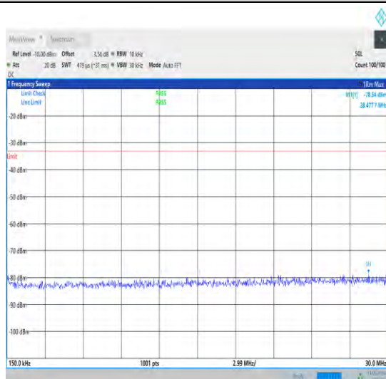
1-N70-15-15-M-1-DFT-PI2BPSK-Inner_1RB_Left-1 @1-0.15-30-Ant1-28.48--78.54--33-PASS
