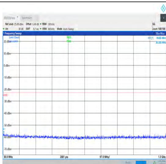
1-N70-15-15-H-1-DFT-PI2BPSK-Inner_1RB_Left-1@ 1-30-1000-Ant1-35.34--56.83--23-PASS
