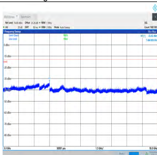
1-N70-15-15-M-1-DFT-PI2BPSK-Inner_1RB_Left-1 @1-3000-18000-Ant1-7484.00--32.92--13-PASS
