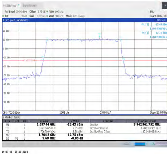
1-N70-15-10-M-4-DFT-64QAM-Outer_Full-50@0-Ant 1-8.943-9.680-≤10-PASS
