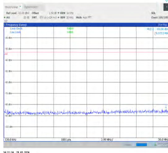
1-N70-15-15-L-1-DFT-PI2BPSK-Inner_1RB_Left-1@ 1-0.15-30-Ant1-29.37--83.58--33-PASS
