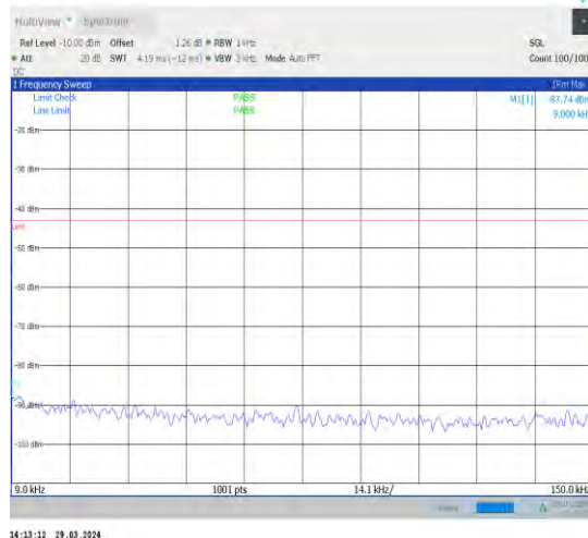
1-N70-15-15-M-1-DFT-PI2BPSK-Inner_1RB_Left-1@ 1-0.009-0.15-Ant1-0.01--87.74--43-PASS
