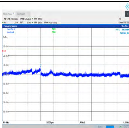
1-N70-15-15-L-1-DFT-PI2BPSK-Inner_1RB_Left-1@ 1-3000-18000-Ant1-7498.50--33.09--13-PASS
