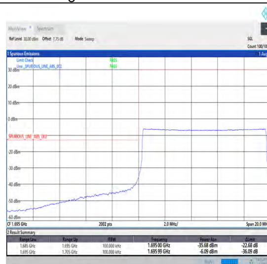
1-N70-15-10-L-6-CP-QPSK-Outer_Full-52@0-Ant1 1-1-seegraph-PASS-see graph
