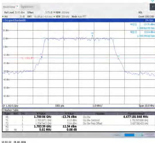
1-N70-15-5-M-5-DFT-256QAM-Outer_Full-25@0-Ant 1-4.477-5.020-≤5-PASS
