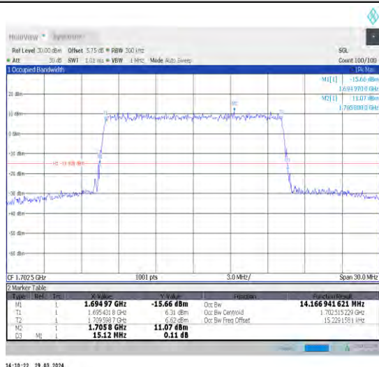
1-N70-15-15-M-9-CP-256QAM-Outer_Full-79@0-An t1-14.167-15.120≤15-PASS
