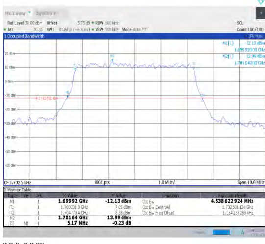
1-N70-15-5-M-7-CP-16QAM-Outer_Full-25@0-Ant1- 4.539-5.170-≤5-PASS
