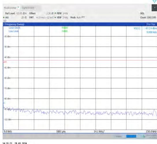
1-N70-15-15-H-1-DFT-PI2BPSK-Inner_1RB_Left-1 @1-0.009-0.15-Ant1-0.01--87.24--43-PASS
