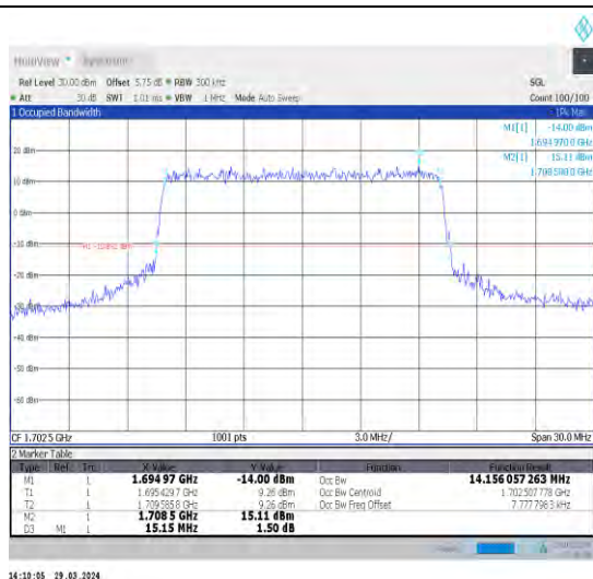
1-N70-15-15-M-7-CP-16QAM-Outer_Full-79@0-Ant 1-14.156-15.150≤15-PASS
