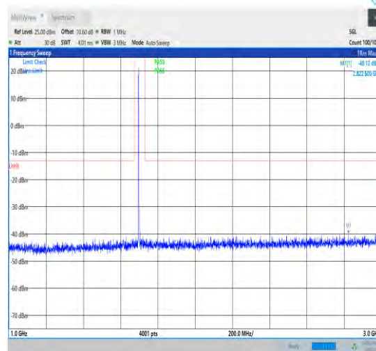
1-N70-15-15-L-1-DFT-PI2BPSK-Inner_1RB_Left-1@ 1-1000-3000-Ant1-2822.50--40.12--13-PASS
