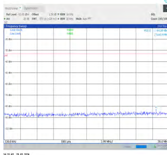
1-N70-15-15-H-1-DFT-PI2BPSK-Inner_1RB_Left-1@ 1-0.15-30-Ant1-27.64--84.39--33-PASS
