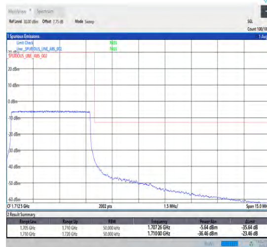
1-N70-15-5-H-6-CP-QPSK-Outer_Full-25@0-Ant1 -1-seegraph-PASS-see graph
