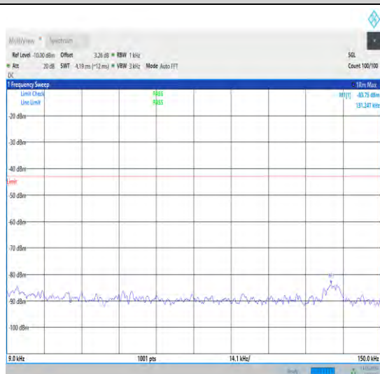
1-N70-15-15-H-1-DFT-PI2BPSK-Inner_1RB_Left-1@ 1-0.009-0.15-Ant1-0.13--83.75--43-PASS
