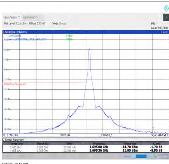
1-N70-15-10-L-1-DFT-PI2BPSK-Edge_1RB_Left-1@0-Ant1-1-seegraph-PASS-see graph
