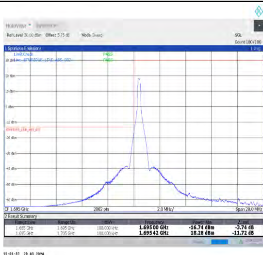
1-N70-15-10-L-4-CP-QPSK-Edge_1RB_Left-1@0-Ant1-1-seegraph-PASS-see graph
