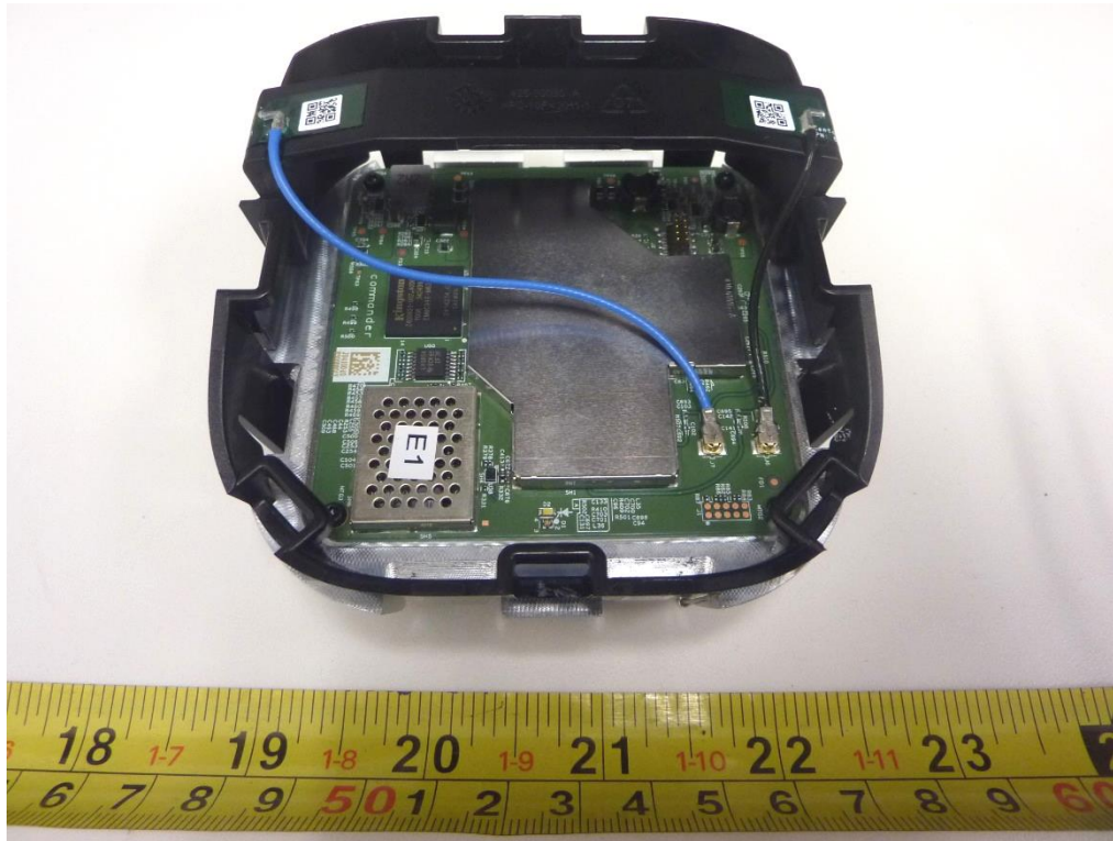
Figure 1 - Internal Photo of EUT- Top View
