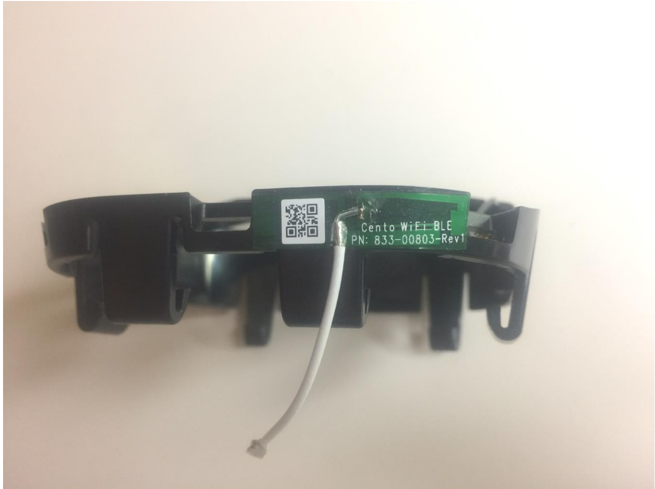
Figure 10 - Internal Photo of EUT- Antenna BLE View
