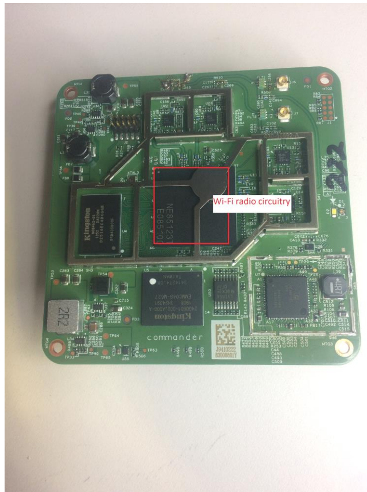
Figure 5 - Internal Photo of EUT- Main PCB No Shield Top View
