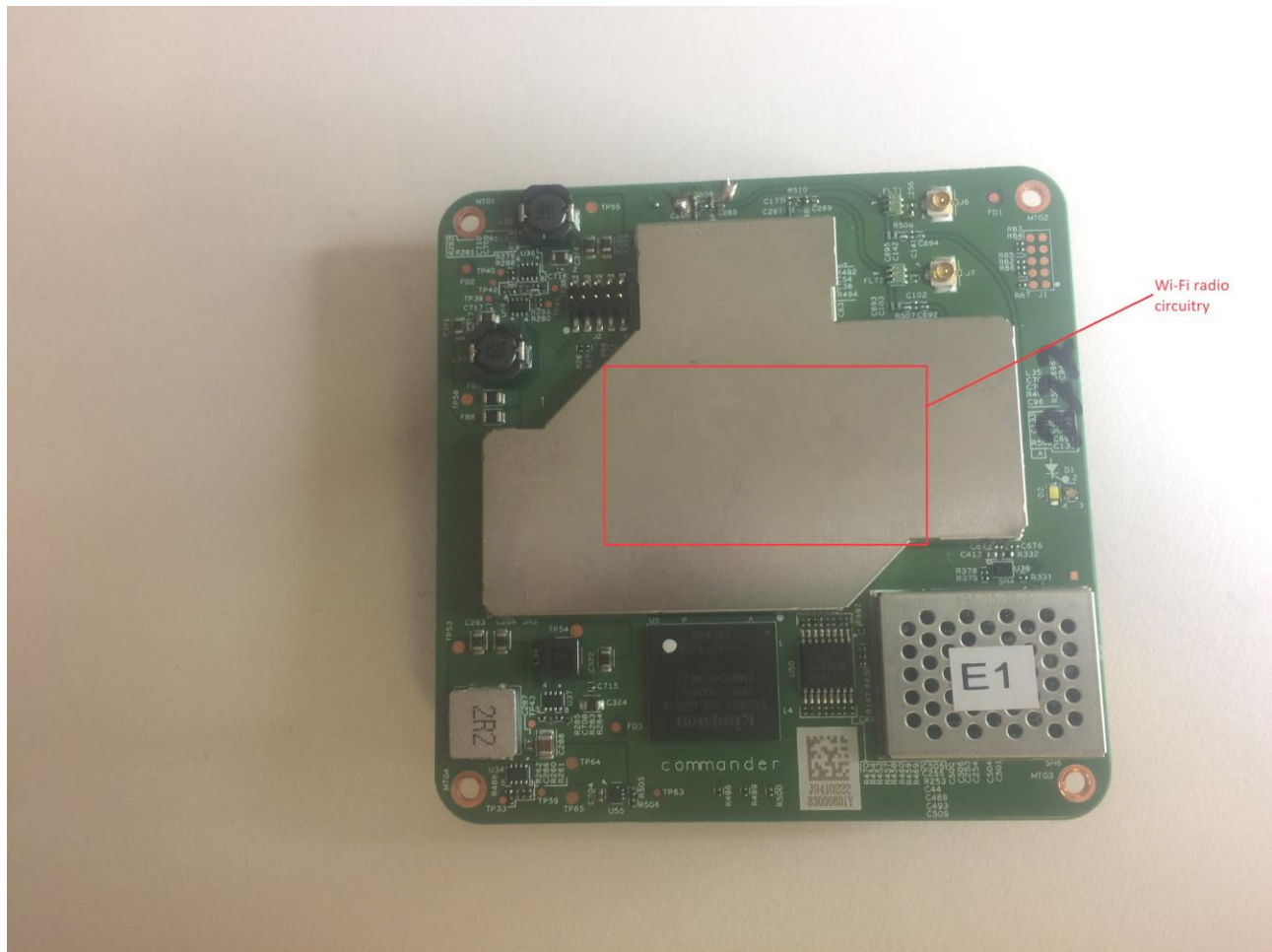
Figure 3 - Internal Photo of EUT- Main PCB with Shield Top View
