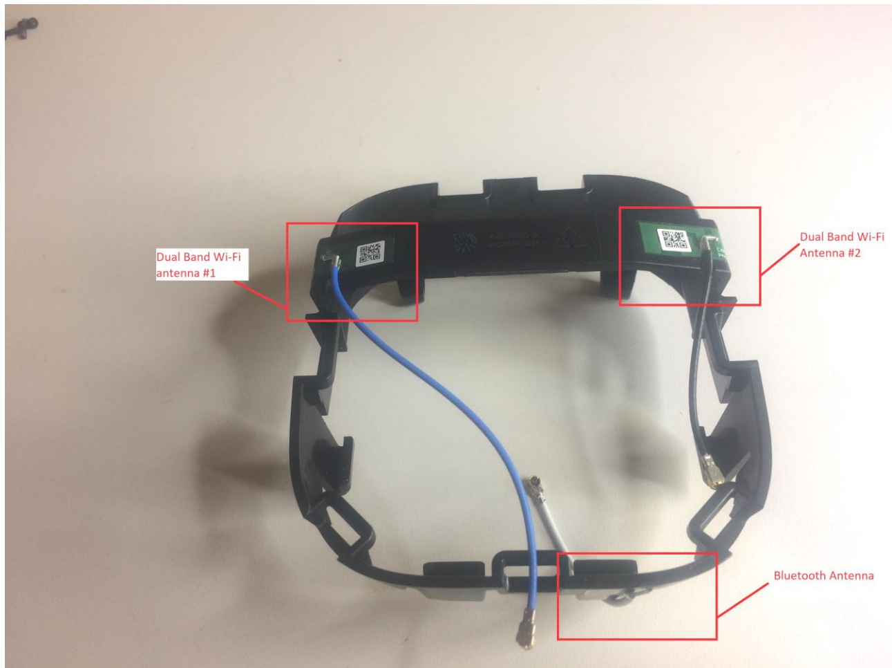
Figure 9 - Internal Photo of EUT- Antenna Carrier View
