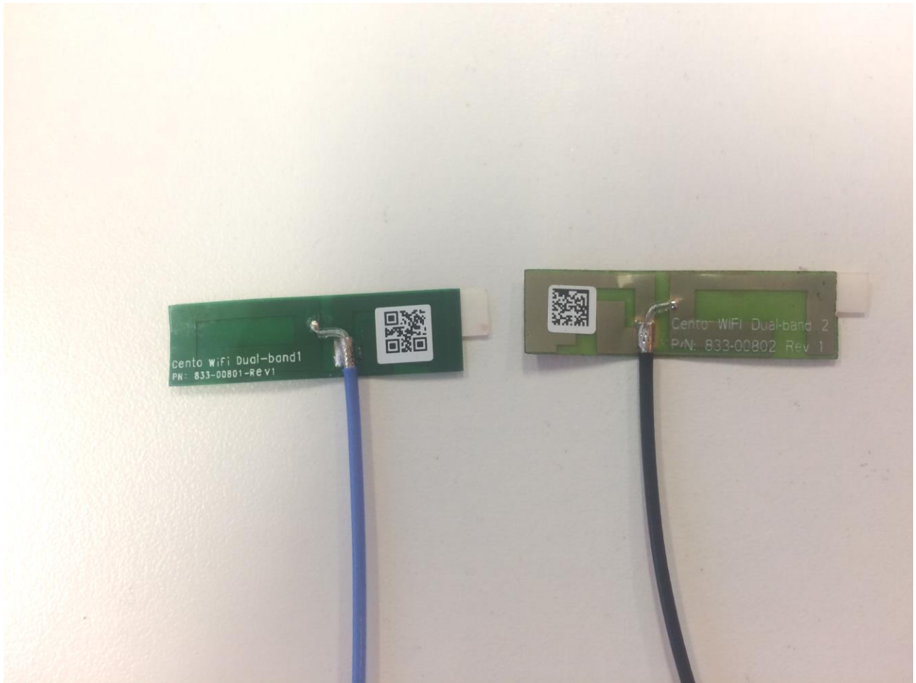
Figure 13 - Internal Photo of EUT- Antenna 1 and 2 WiFi View
