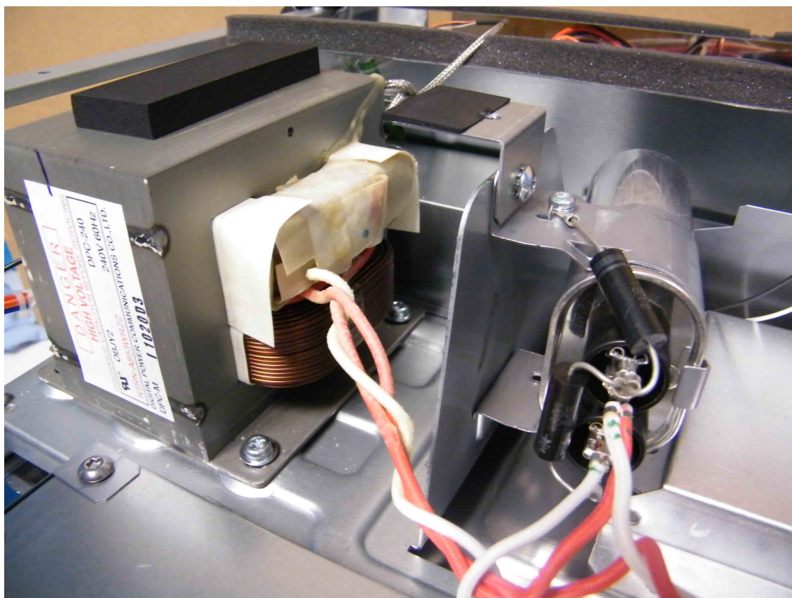
HV TRANSFORMER AND HV CAPACITOR
