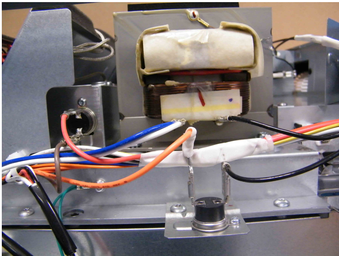
HV TRANSFORMER AND TWO PROTECTIVE THERMAL CUT-OUTS
