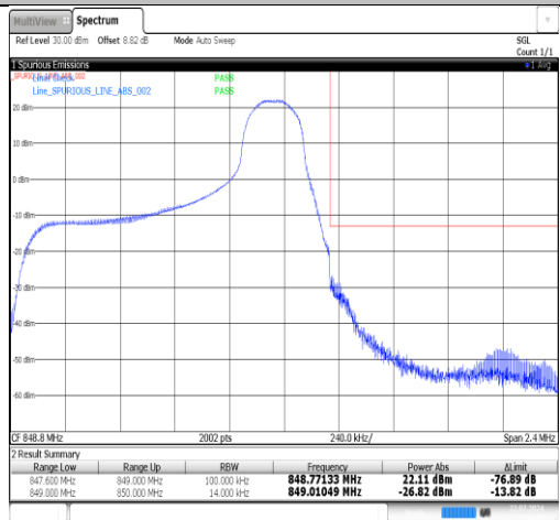
Band26(824-849)-1.4MHz-16QAM-27033-1RB#5-PASS
