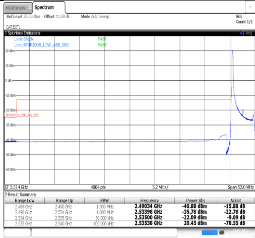
Band41(2535-2655)-5MHz-16QAM-40065-1RB#24-PASS
