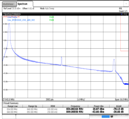
Band26(824-849)-15MHz-16QAM-26965-1RB#0-PASS
