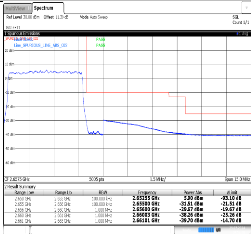
Band41(2535-2655)-5MHz-16QAM-41215-25RB#0-PASS
