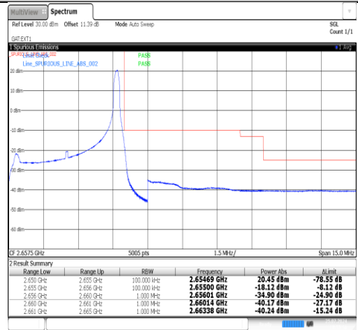
Band41(2535-2655)-5MHz-16QAM-41215-1RB#24-PASS
