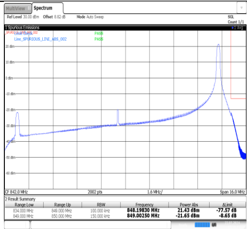
Band26(824-849)-15MHz-16QAM-26965-1RB#74-PASS
