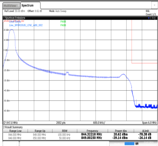
Band26(824-849)-5MHz-16QAM-27015-1RB#0-PASS
