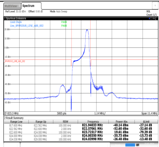
Band26(814-824)-1.4MHz-16QAM-26783-1RB#5-PASS
