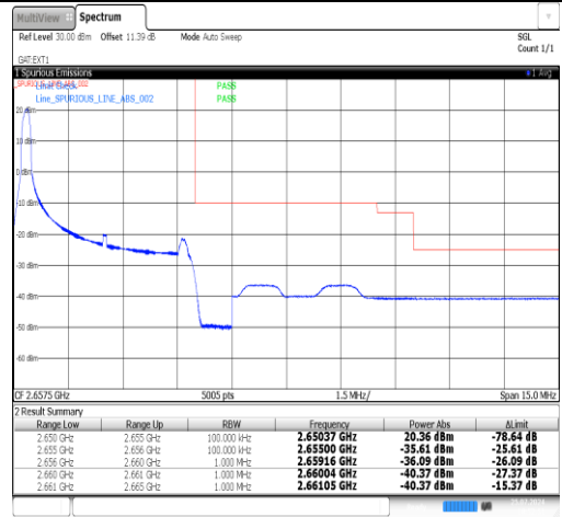
Band41(2535-2655)-5MHz-16QAM-41215-1RB#0-PASS
