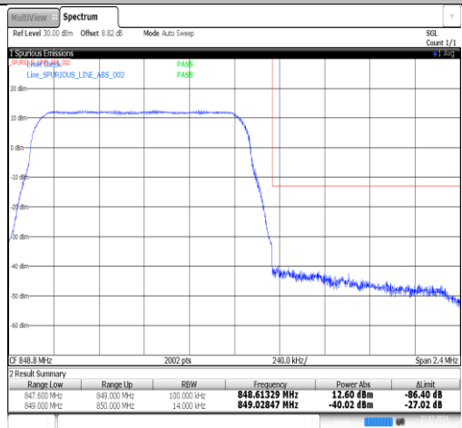
Band26(824-849)-1.4MHz-16QAM-27033-6RB#0-PASS
