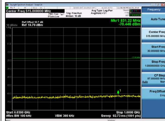
CUE-802.11n-40-5550M-chain1(30MHz-1GHz)
