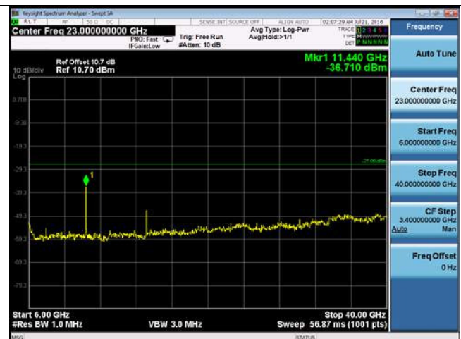
CUE-802.11n20-5720M -chain4(6GHz-40GHz)
