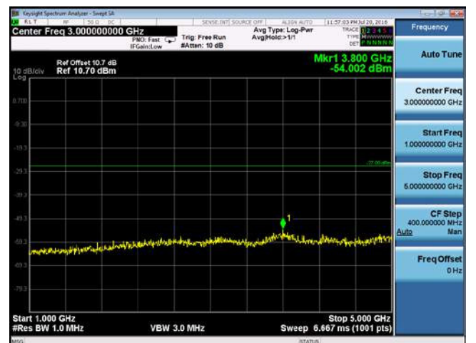
CUE-802.11n-40-5550M-chain1(1GHz-5GHz)
