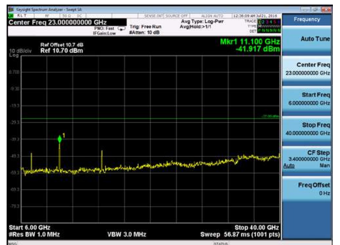
CUE-802.11n-40-5550M-chain2(6GHz-40GHz)
