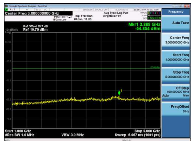
CUE-802.11n40-5710M -chain1(1GHz-5GHz)
