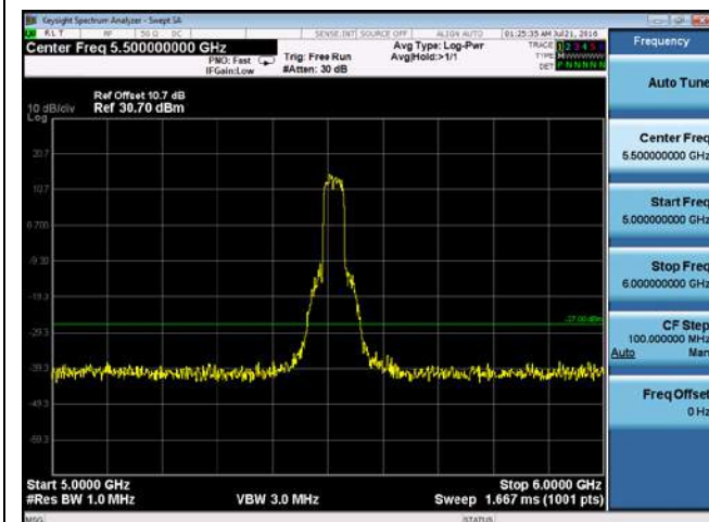
CUE-802.11n-40-5510M-chain3(5GHz-6GHz)
