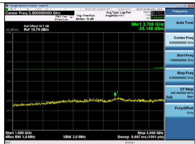
CUE-802.11n20-5720M -chain4(1GHz-5GHz)
