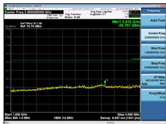
CUE-802.11n20-5720M -chain3(1GHz-5GHz)
