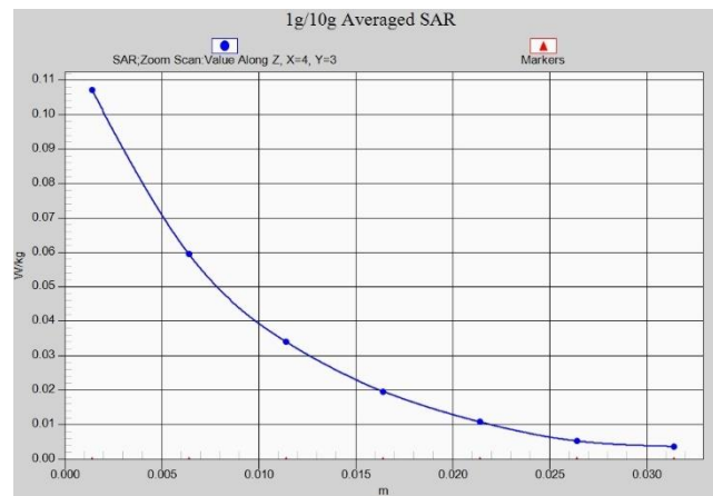
Fig. 1-28 Z-Scan at power reference point (WLAN2.4G)
