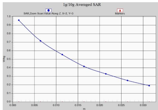
Fig. 1-21 Z-Scan at power reference point (LTEB5)
