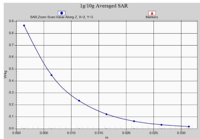
Fig. 1-24 Z-Scan at power reference point (LTEB7)
