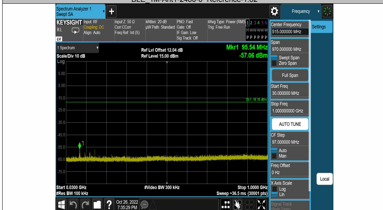
BLE_1M-Ant1-2480-30~1000-1.82
