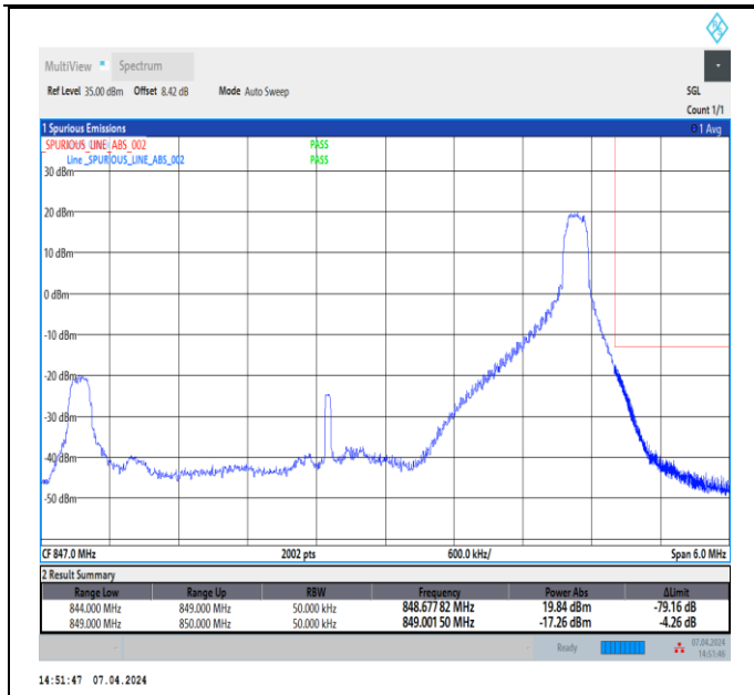
Band5_5MHz_QPSK_20625_1RB#24
