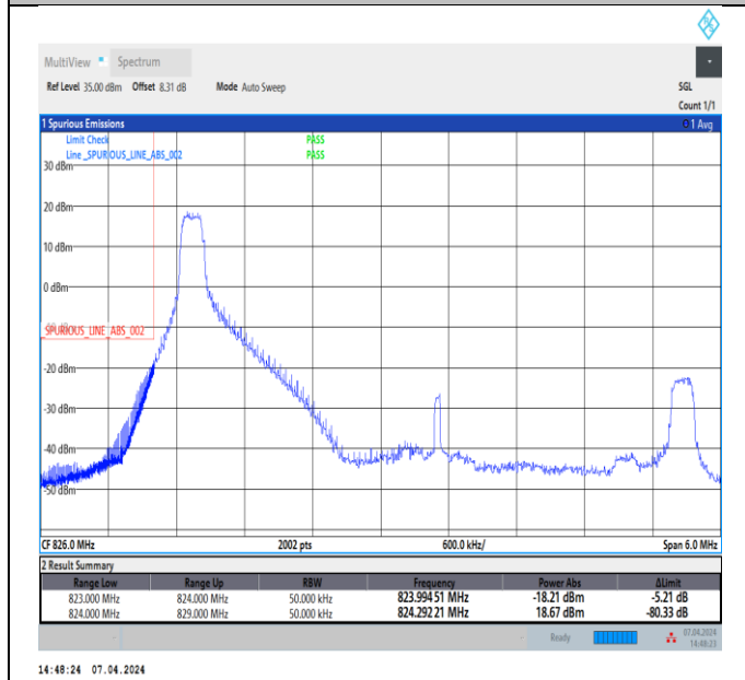
Band5_5MHz_16QAM_20425_1RB#0
