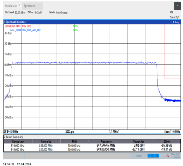
Band5_10MHz_64QAM_20600_50RB#0
