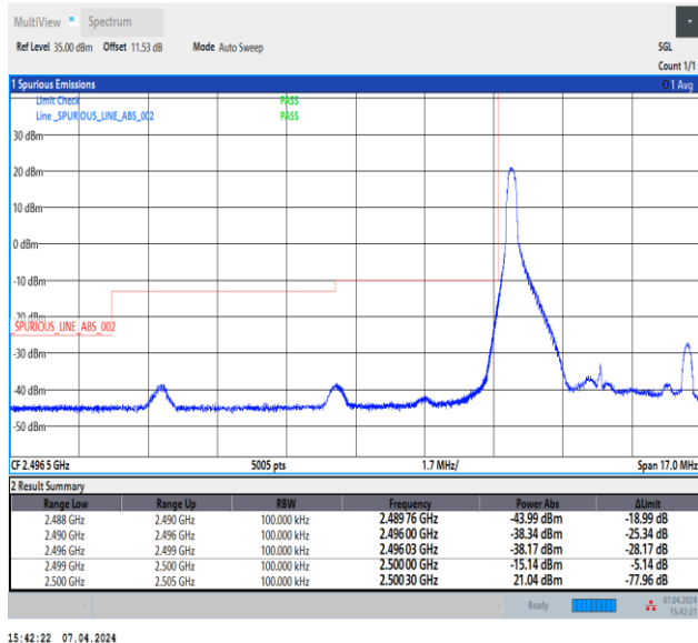
Band7_5MHz_QPSK_20775_1RB#0
