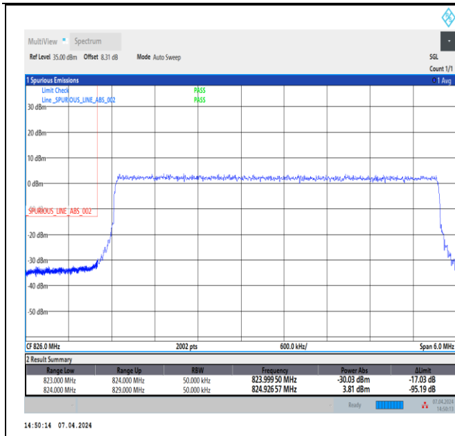
Band5_5MHz_16QAM_20425_25RB#0
