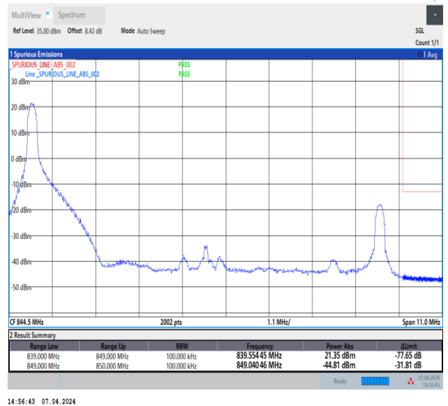
Band5_10MHz_QPSK_20600_1RB#0
