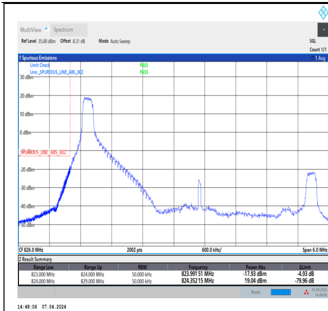
Band5_5MHz_QPSK_20425_1RB#0
