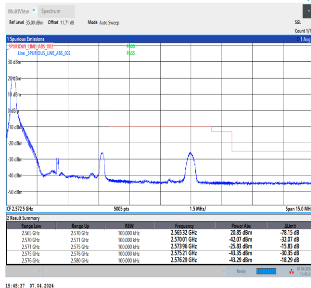
Band7_5MHz_QPSK_21425_1RB#0
