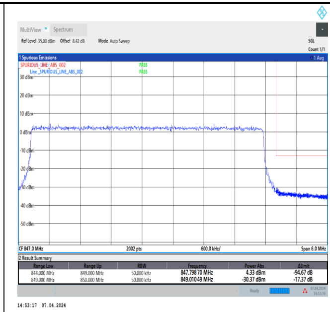
Band5_5MHz_64QAM_20625_25RB#0
