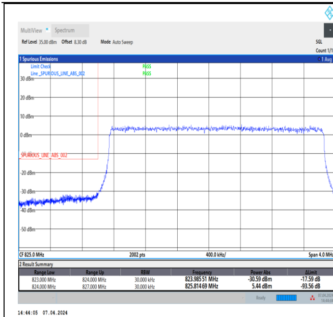
Band5_3MHz_QPSK_20415_15RB#0
