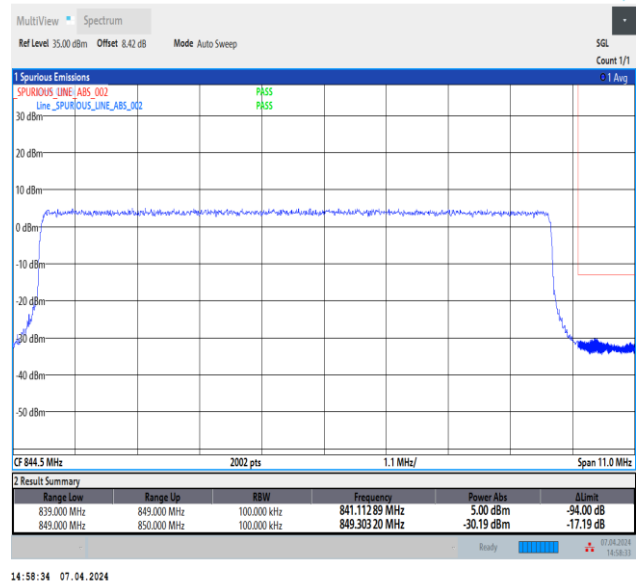
Band5_10MHz_QPSK_20600_50RB#0
