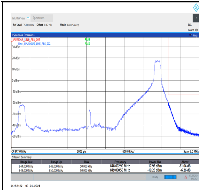
Band5_5MHz_64QAM_20625_1RB#24
