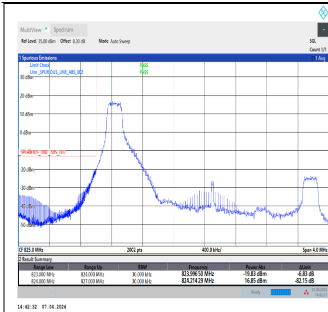
Band5_3MHz_16QAM_20415_1RB#0
