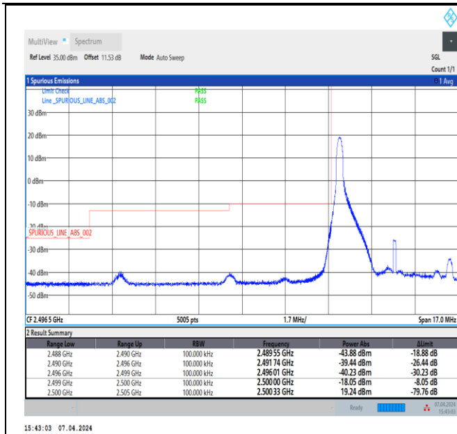
Band7_5MHz_64QAM_20775_1RB#0
