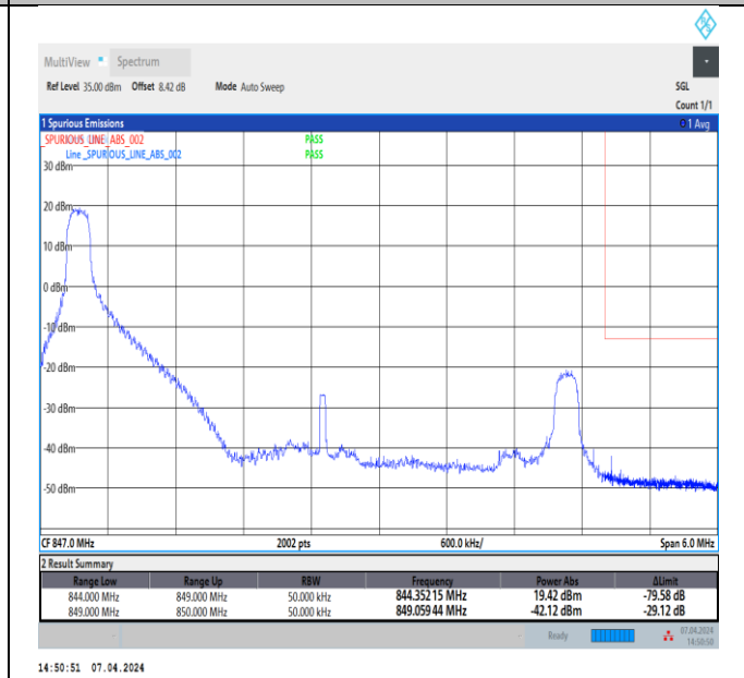
Band5_5MHz_QPSK_20625_1RB#0
