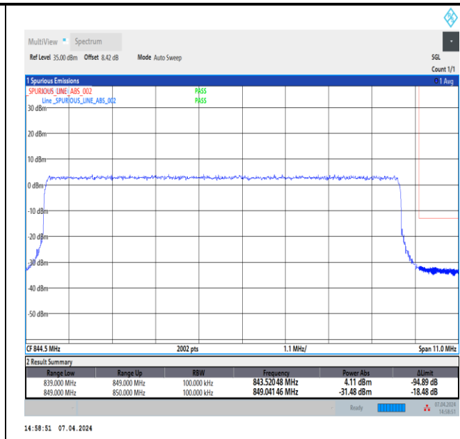
Band5_10MHz_16QAM_20600_50RB#0
