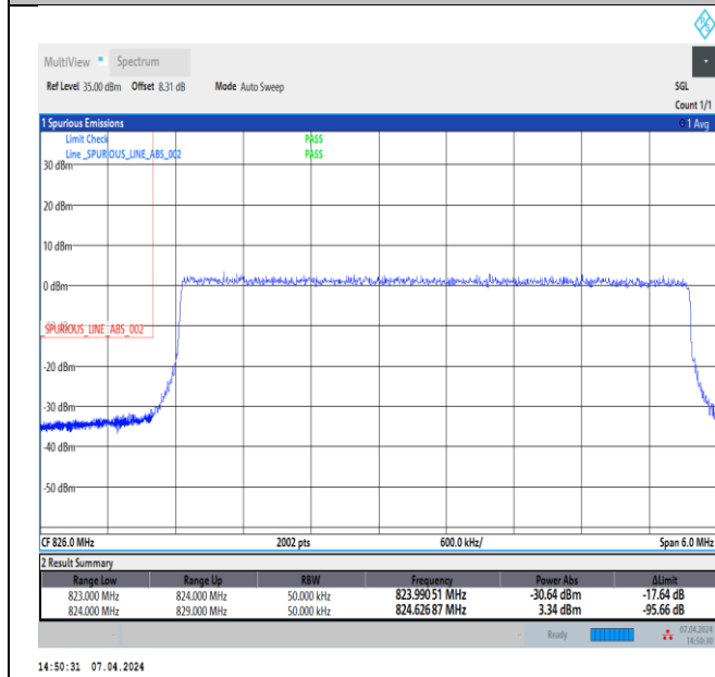
Band5_5MHz_64QAM_20425_25RB#0
