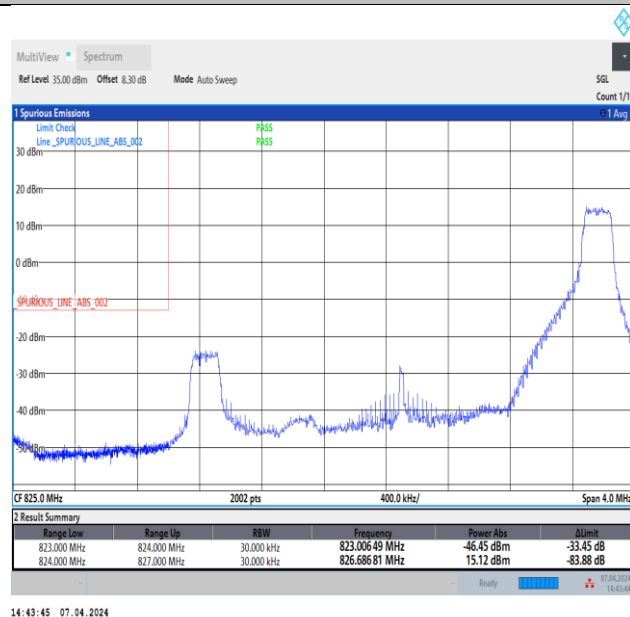
Band5_3MHz_64QAM_20415_1RB#14
