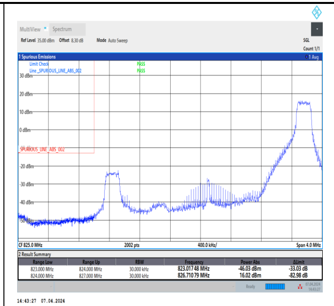
Band5_3MHz_16QAM_20415_1RB#14
