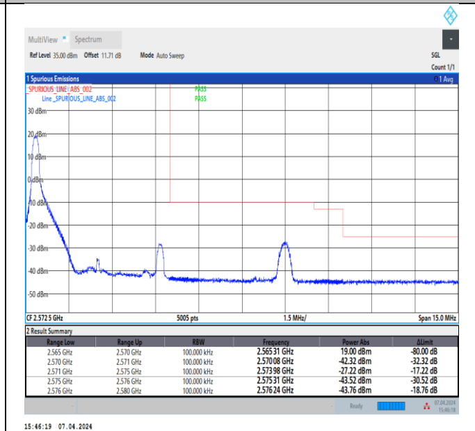
Band7_5MHz_64QAM_21425_1RB#0
