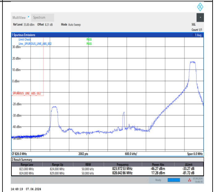
Band5_5MHz_16QAM_20425_1RB#24
