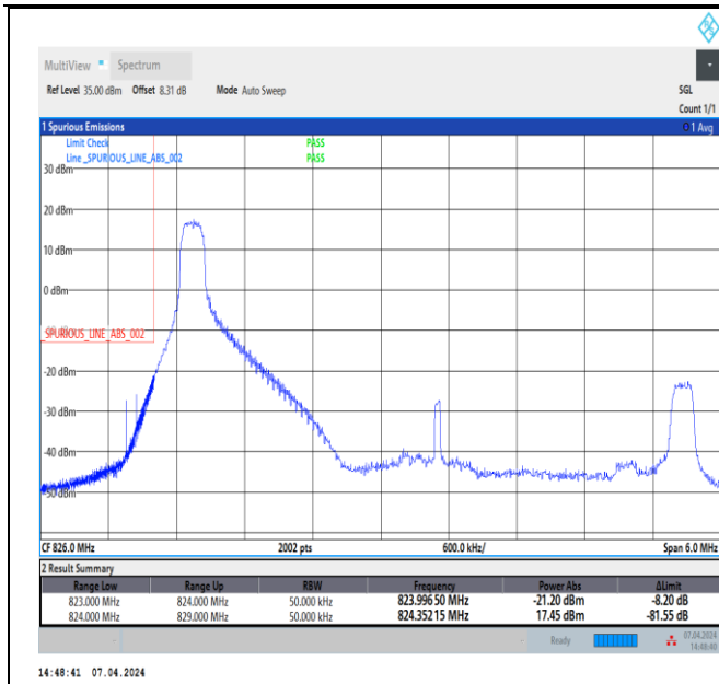
Band5_5MHz_64QAM_20425_1RB#0
