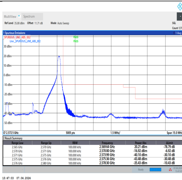
Band7_5MHz_16QAM_21425_1RB#24
