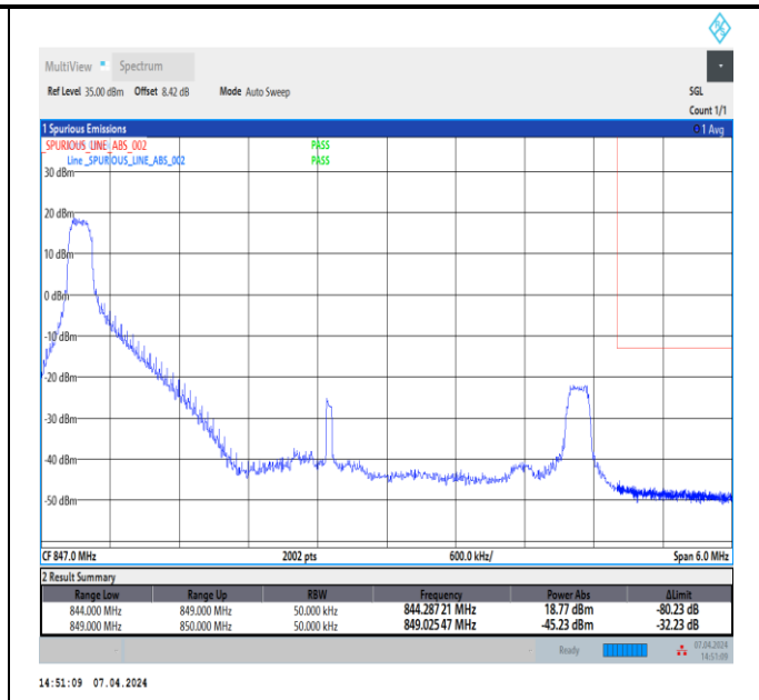
Band5_5MHz_16QAM_20625_1RB#0
