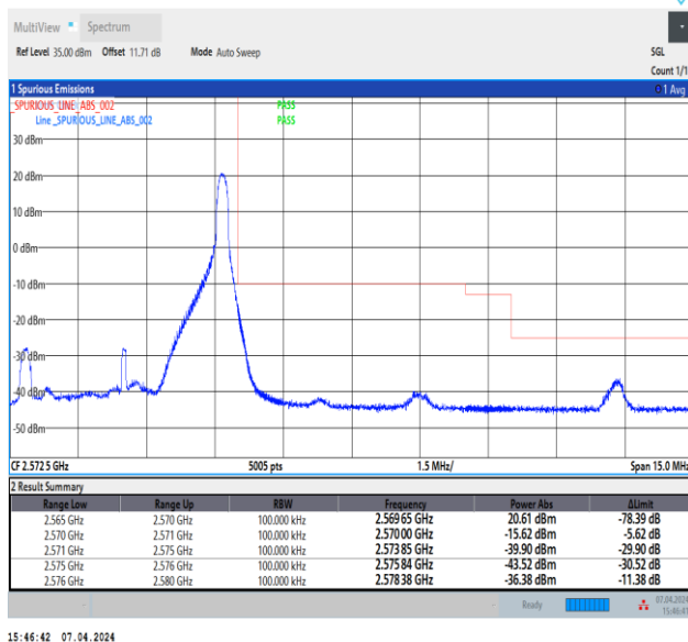
Band7_5MHz_QPSK_21425_1RB#24
