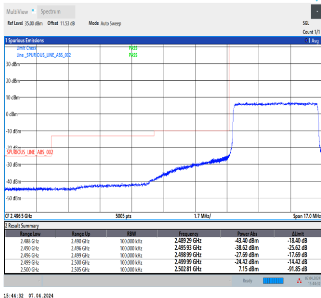
Band7_5MHz_QPSK_20775_25RB#0
