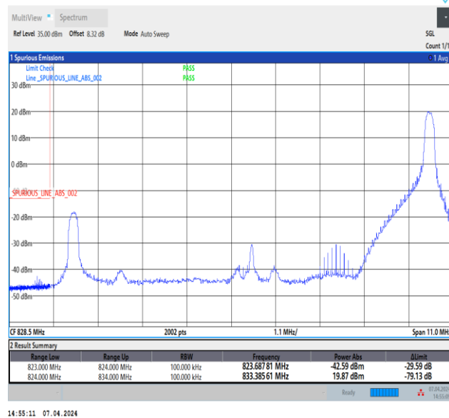
Band5_10MHz_16QAM_20450_1RB#49
