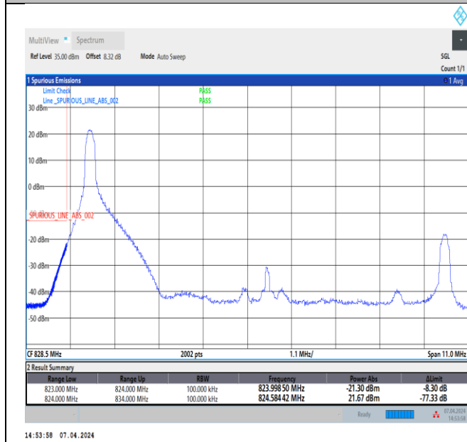
Band5_10MHz_QPSK_20450_1RB#0
