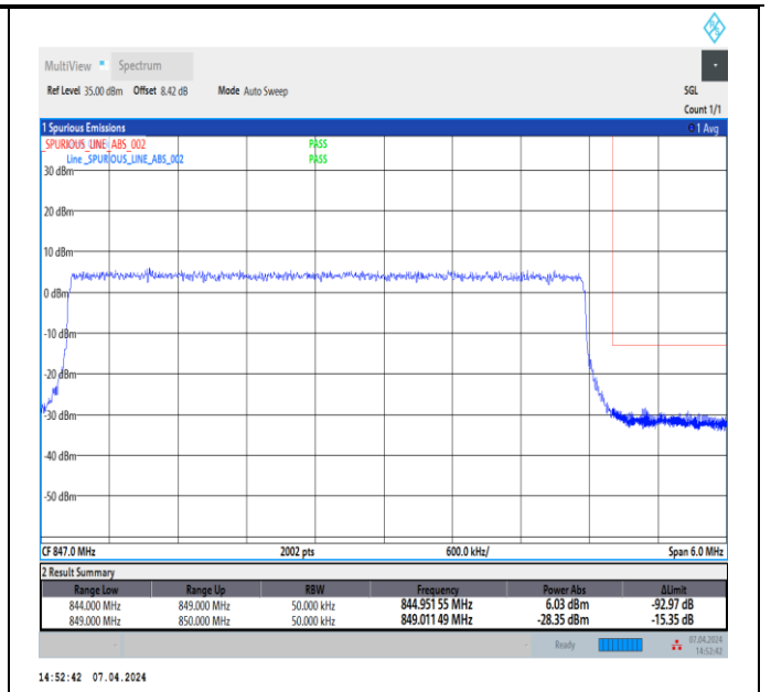
Band5_5MHz_QPSK_20625_25RB#0
