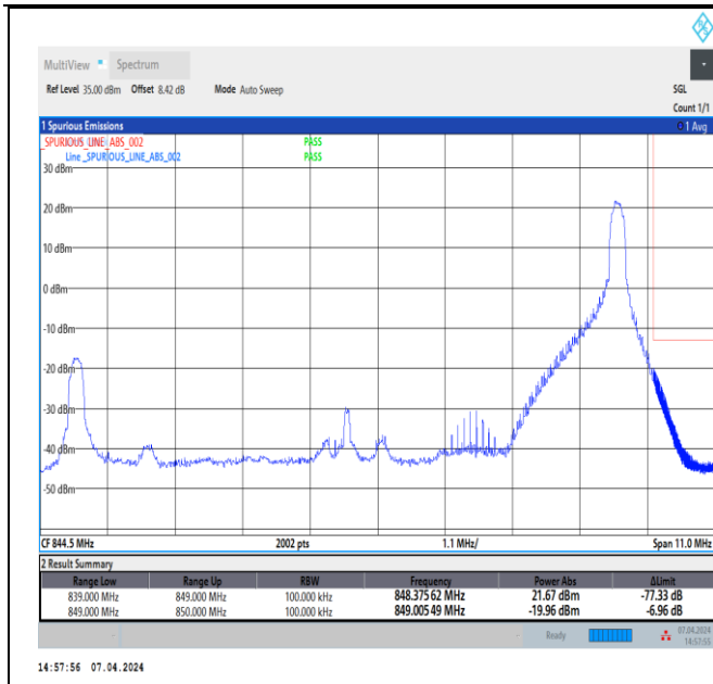
Band5_10MHz_16QAM_20600_1RB#49
