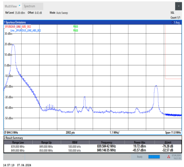
Band5_10MHz_64QAM_20600_1RB#0
