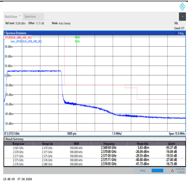
Band7_5MHz_16QAM_21425_25RB#0
