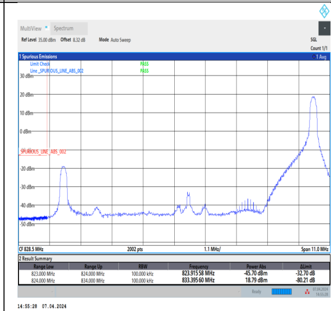
Band5_10MHz_64QAM_20450_1RB#49
