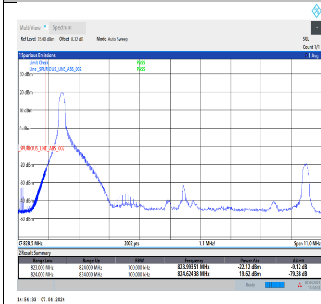
Band5_10MHz_64QAM_20450_1RB#0
