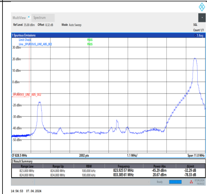
Band5_10MHz_QPSK_20450_1RB#49
