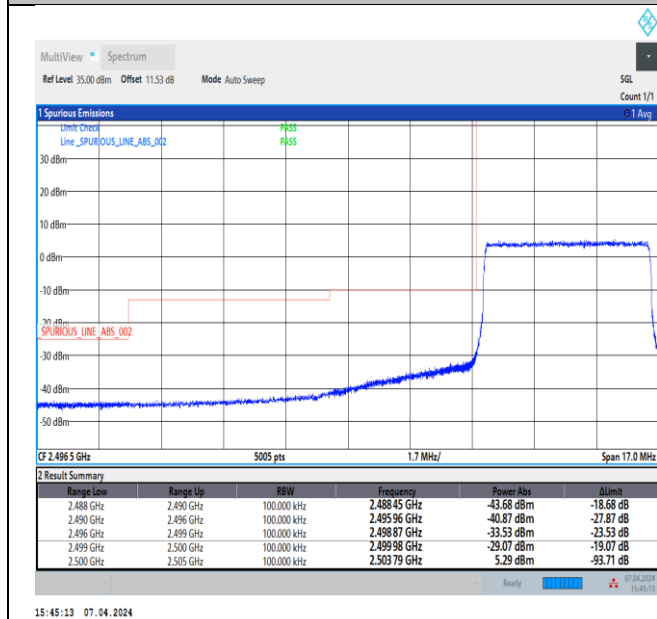
Band7_5MHz_64QAM_20775_25RB#0
