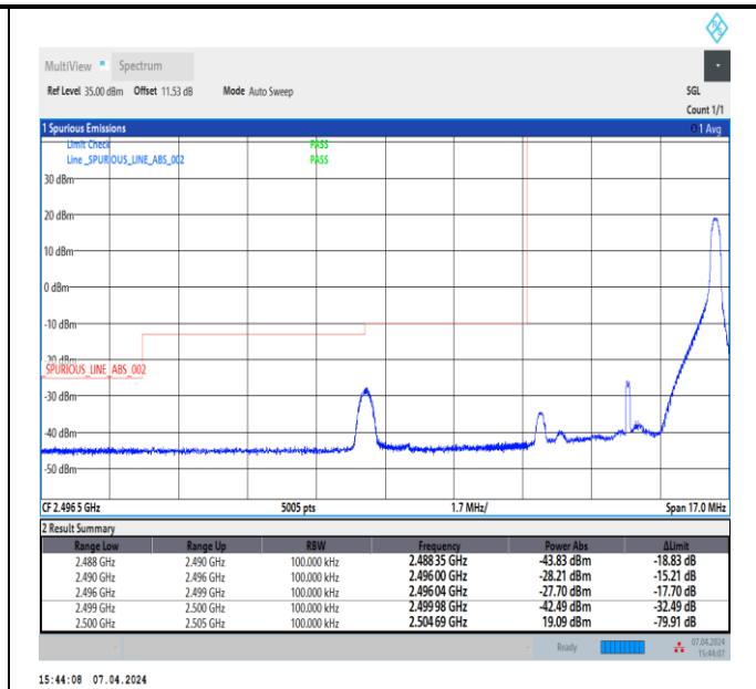
Band7_5MHz_64QAM_20775_1RB#24
