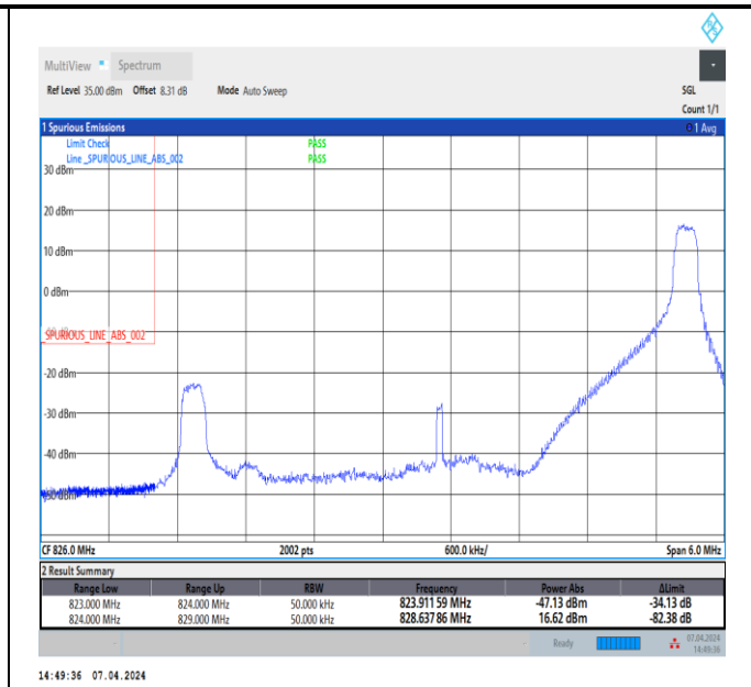
Band5_5MHz_64QAM_20425_1RB#24
