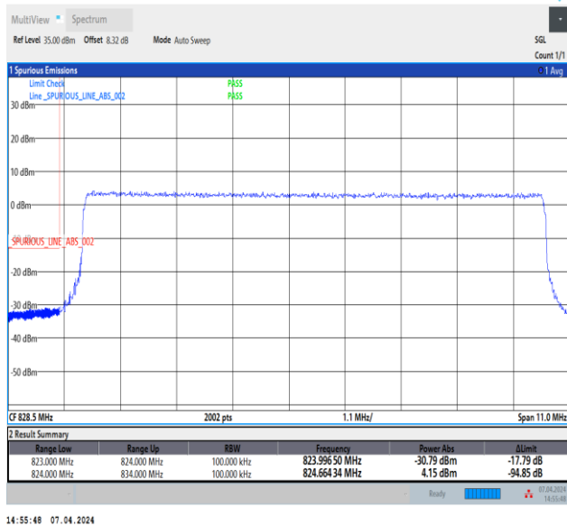
Band5_10MHz_QPSK_20450_50RB#0
