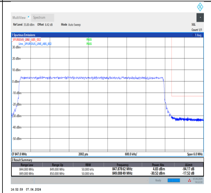
Band5_5MHz_16QAM_20625_25RB#0
