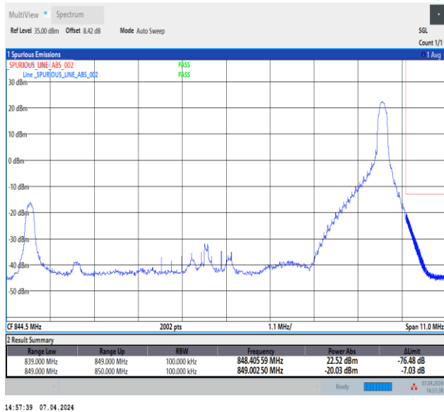
Band5_10MHz_QPSK_20600_1RB#49
