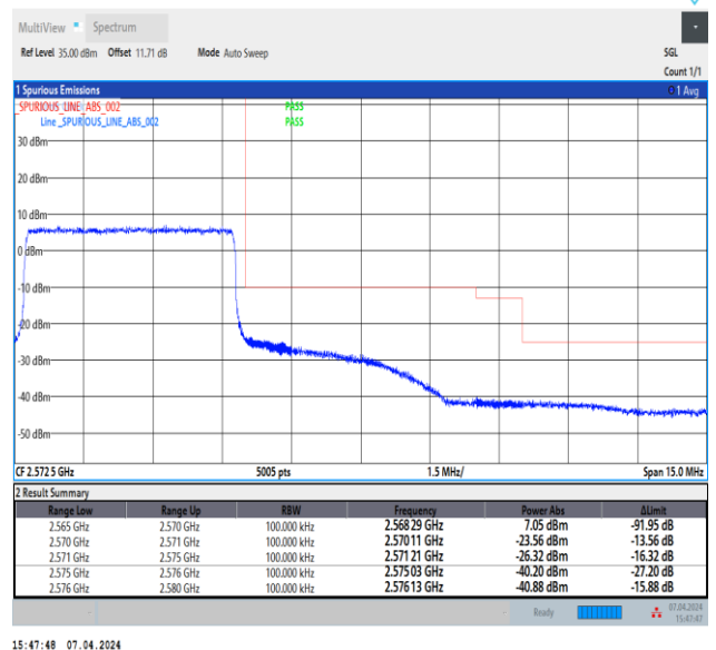
Band7_5MHz_QPSK_21425_25RB#0
