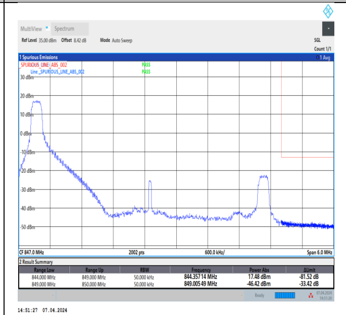
Band5_5MHz_64QAM_20625_1RB#0
