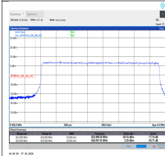
Band5_5MHz_QPSK_20425_25RB#0
