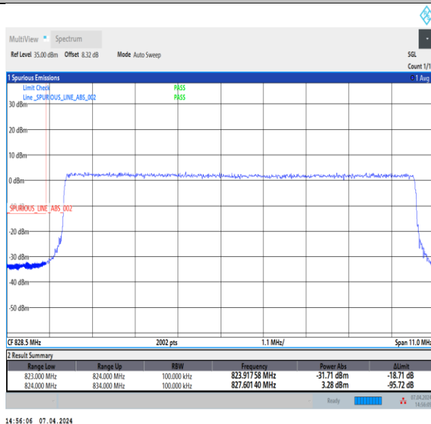
Band5_10MHz_16QAM_20450_50RB#0
