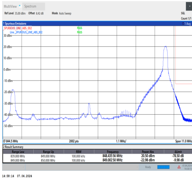
Band5_10MHz_64QAM_20600_1RB#49
