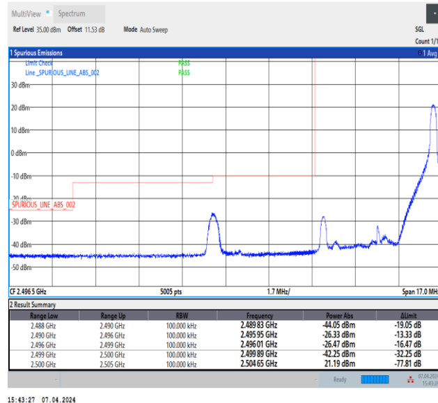
Band7_5MHz_QPSK_20775_1RB#24
