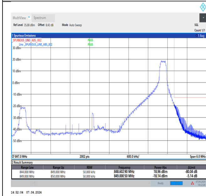
Band5_5MHz_16QAM_20625_1RB#24
