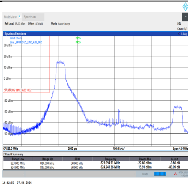
Band5_3MHz_64QAM_20415_1RB#0
