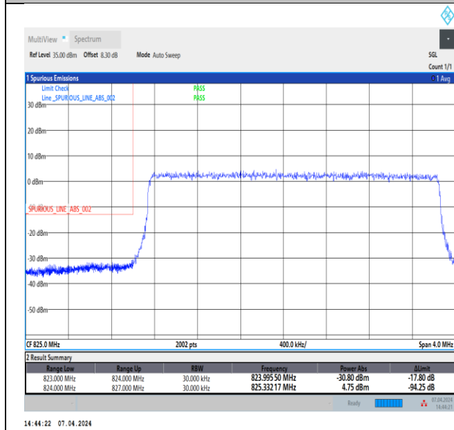
Band5_3MHz_16QAM_20415_15RB#0
