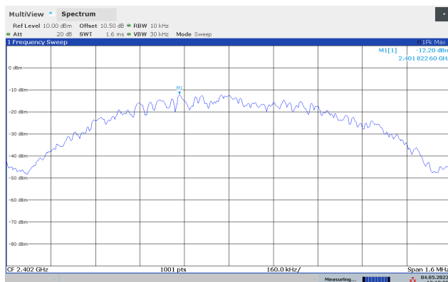
PSD, 2402 MHz, 1Mbit
