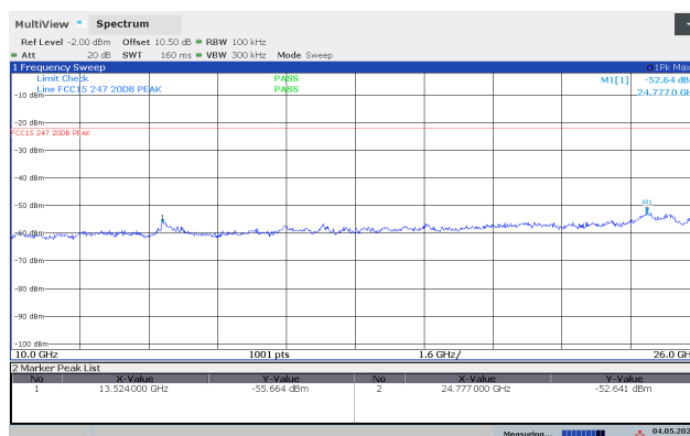
Conducted Emissions 10-26 GHz, 2440 MHz, 2Mb
