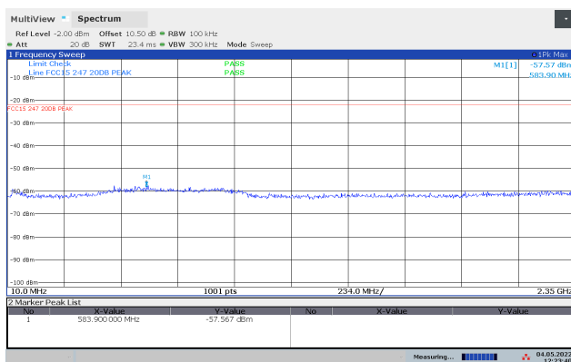
Conducted Emissions 10-2350 MHz, 2440 MHz, 2Mb
