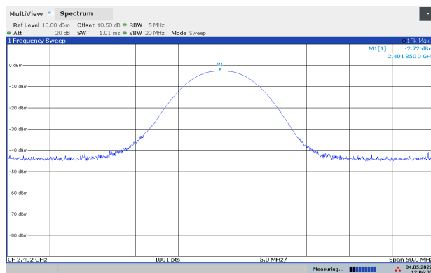
Peak Power, 2402 MHz, 2Mbit
