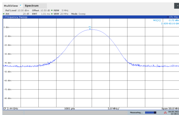
Peak Power, 2440 MHz, 2Mbit
