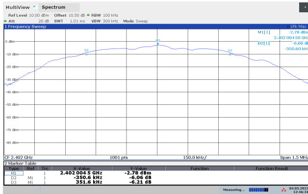
DTS BW, 2402 MHz, GFSK 1Mb
