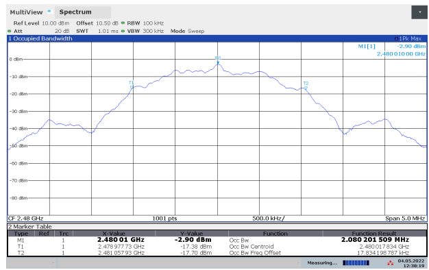
99% Occupied BW, 2480 MHz, 2Mbit
