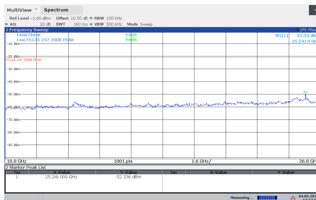
Conducted Emissions 10-26 GHz, 2402 MHz, 2Mb
