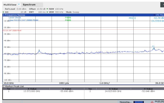
Conducted Emissions 10-26 GHz, 2480 MHz, 2Mb
