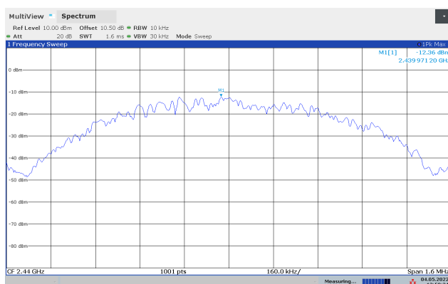
PSD, 2440 MHz, 1Mbit
