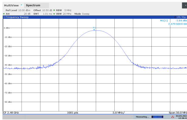
Peak Power, 2480 MHz, 2Mbit
