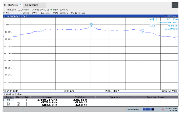
DTS BW, 2440 MHz, GFSK 2Mb
