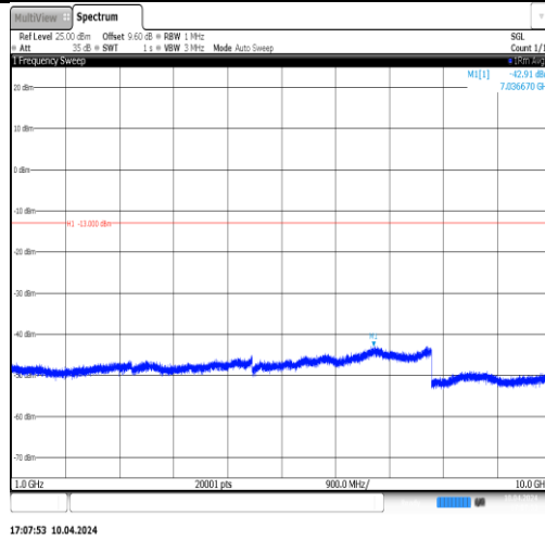
Band5-4182-2-1000~10000MHz-PASS
