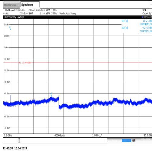
Band2-9400-2-1000~20000MHz-PASS
