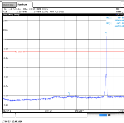
Band5-4233-2-30~1000MHz-PASS
