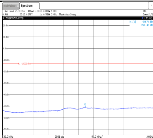
Band4-1513-1-30~1000MHz-PASS
