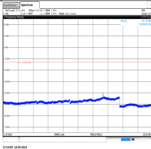
Band5-4182-4-1000~10000MHz-PASS
