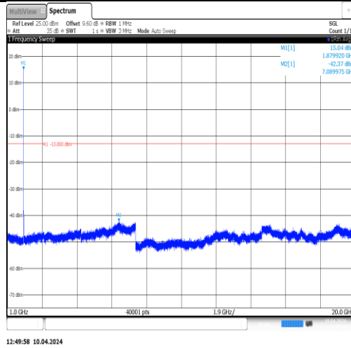
Band2-9400-5-1000~20000MHz-PASS
