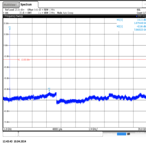
Band2-9400-3-1000~20000MHz-PASS
