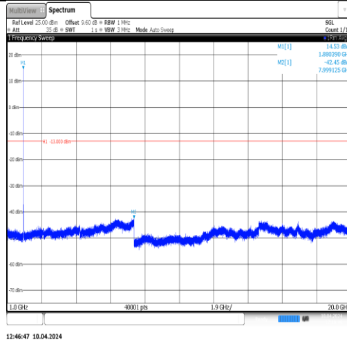
Band2-9400-4-1000~20000MHz-PASS
