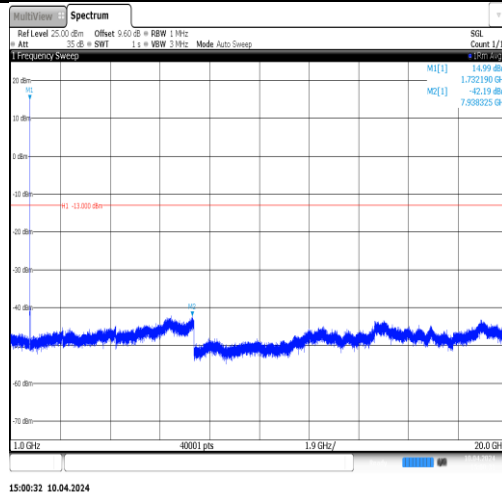
Band4-1413-2-1000~20000MHz-PASS
