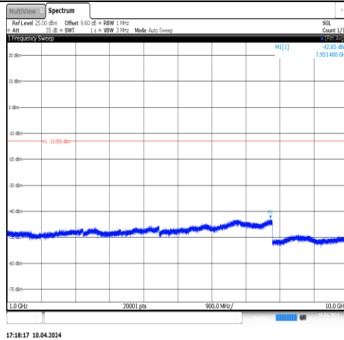
Band5-4233-5-1000~10000MHz-PASS
