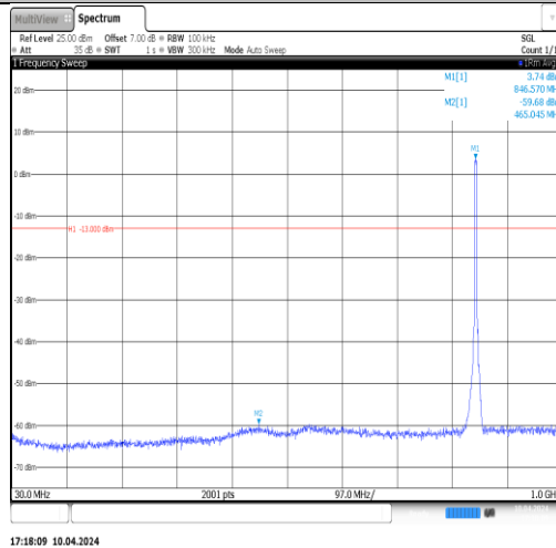
Band5-4233-5-30~1000MHz-PASS
