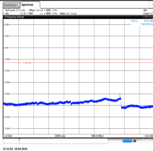
Band5-4182-3-1000~10000MHz-PASS
