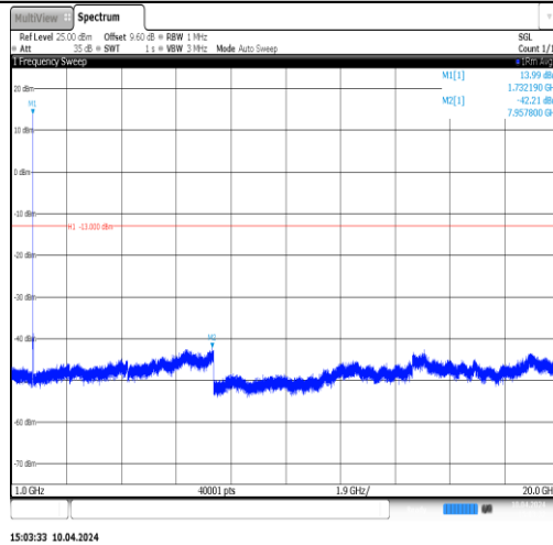
Band4-1413-3-1000~20000MHz-PASS
