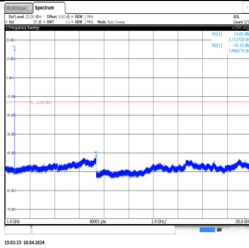
Band4-1312-3-1000~20000MHz-PASS
