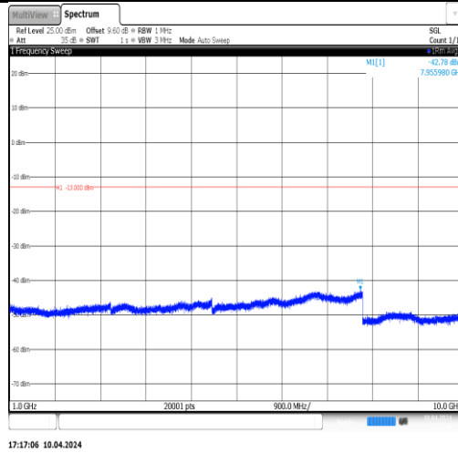
Band5-4182-5-1000~10000MHz-PASS
