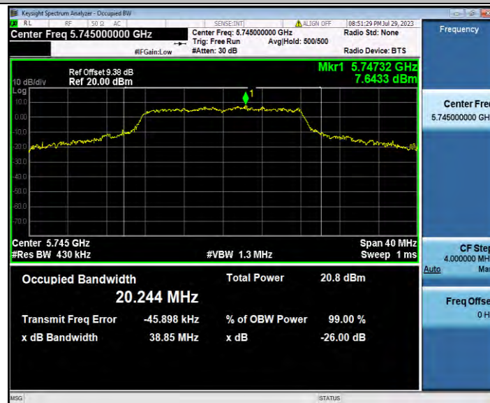
11N20SISO_Ant0_5745
