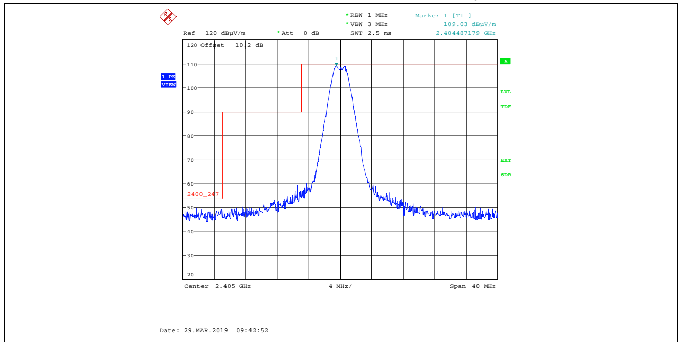
Plot 5.2.4.2.2. Band-Edge Radiated Emissions, Lower Band-edge, Peak Detector Rx Antenna in Horizontal Polarization, QPSK Modulation, Power Setting 9, Ch 11, 2405 MHz
