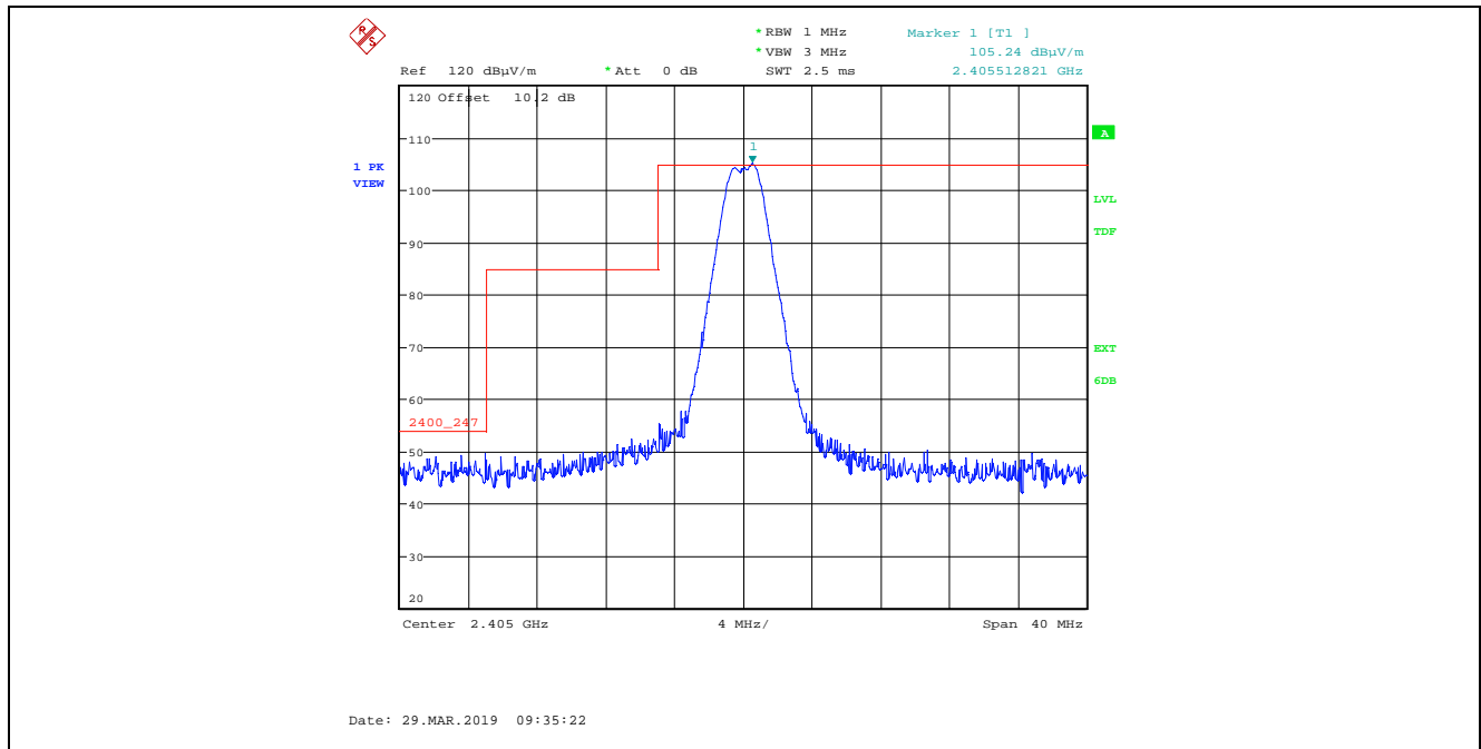
Plot 5.2.4.2.1. Band-Edge Radiated Emissions, Lower Band-edge, Peak Detector Rx Antenna in Vertical Polarization, QPSK Modulation, Power Setting 9, Ch 11, 2405 MHz
