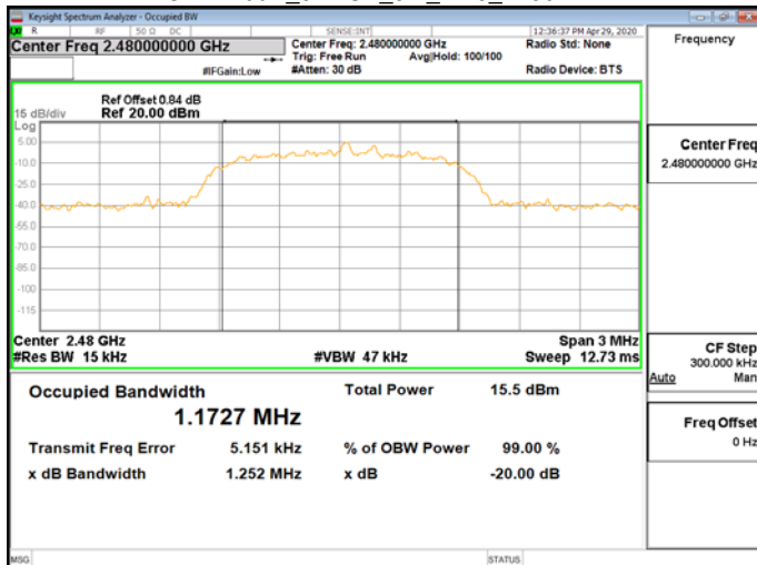
OBW 20dB_8DPSK_3M_DH5_2480MHz
