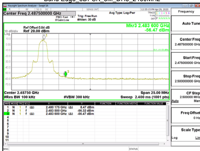
Band Edge_8DPSK_3M_DH5_2480MHz
